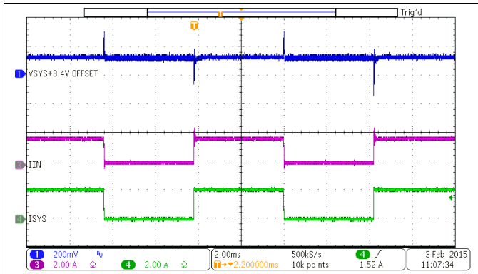
VBUS = 5 V I IN = 3 A Charge Disable
