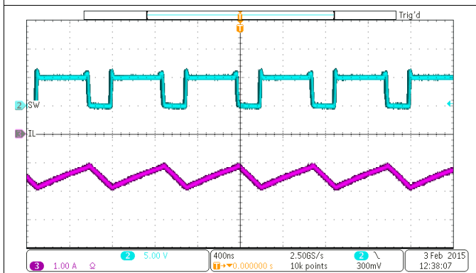
VBAT = 3.8 V I LOAD = 1 A
