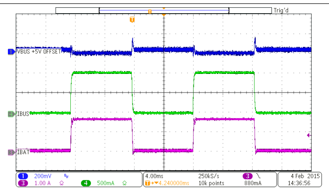
VBAT = 3.8 V I LOAD = 0 A - 1 A
