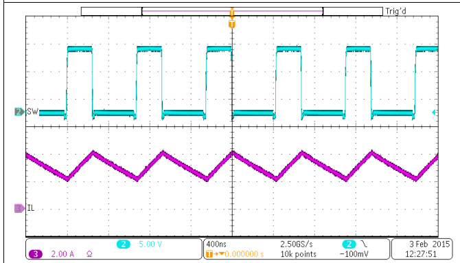
VBUS = 12 V VBAT = 3.8 V ICHG = 3 A
