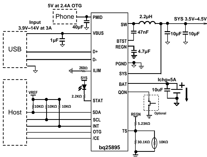
图 47. bq25895 with D+/D- Interface and 2.4 A Boost Mode Output
