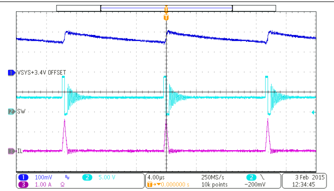
VBUS = 9V No Battery I SYS = 10 mA, Charge Disable
