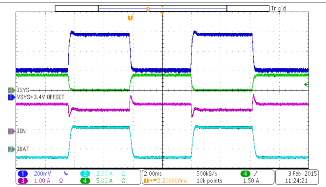
VBUS = 9 V I IN = 1.5 A VBAT = 3.8 V I CHG = 2 A I SYS = 0 A - 4 A
