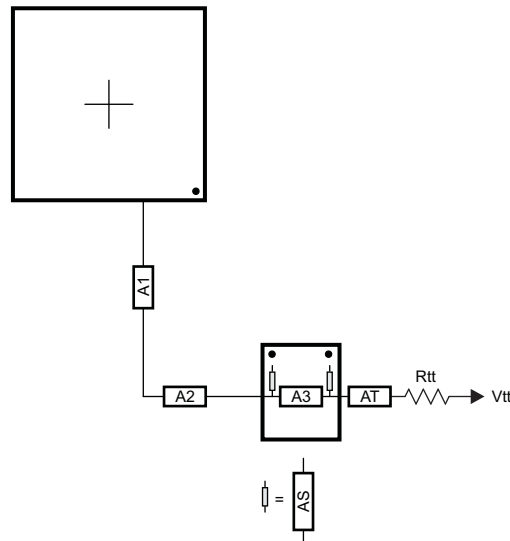
图 7-57. ADDR_CTRL Routing for Two Mirrored DDR3 Devices
