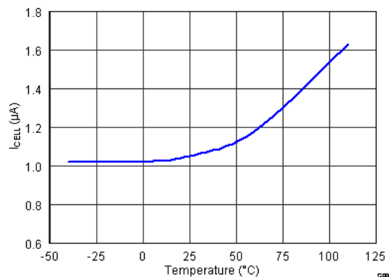
Figure 7-4. I_{CELL} vs. Temperature at V_{CELL} = 9.2\text{ V}
