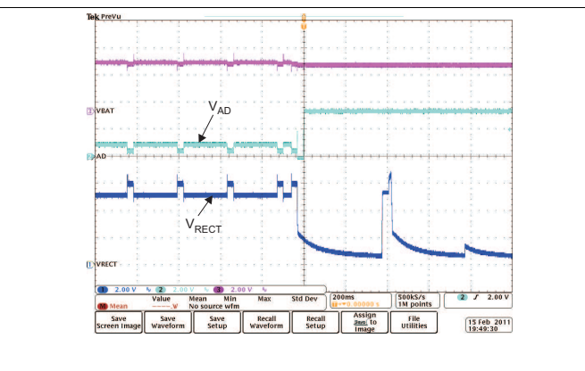
Figure 16. On-the-Go Enabled ( V_{OTG} = 3.5\text{ V} ) (3)
