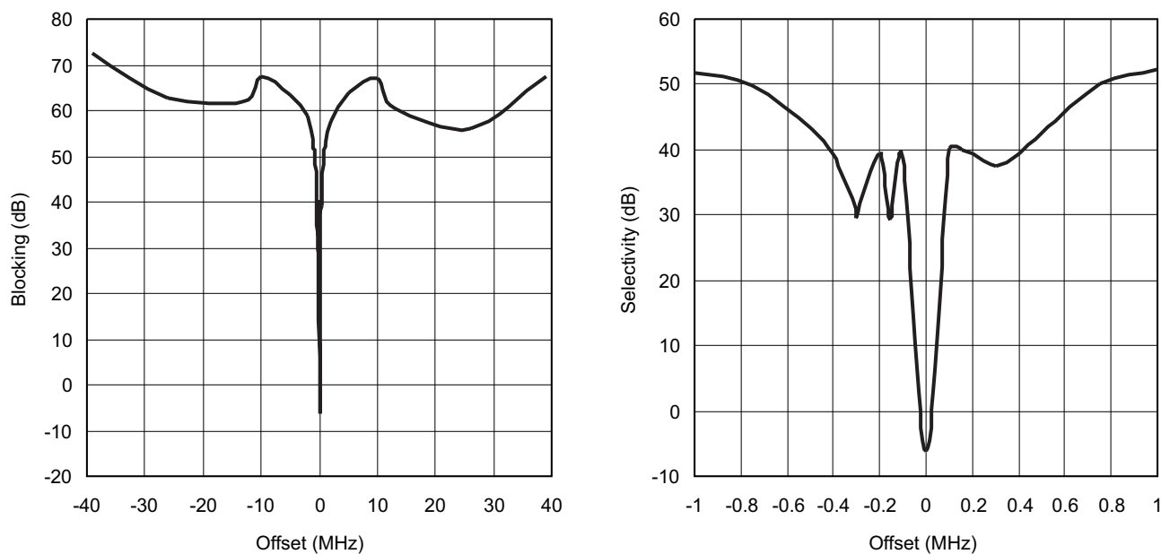
Figure 5-21. Typical Selectivity at 1.2-kBaud Data Rate
