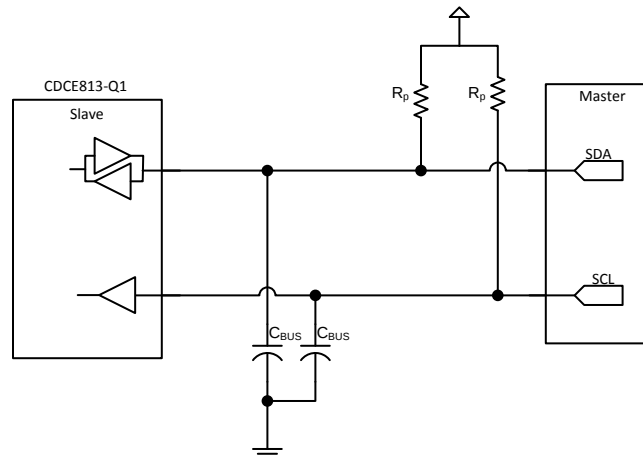
Figure 7. I2C Hardware Interface
