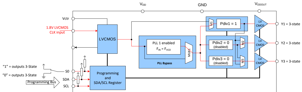
Figure 5. CDCE813-Q1 Default Configuration
