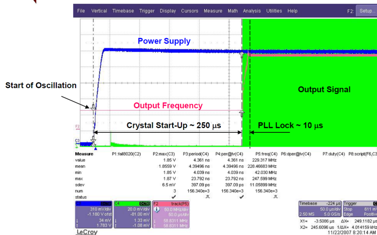
Figure 17. Crystal Oscillator Start-Up vs PLL Lock Time
