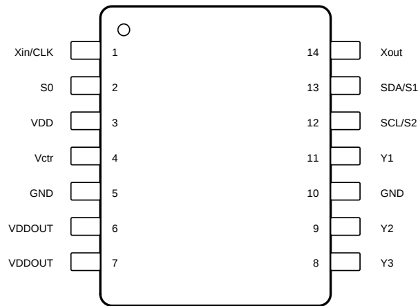
PW Package 14-Pin TSSOP Top View
