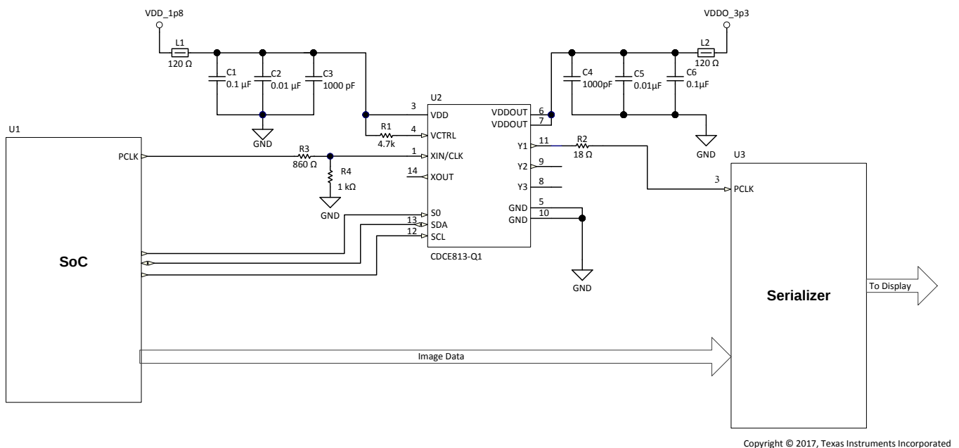
Figure 14. PCLK Jitter Cleaner Reference Design
