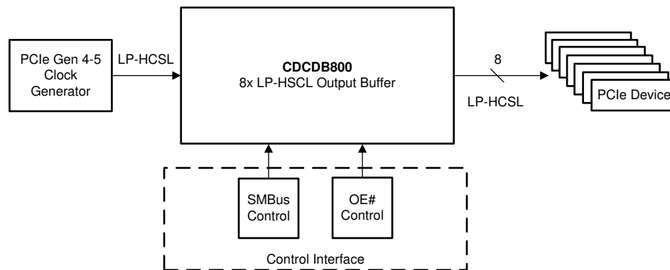
图 9-1. Typical Application
