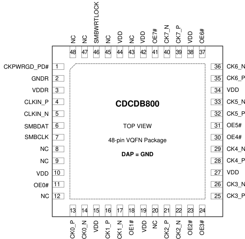
图 5-1. CDCDB800 RSL Package 48-Pin VQFN Top View
