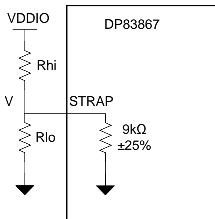
Figure 24. Strap Circuit
