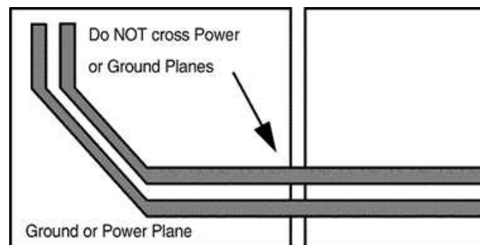
图 37. Differential Signal Pair-Plane Crossing
