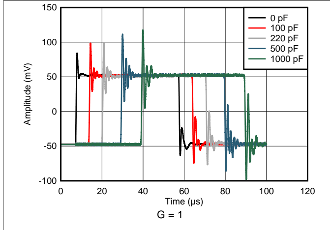
Figure 37. Small-Signal Response vs Capacitive Load
