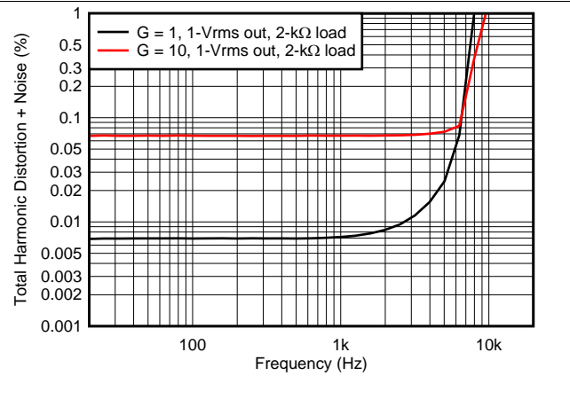
Figure 38. Total Harmonic Distortion + Noise vs Frequency
