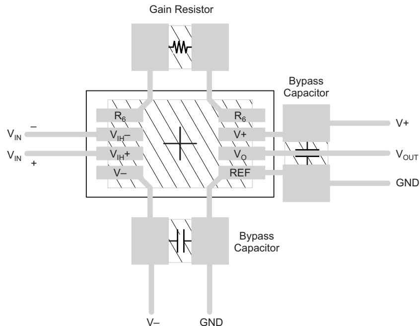
Figure 36. Recommended Layout
