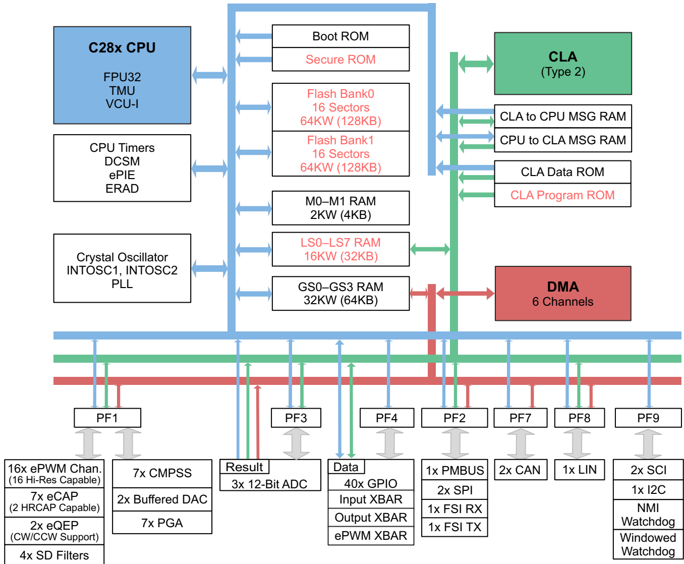
图 3-1. Functional Block Diagram
