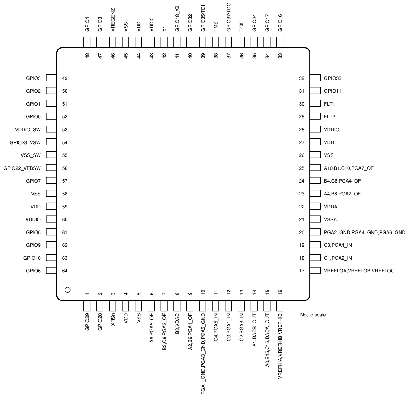
图 6-3. F280048/C, F280040/C 64-Pin PM Low-Profile Quad Flatpack — Q-Temperature (Top View)
