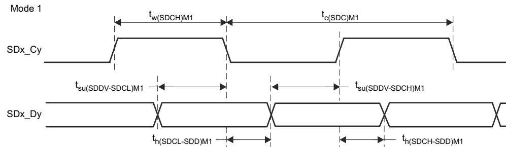
图 7-66. SDFM Timing Diagram - Mode 1
