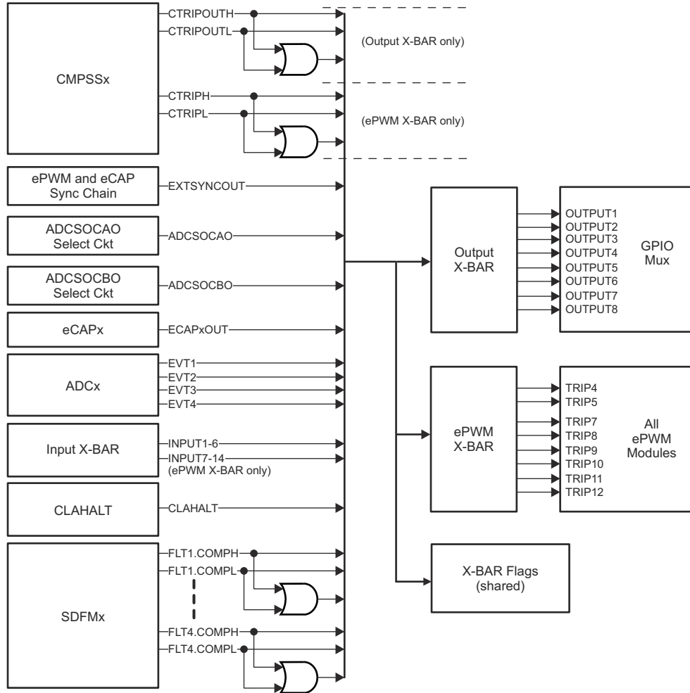
图 6-6. Output X-BAR and ePWM X-BAR Sources
