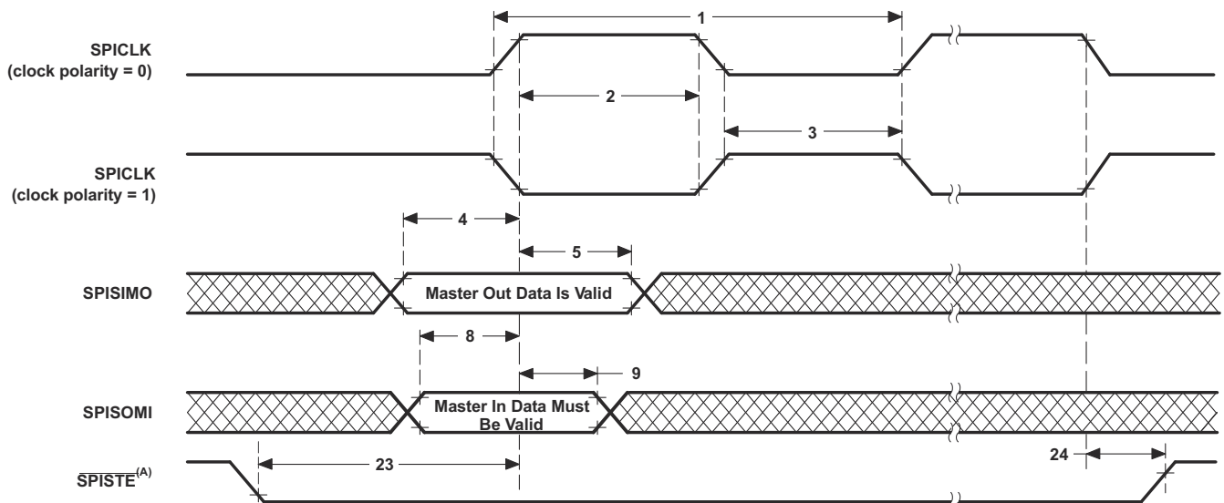
图 7-75. SPI Master Mode External Timing (Clock Phase = 0)
