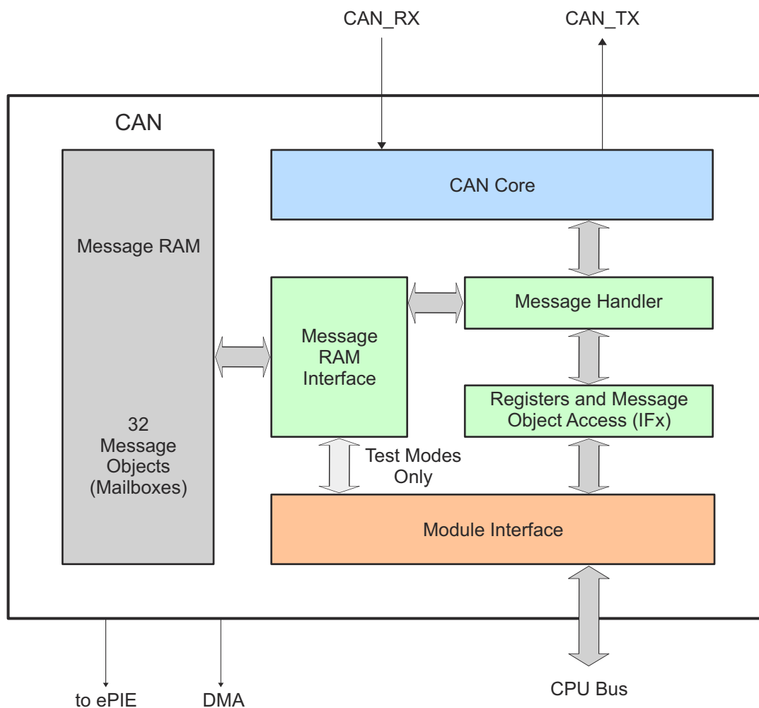
图 7-69. CAN Block Diagram
