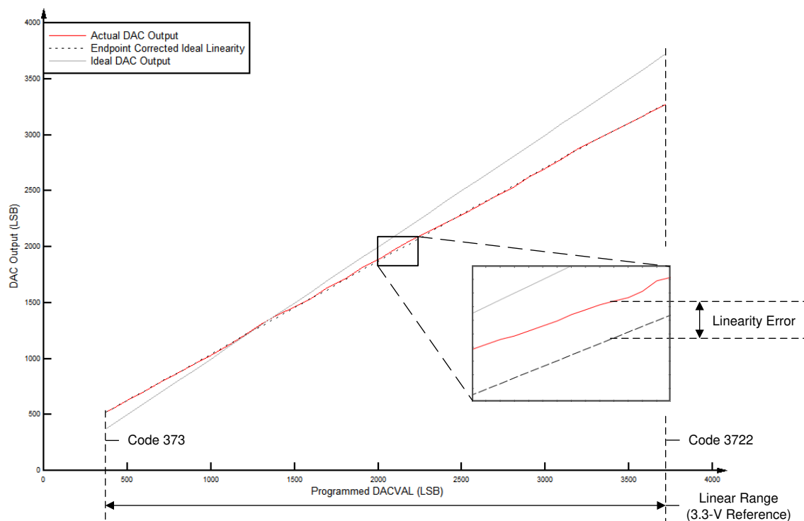
图 7-41. Buffered DAC Linearity
