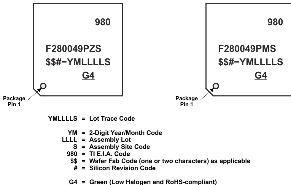
图 10-2. Examples of Device Markings for PM and PZ Packages
