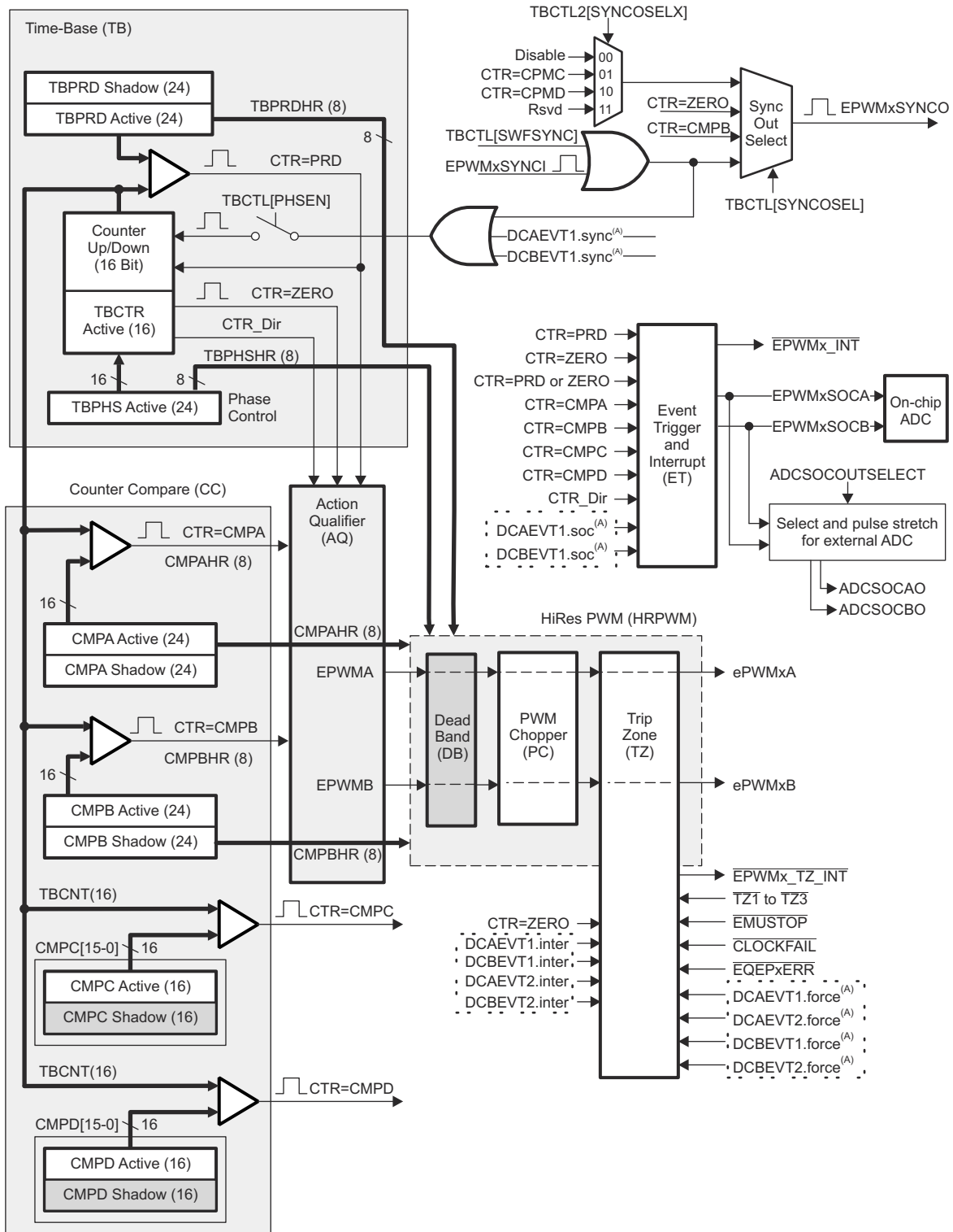
图 7-58. ePWM Submodules and Critical Internal Signal Interconnects
