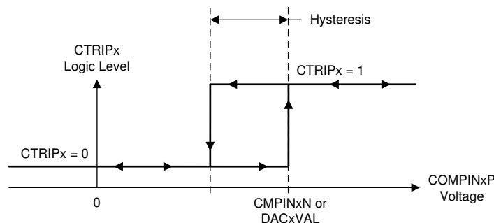
图 7-50. CMPSS Comparator Hysteresis
