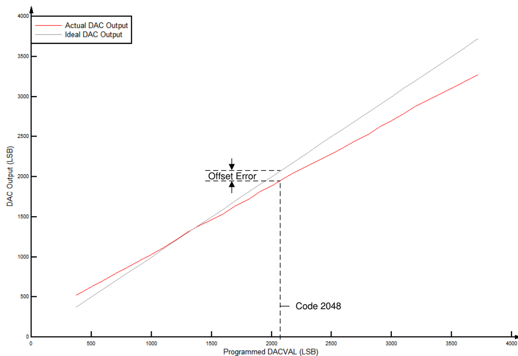
图 7-39. Buffered DAC Offset
