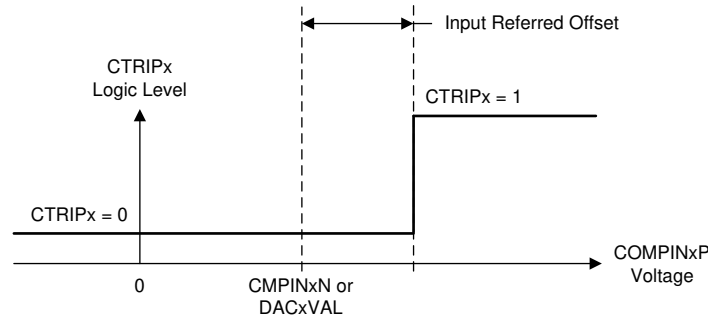
图 7-49. CMPSS Comparator Input Referred Offset
