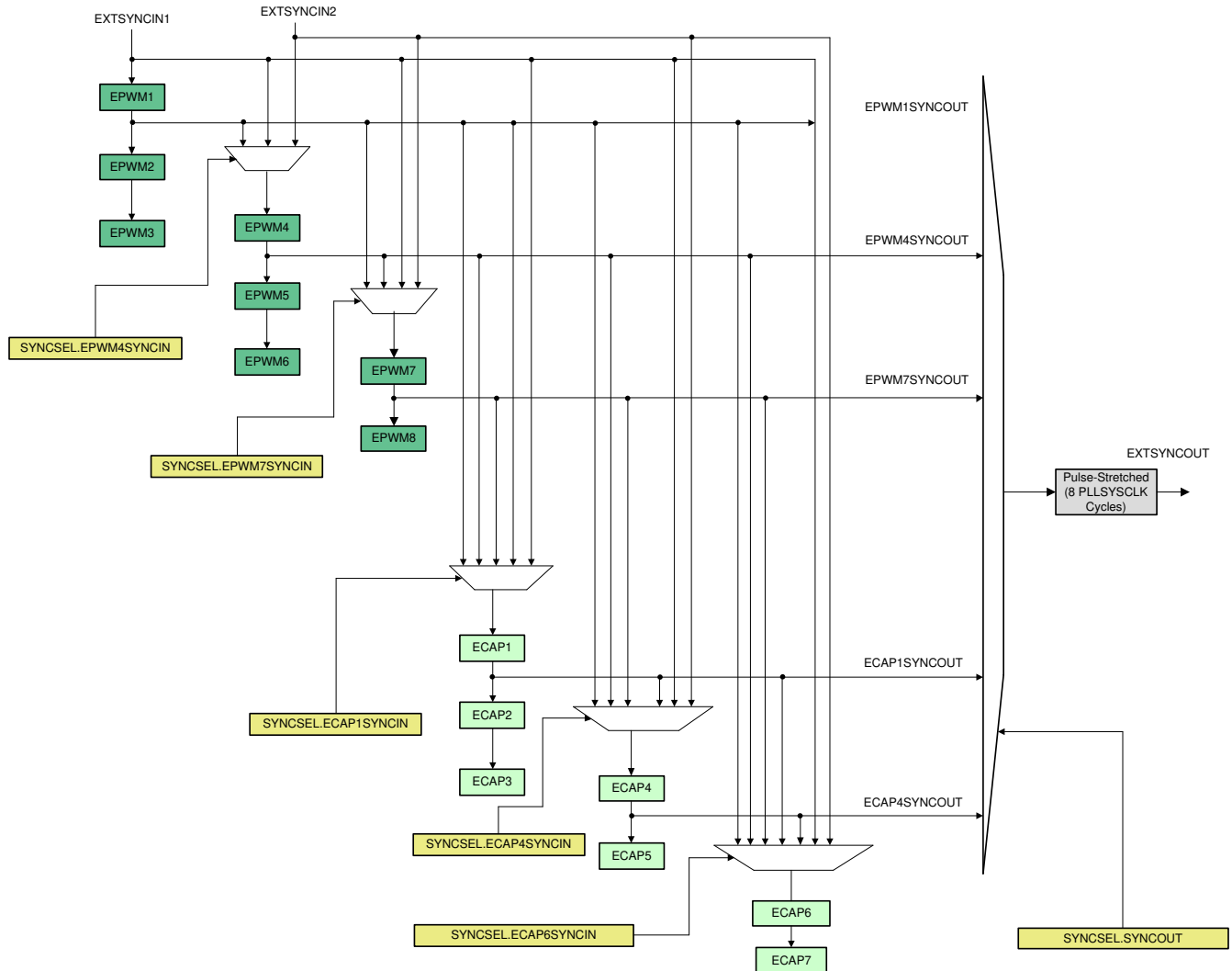
图 7-60. Synchronization Chain Architecture
