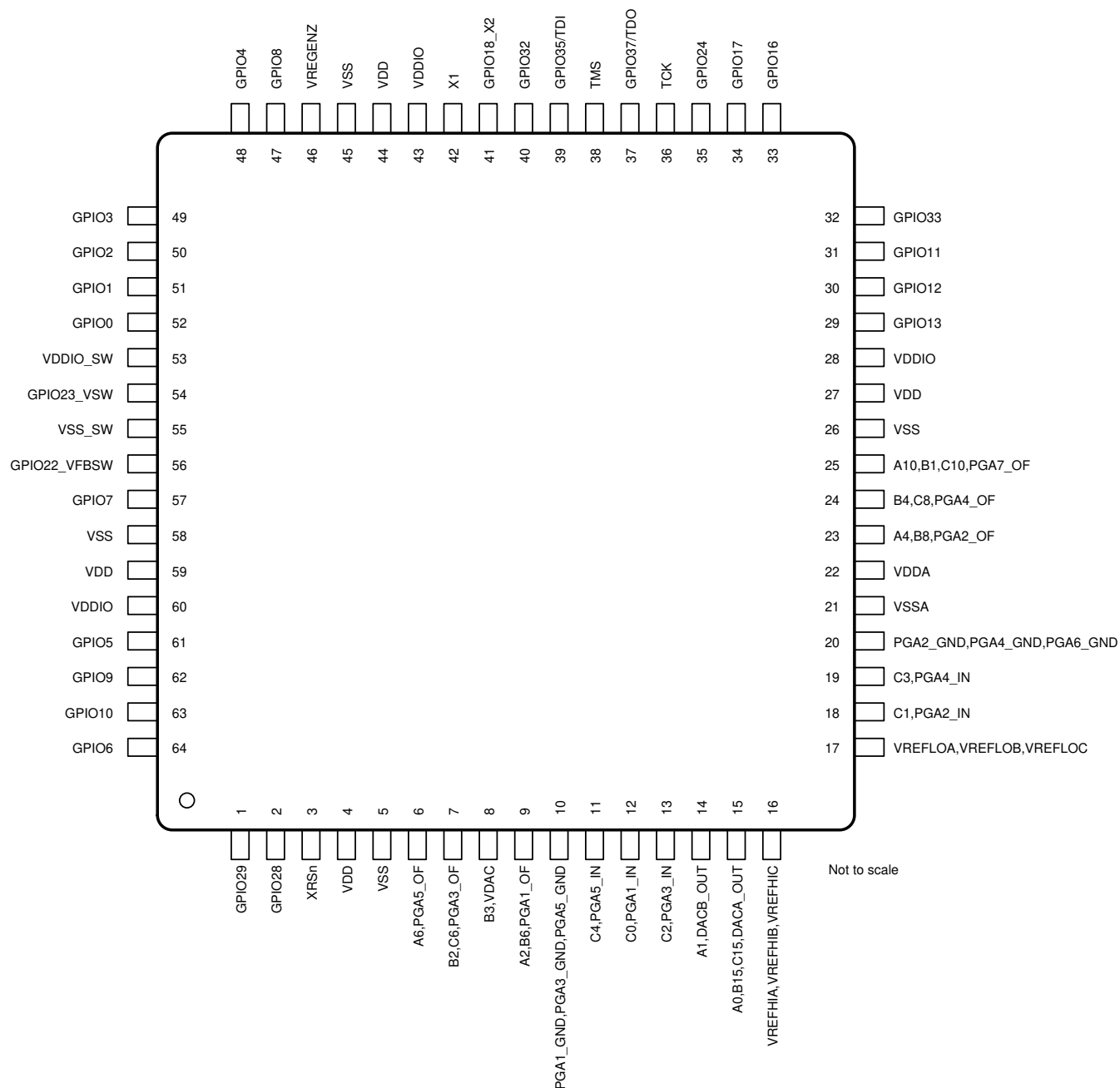
图 6-2. F280049/C/M, F280045, F280041/C 64-Pin PM Low-Profile Quad Flatpack (Top View)
