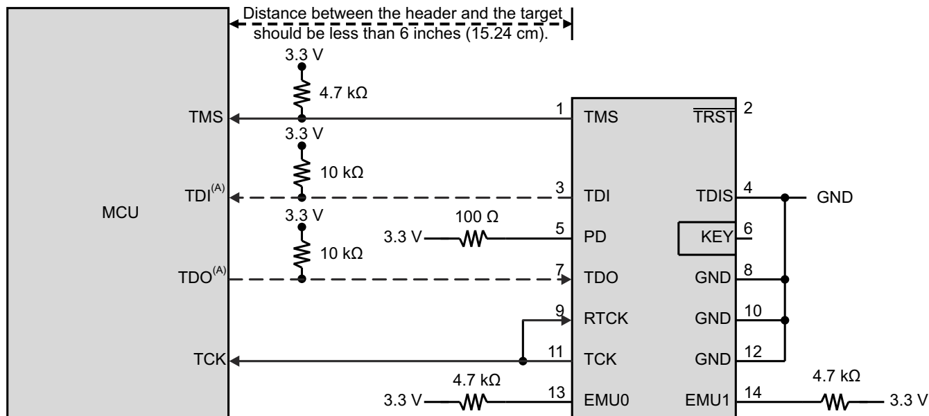
图 7-17. Connecting to the 14-Pin JTAG Header
