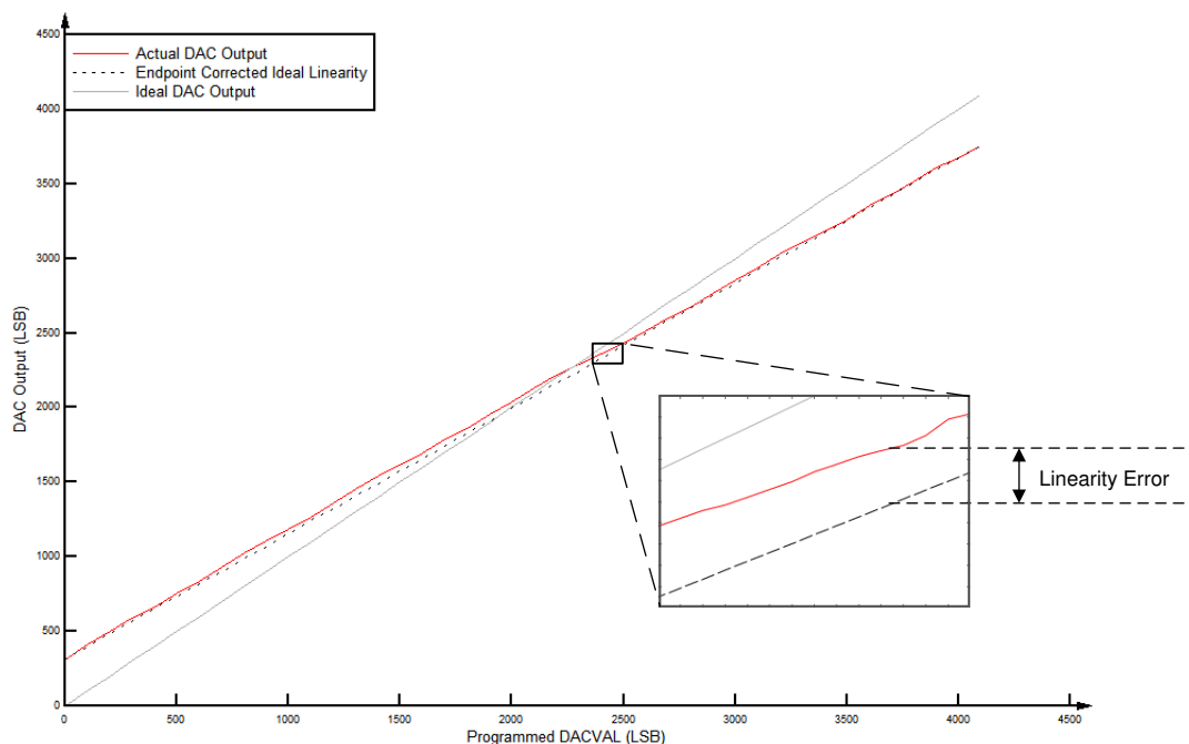
图 7-53. CMPSS DAC Static Linearity
