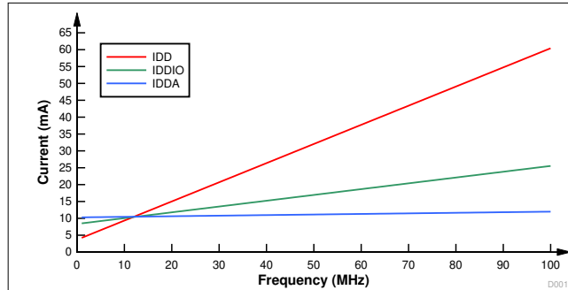
图 7-2. Current Versus Frequency — External Supply
