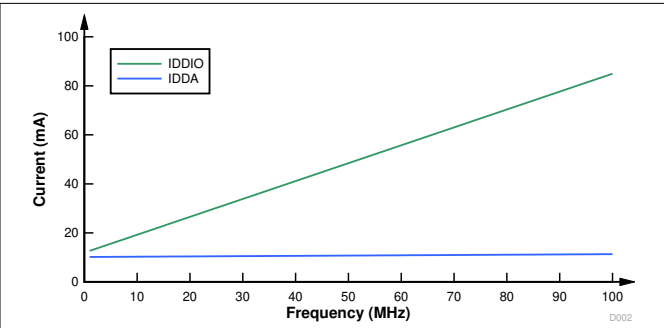
图 7-3. Current Versus Frequency — Internal VREG
