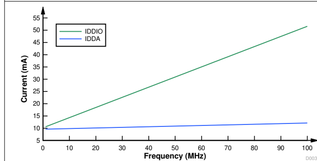
图 7-4. Current Versus Frequency — DCDC
