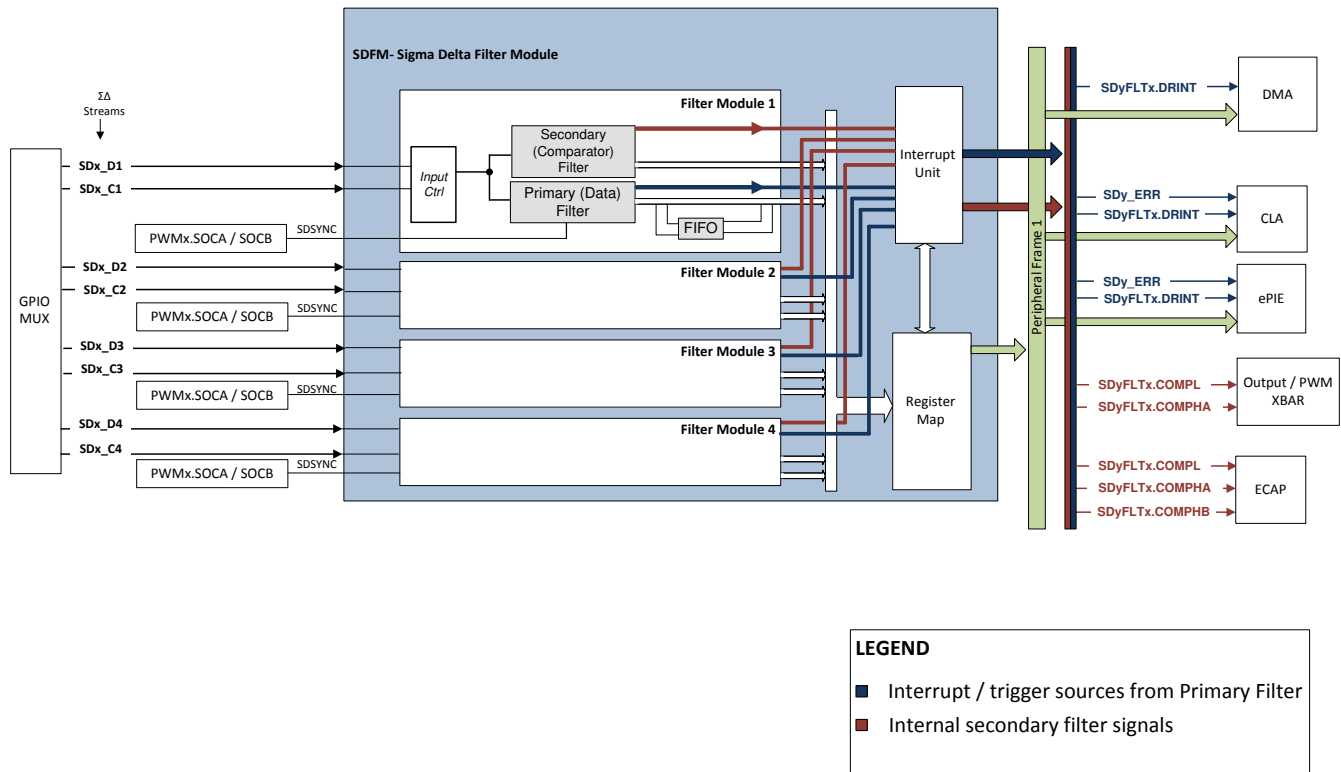
图 7-64. SDFM Block Diagram
