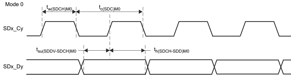
图 7-65. SDFM Timing Diagram - Mode 0
