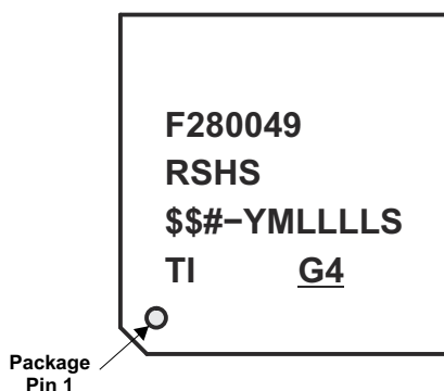
图 10-3. Example of Device Markings for RSH Package
