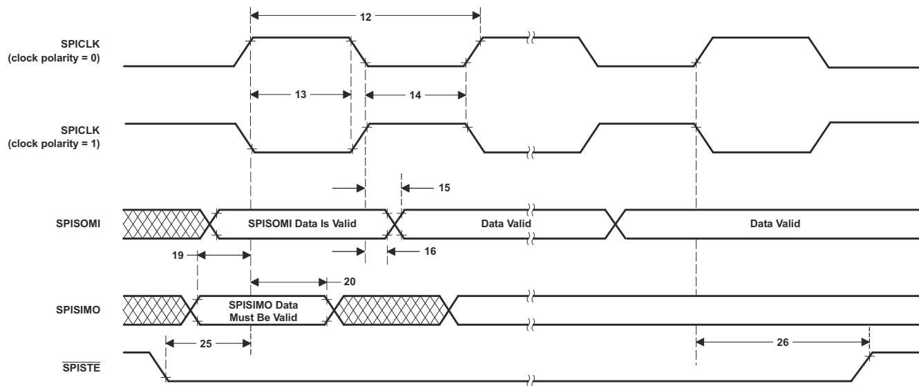
图 7-82. High-Speed SPI Slave Mode External Timing (Clock Phase = 1)
