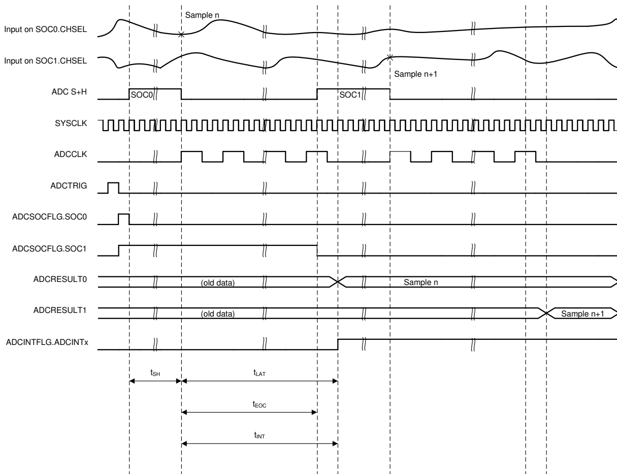
图 7-35. ADC Timings
