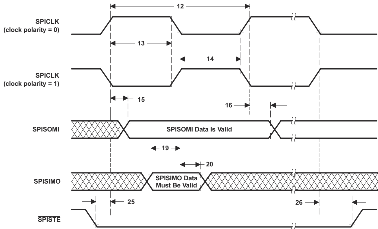
图 7-77. SPI Slave Mode External Timing (Clock Phase = 0)
