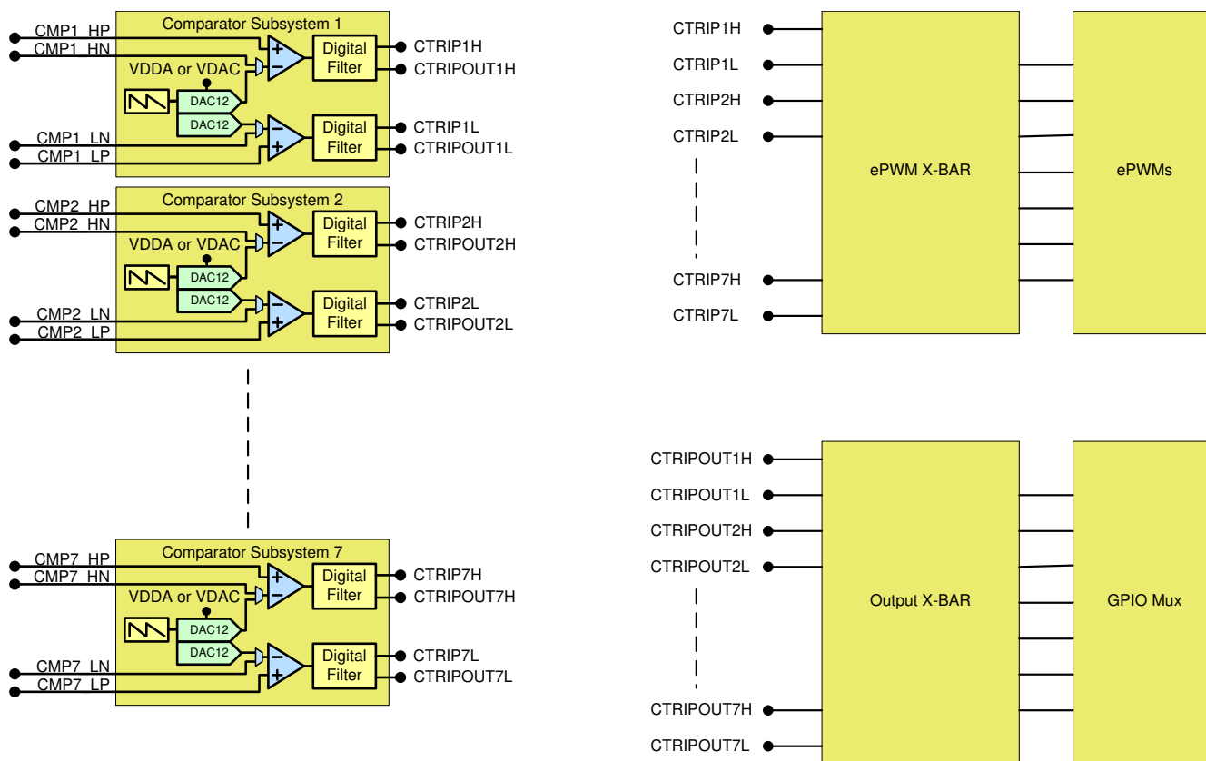
图 7-48. CMPSS Connectivity
