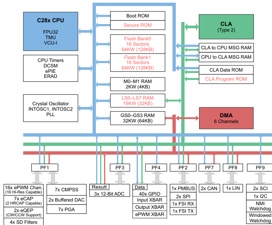
图 8-1. Functional Block Diagram
