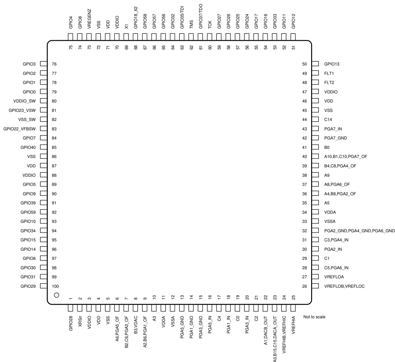
图 6-1. 100-Pin PZ Low-Profile Quad Flatpack (Top View)
