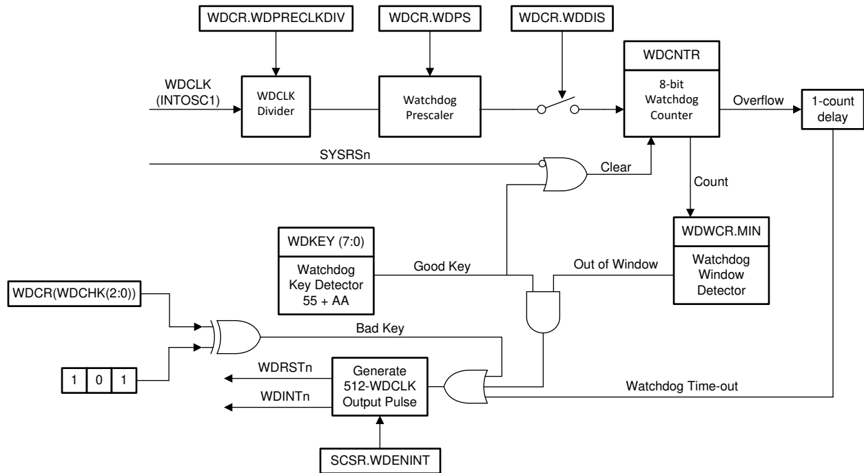
图 8-4. Windowed Watchdog
