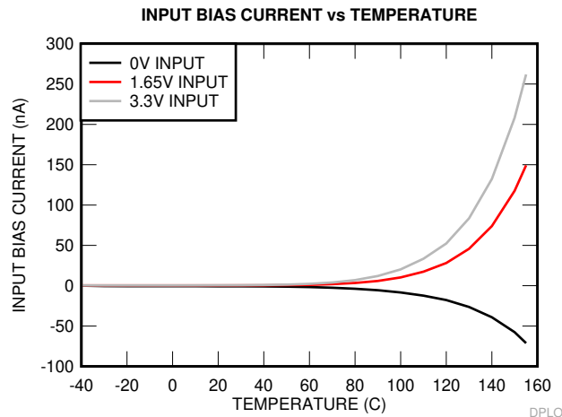
图 7-37. Input Bias Current Versus Temperature
