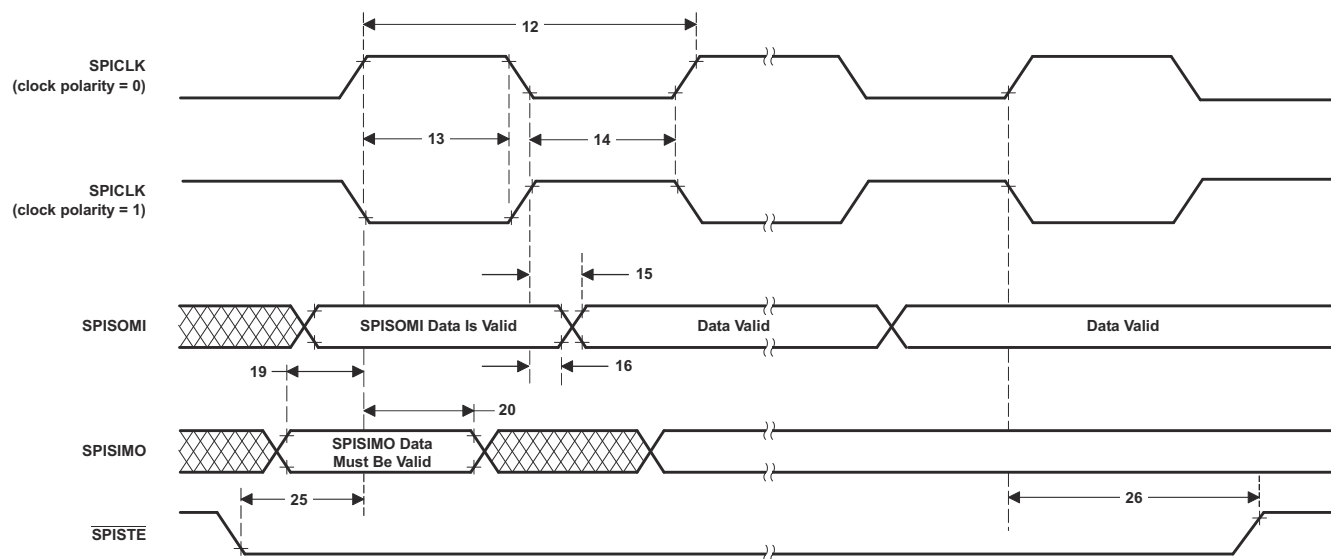
图 7-78. SPI Slave Mode External Timing (Clock Phase = 1)
