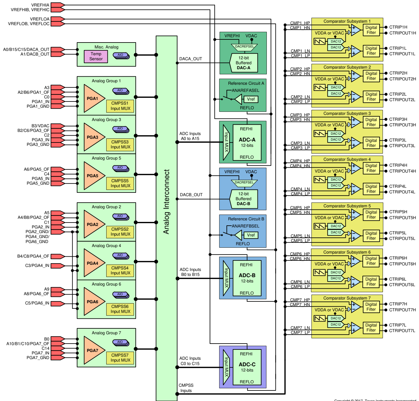
图 7-28. Analog Subsystem Block Diagram (100-Pin PZ LQFP)
