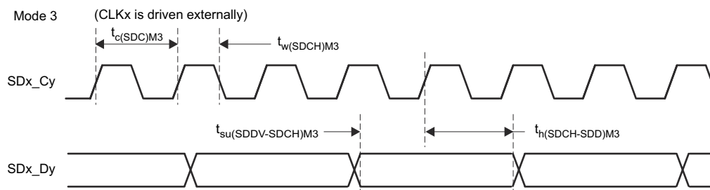
图 7-68. SDFM Timing Diagram - Mode 3
