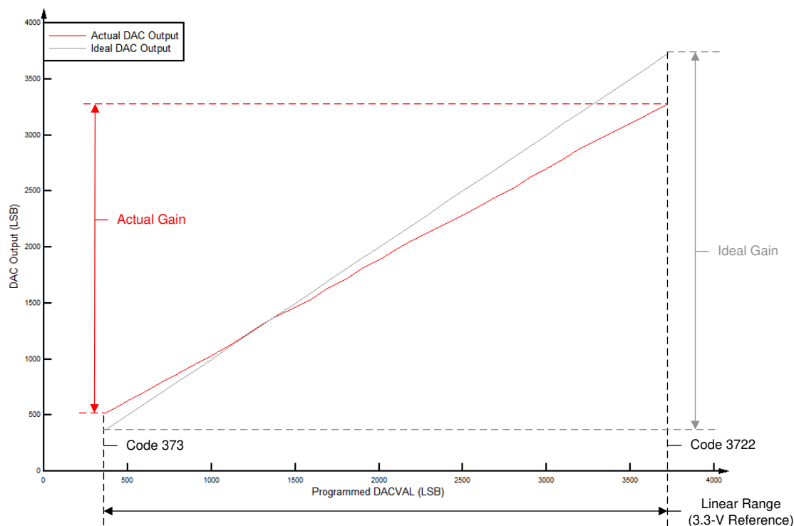
图 7-40. Buffered DAC Gain
