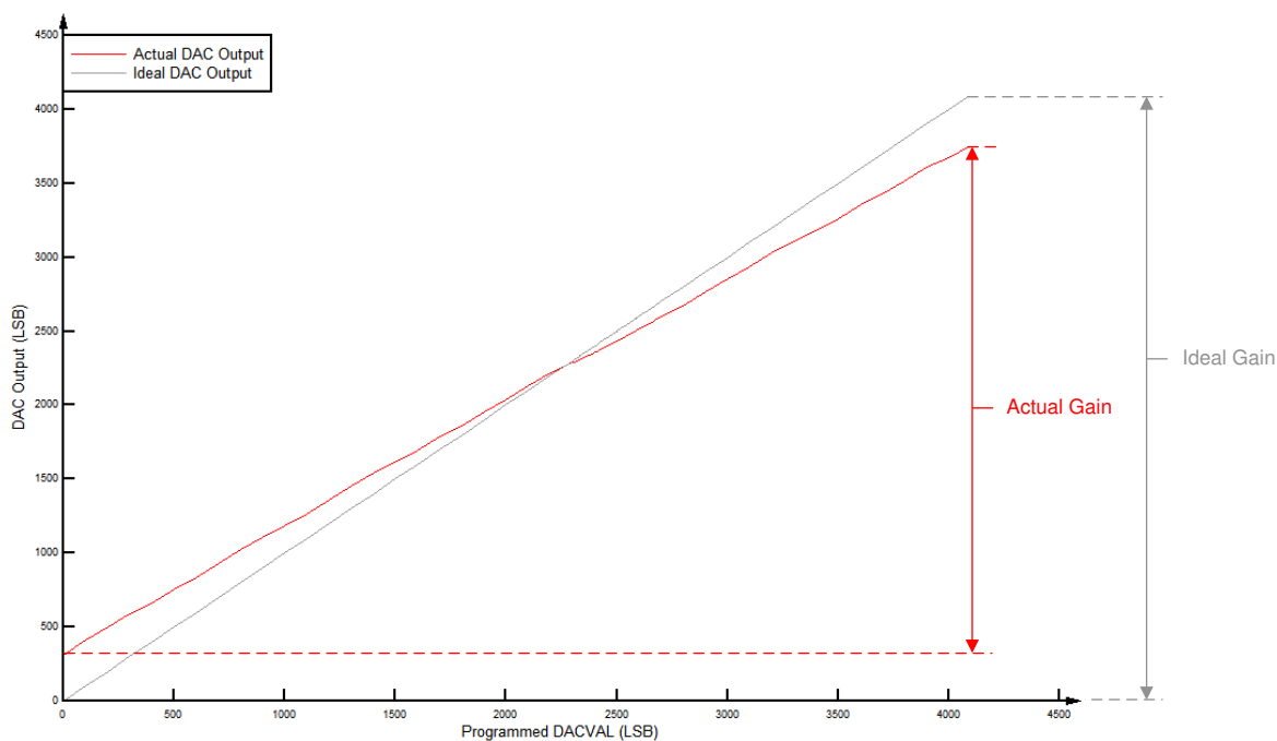
图 7-52. CMPSS DAC Static Gain
