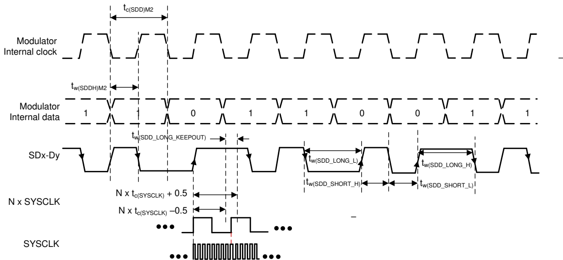
图 7-67. SDFM Timing Diagram - Mode 2
