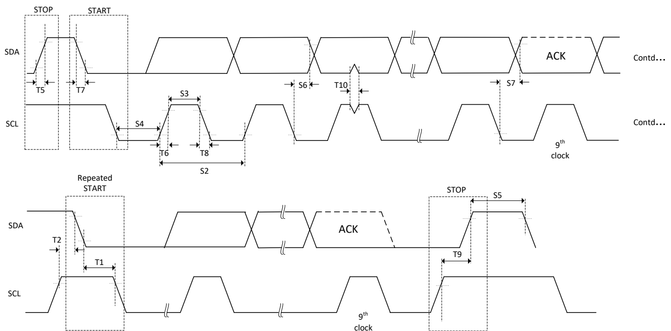
图 7-71. I2C Timing Diagram
