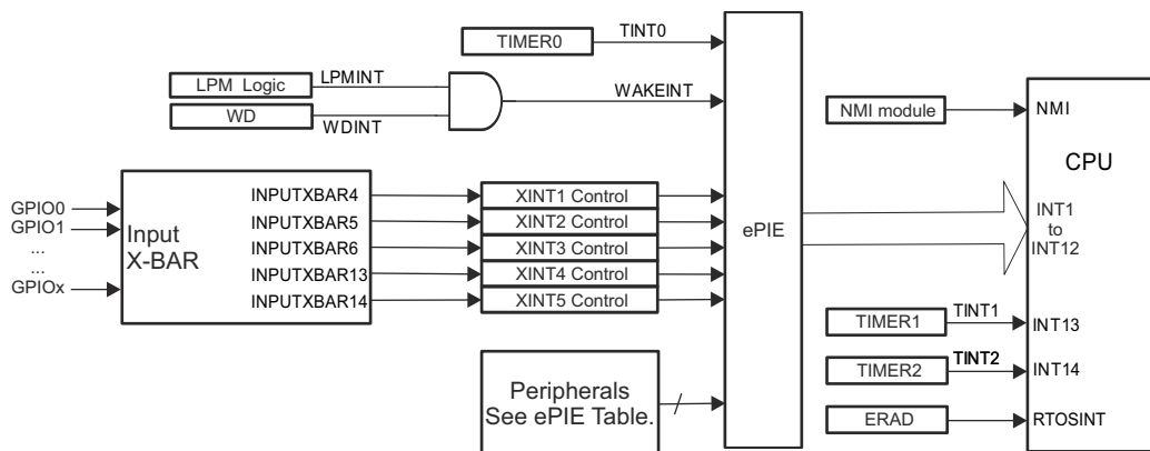
图 7-24. Device Interrupt Architecture
