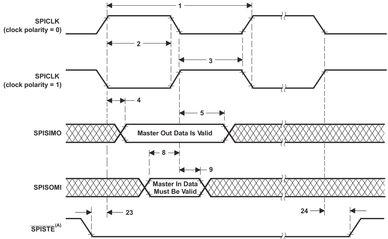
图 7-79. High-Speed SPI Master Mode External Timing (Clock Phase = 0)
