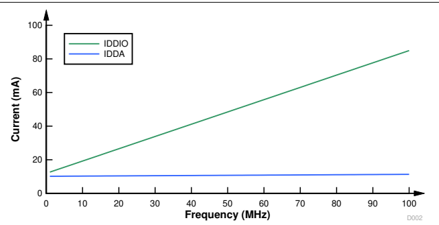
图 7-3. Current Versus Frequency — Internal VREG
