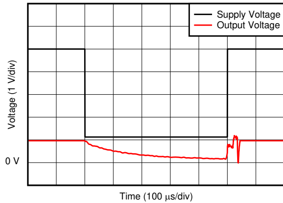
V_S = 5.0\text{ V} , A3 devices 图 6-18. Brownout Recovery
