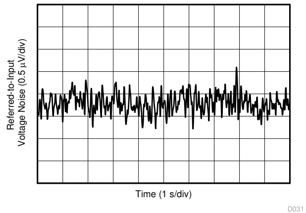
图 6-12. 0.1-Hz to 10-Hz Voltage Noise (Referred-To-Input)
