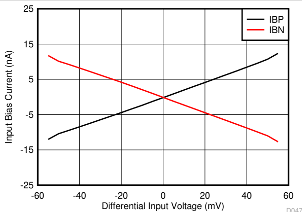
V_S = 5.0\text{ V} , V_{\text{REF}} = 2.5\text{ V} , A2, A3, A4, A5 devices 图 6-21. IB+ and IB- vs. Differential Input Voltage
