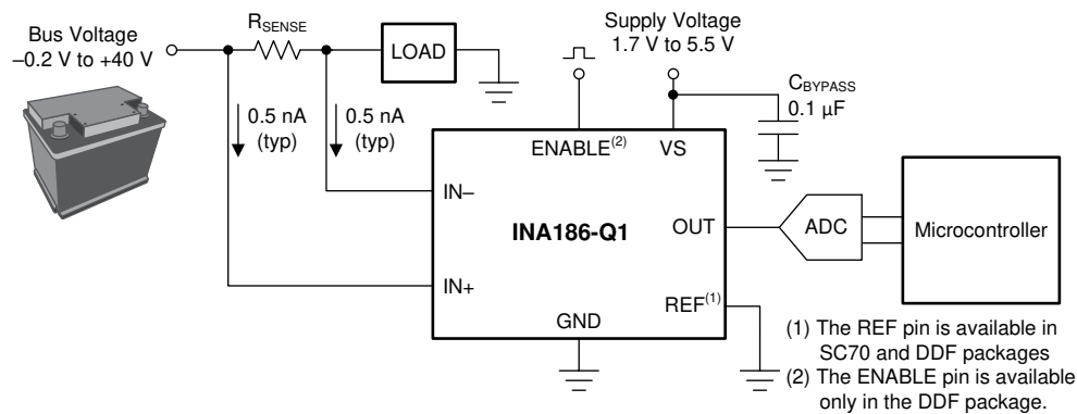
图 8-1. Basic Connections
