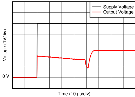
V_S = 5.0\text{ V} , A3 devices 图 6-17. Start-Up Response
