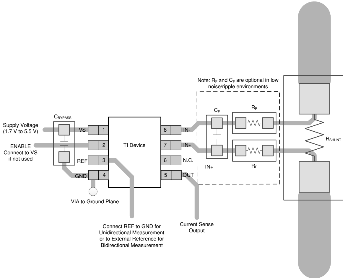
图 10-2. Recommended Layout for SOT-23 (DDF) Package
