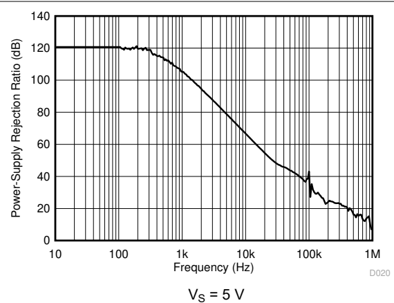
图 6-2. Power-Supply Rejection Ratio vs. Frequency
