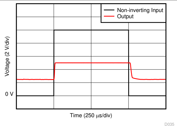
图 6-14. Common-Mode Voltage Transient Response
