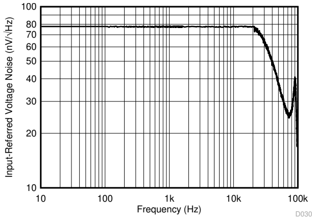
图 6-11. Input-Referred Voltage Noise vs. Frequency
