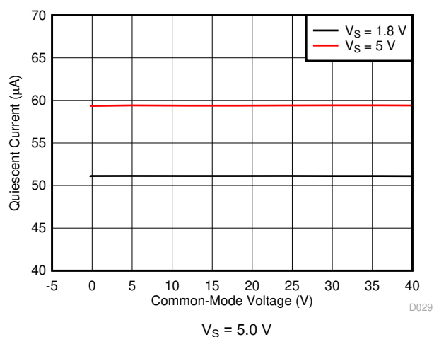
图 6-10. Quiescent Current vs. Common-Mode Voltage
