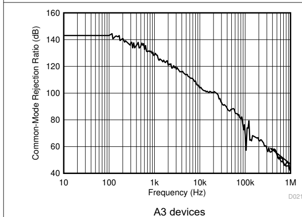
图 6-3. Common-Mode Rejection Ratio vs. Frequency
