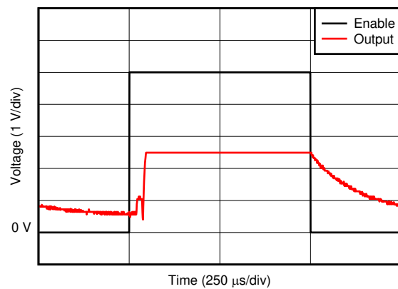
V_S = 5.0\text{ V} , A3 devices 图 6-19. Enable and Disable Response
