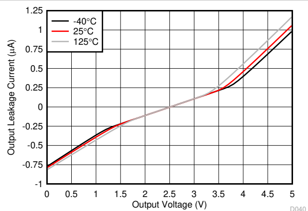
V_S = 5.0\text{ V} , V_{\text{ENABLE}} = 0\text{ V} , V_{\text{REF}} = 2.5\text{ V} 图 6-22. Output Leakage vs. Output Voltage (A1, A2, and A3 Devices)
