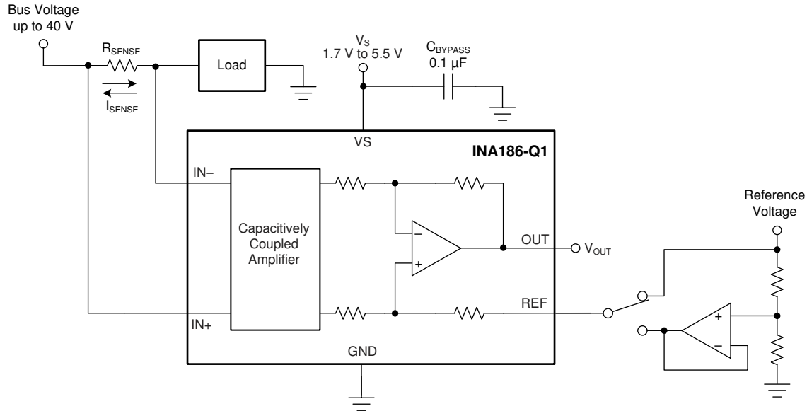
图 7-4. Bidirectional Application
