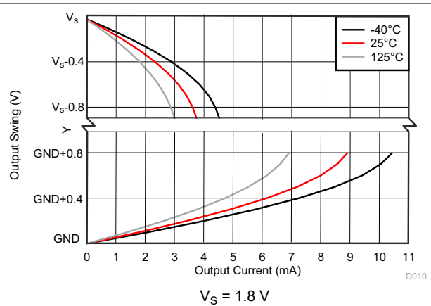
图 6-4. Output Voltage Swing vs. Output Current
