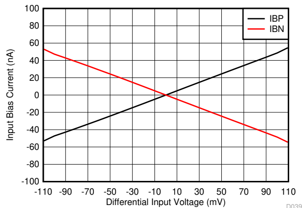
V_S = 5.0\text{ V} , V_{\text{REF}} = 2.5\text{ V} , A1 devices 图 6-20. IB+ and IB- vs. Differential Input Voltage
