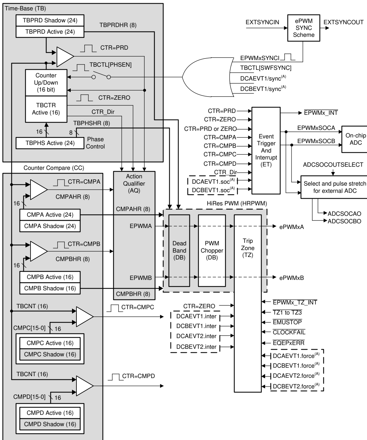
图 7-50. ePWM Submodules and Critical Internal Signal Interconnects
