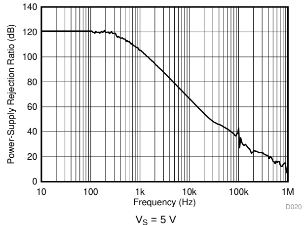
图 2. Power-Supply Rejection Ratio vs Frequency
