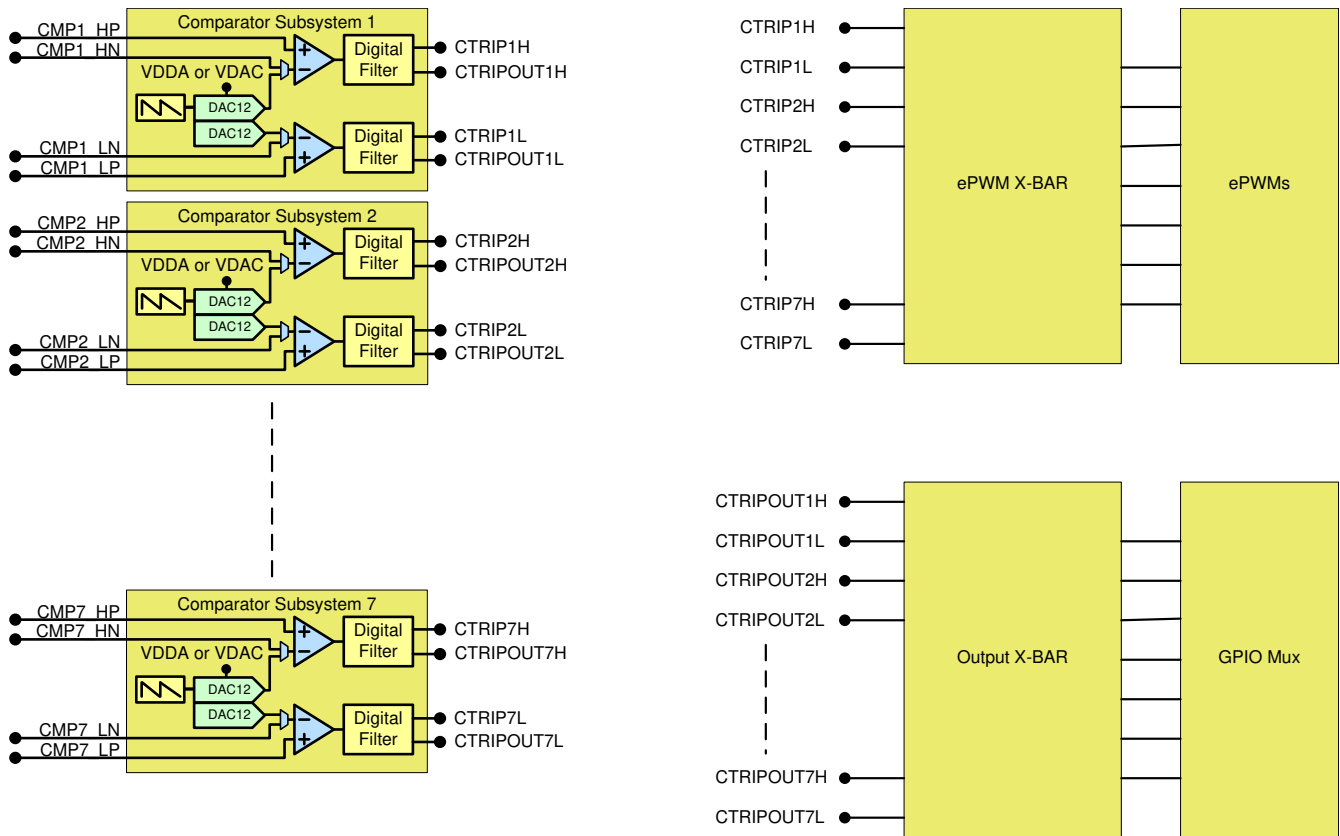
图 7-48. CMPSS Connectivity
