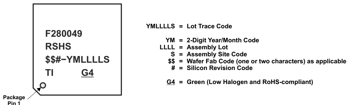
图 10-3. Example of Device Markings for RSH Package
