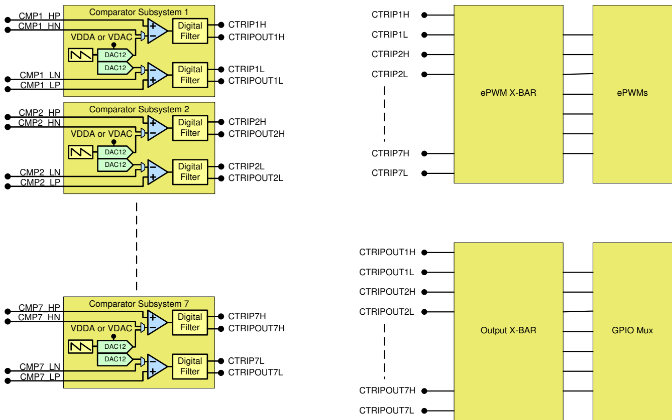
图 7-48. CMPSS Connectivity
