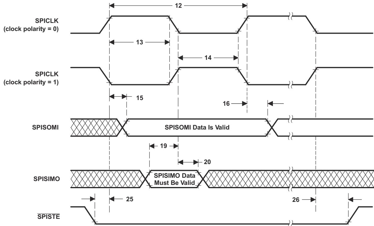
图 7-77. SPI Slave Mode External Timing (Clock Phase = 0)
