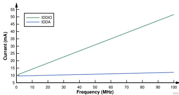
图 7-4. Current Versus Frequency — DCDC
