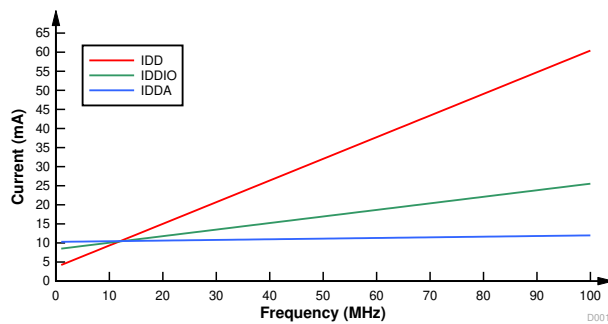
图 7-2. Current Versus Frequency — External Supply
