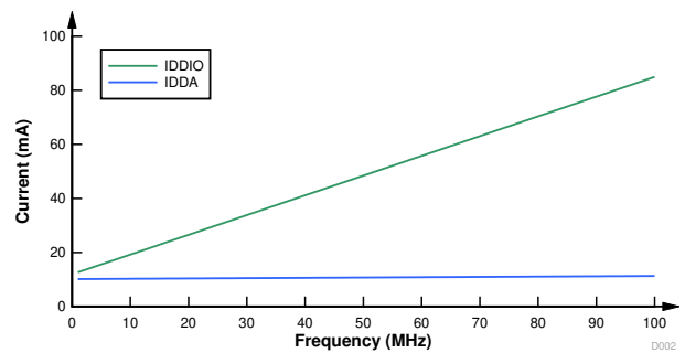
图 7-3. Current Versus Frequency — Internal VREG
