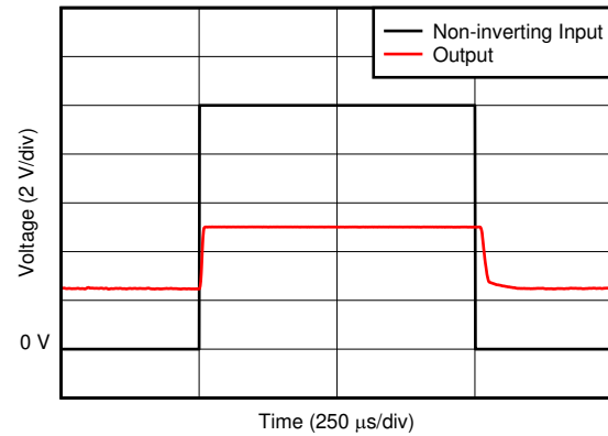
图 14. Common-Mode Voltage Transient Response
