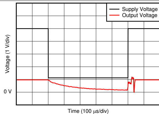
图 16. Noninverting Differential Input Overload
