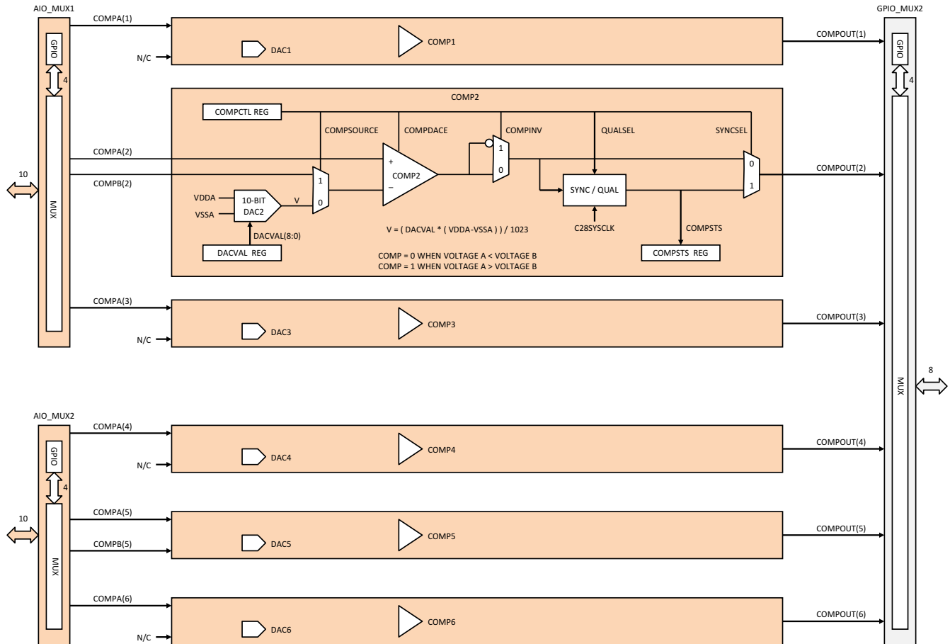
图 7-13. Comparator + DAC Units
