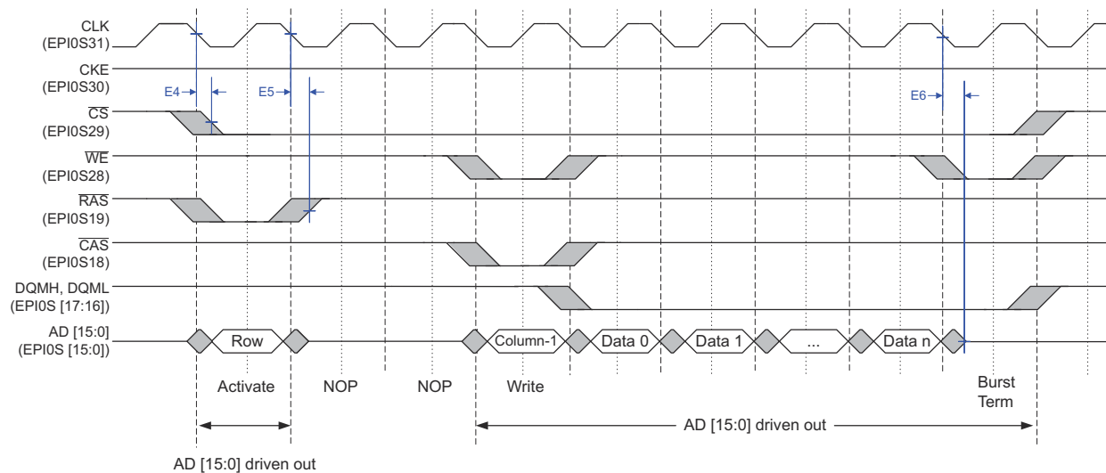
图 7-23. SDRAM Write Timing
