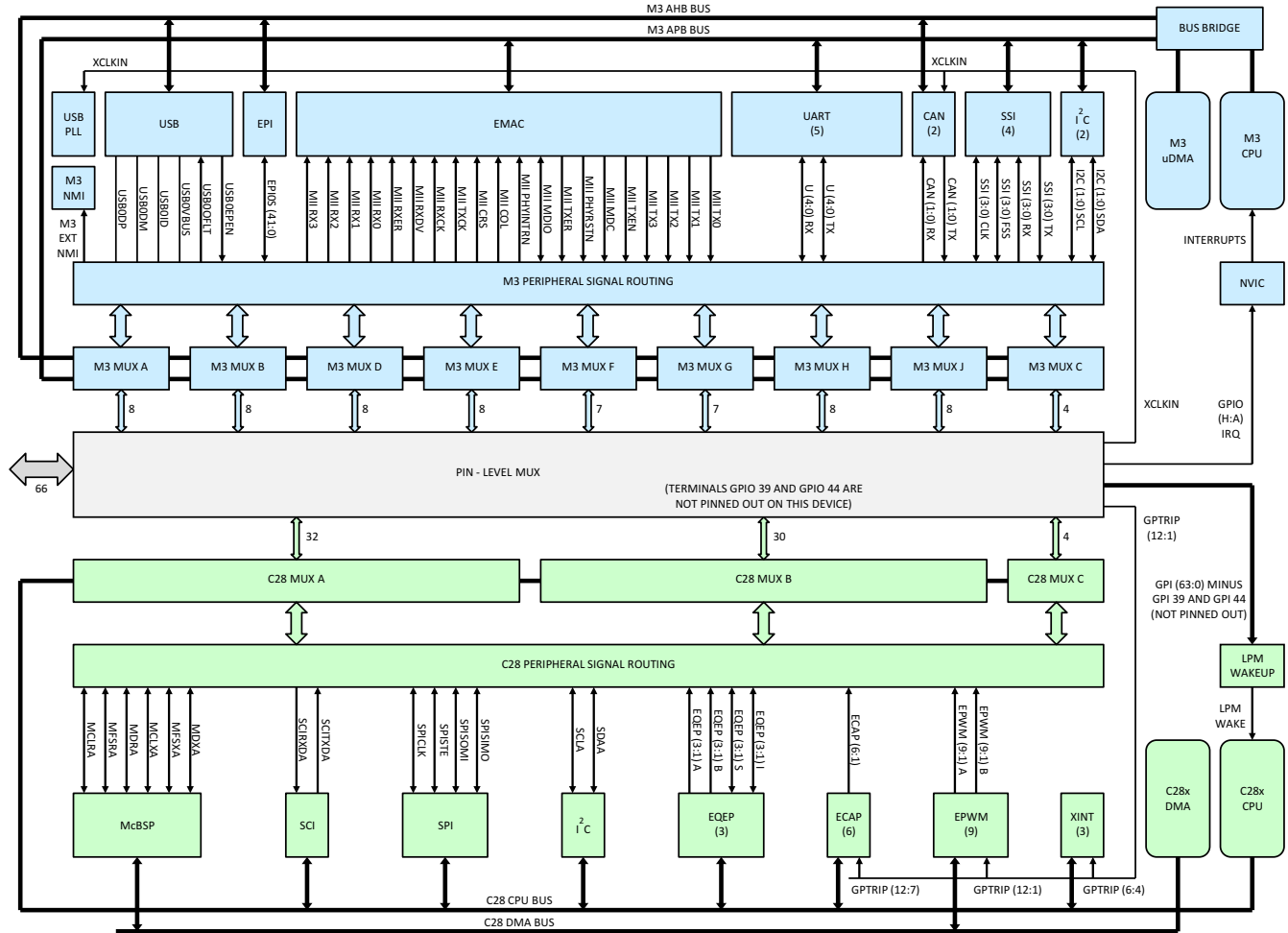
8-15. GPIO_MUX1 Block
