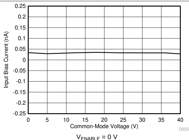
图 7. Input Bias Current vs Common-Mode Voltage (Shutdown)
