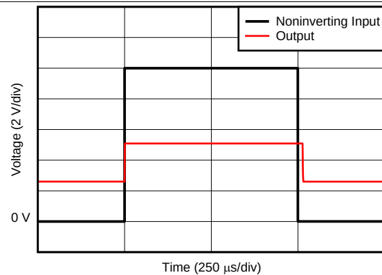
图 32. Common-Mode Voltage Transient Response
