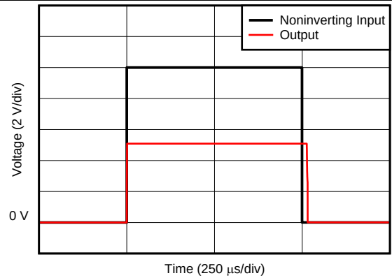
图 32. Common-Mode Voltage Transient Response
