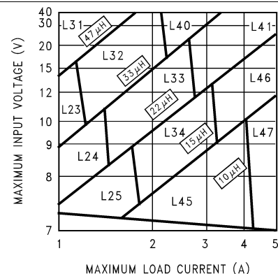
Figure 18. LM2678-5
