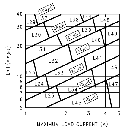
Figure 20. LM2678-Adjustable
