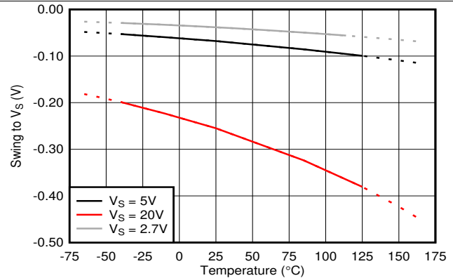
Figure 14. Swing to Supply vs Temperature
