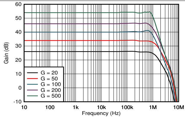
Figure 3. Gain vs Frequency
