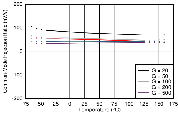
Figure 1. Common-Mode Rejection Ratio vs Temperature
