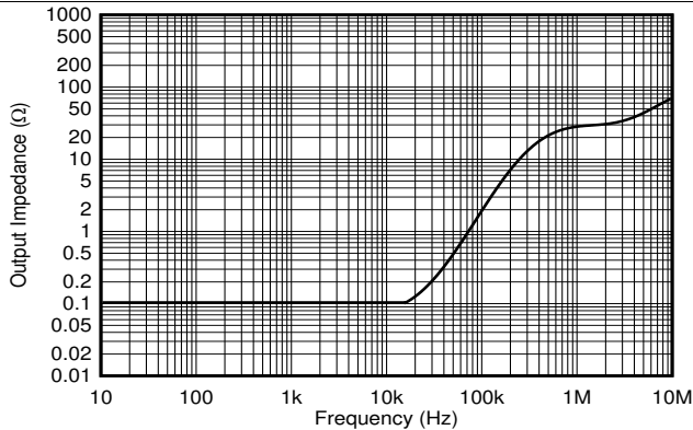
Figure 13. Output Impedance vs Frequency
