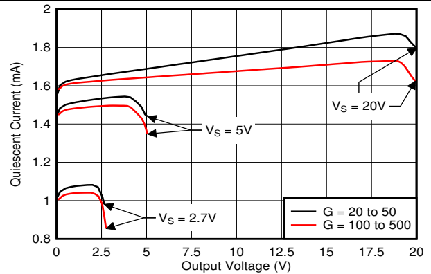
Figure 18. Quiescent Current vs Output Voltage
