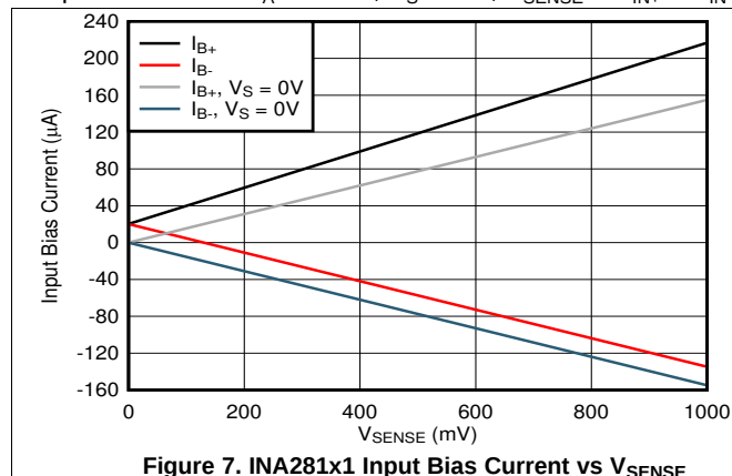
Figure 7. INA281x1 Input Bias Current vs V_{\text{SENSE}}
