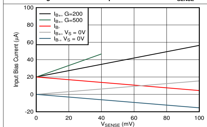
Figure 7. INA281x1 Input Bias Current vs V_{\text{SENSE}}
