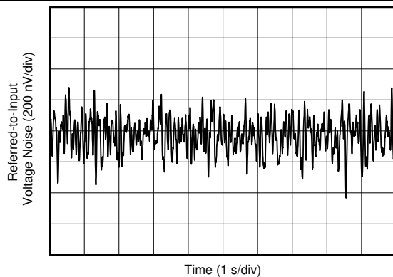
Figure 17. Input Referred Noise
