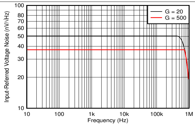
Figure 16. Input Referred Noise vs Frequency
