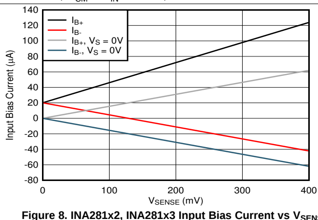
Figure 8. INA281x2, INA281x3 Input Bias Current vs V_{\text{SENSE}}
