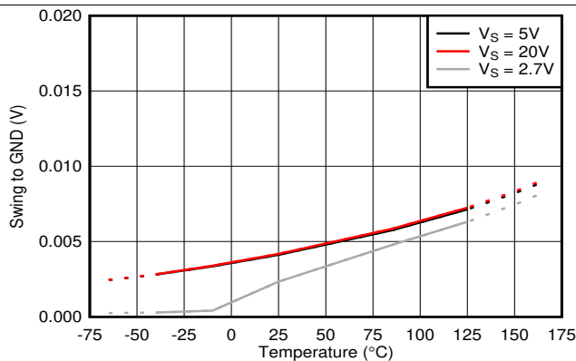
Figure 15. Swing to GND vs Temperature
