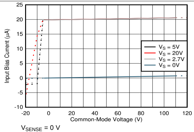
Figure 5. Input Bias Current vs Common-Mode Voltage
