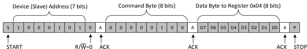
Figure 15. Write to the Fully On Register (0x04)
