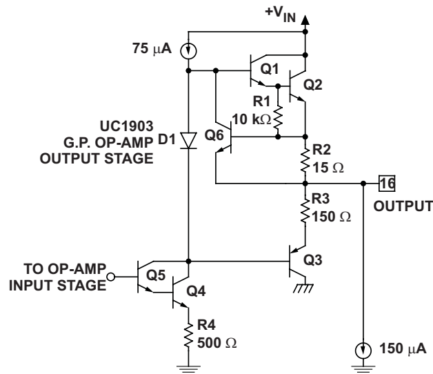
Figure 5. The G.P. Op-Amp on the UC1903
