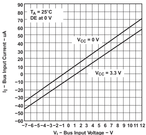
Figure 7-5. HVD11 or HVD12 Bus Input Current vs Bus Input Voltage
