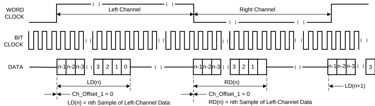
图 15. Left-Justified Mode With \text{Ch\_Offset}_1 = 0 , Bit Clock Inverted
