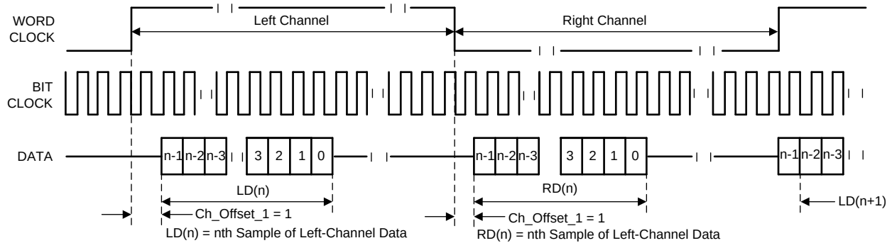
图 14. Left-Justified Mode With \text{Ch\_Offset}_1 = 1
