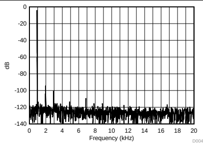
图 139. Line Input to ADC FFT Plot
