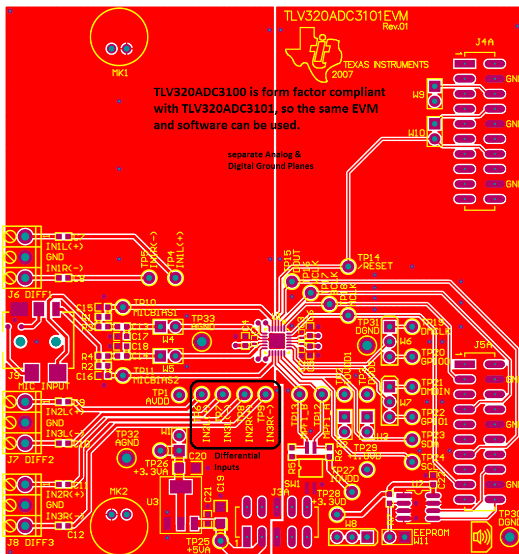
图 141. Layout Recommendation
