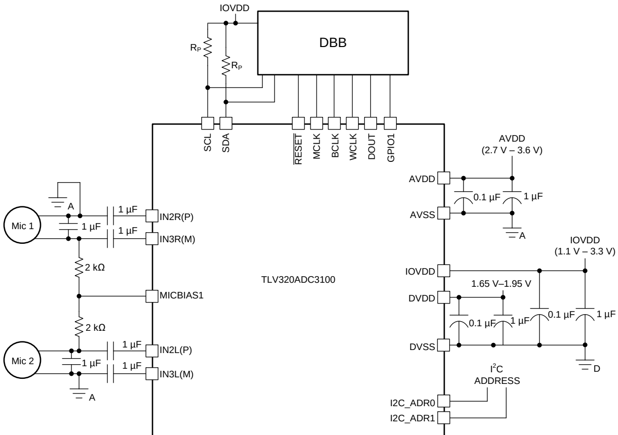
图 137. Typical Connections
