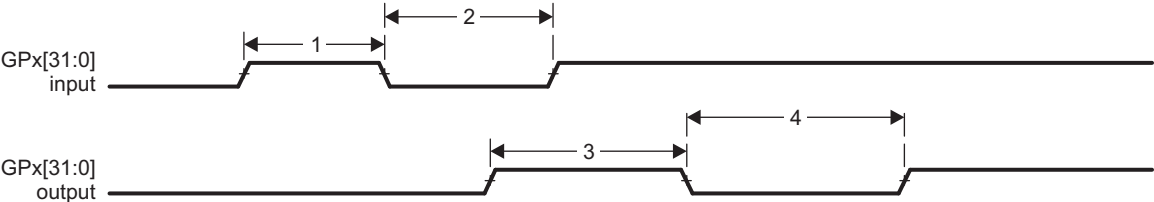
Figure 8-20. GPIO Port Timing
