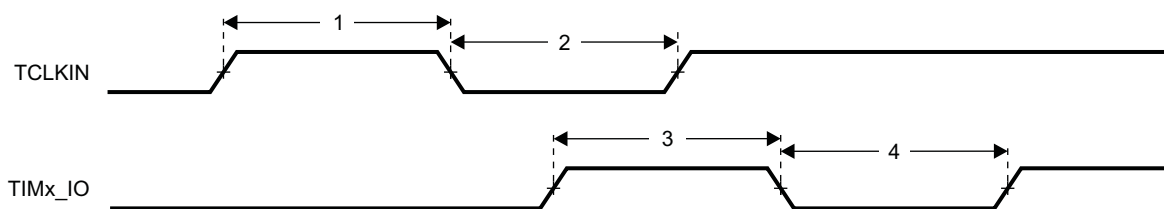
Figure 8-93. Timer Timing
