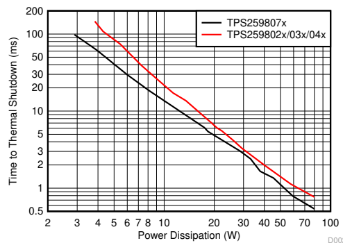
图 7-23. Thermal Shutdown Plot - Inrush/Overload
