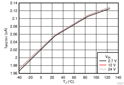
图 7-20. NRETRY Bias Current vs Temperature
