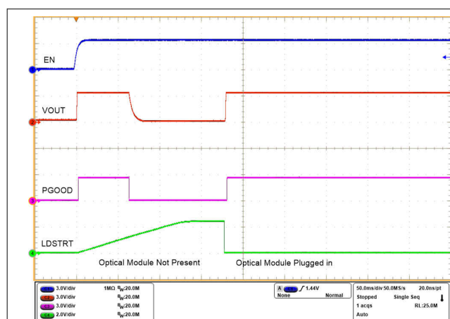
图 9-15. Output Voltage Profile When Optical Module is Inserted
