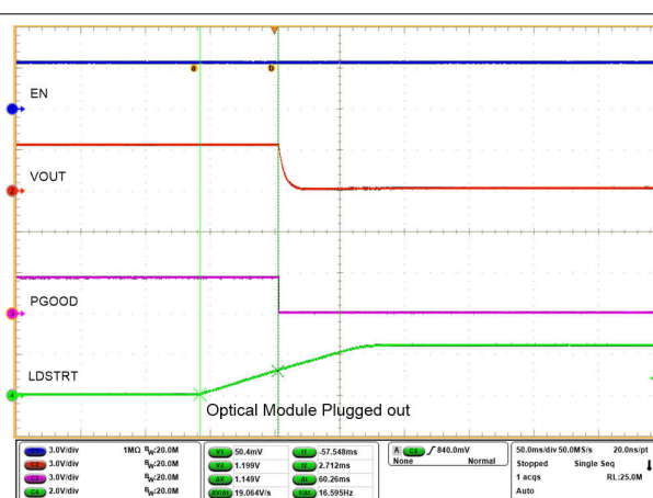
图 9-16. Output Voltage Profile When Optical Module is Plugged Out
