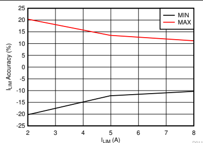
图 7-11. Output Current Limit ( I_{\text{LIM}} ) Accuracy
