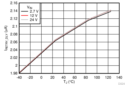
图 7-18. RETRY_DLY Bias Current vs Temperature
