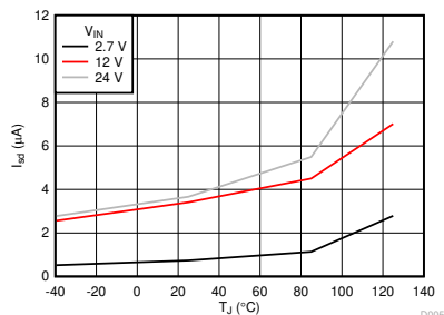
图 7-9. Deep Shut-Down Current vs Temperature
