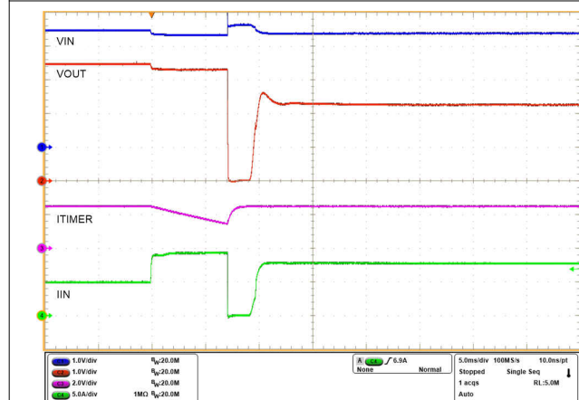
图 9-17. Circuit Breaker With Transient Overcurrent Blanking Interval of 6 ms; Device Restarts in Current Limit Mode
