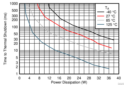
图 7-22. Thermal Shutdown Plot - Steady State
