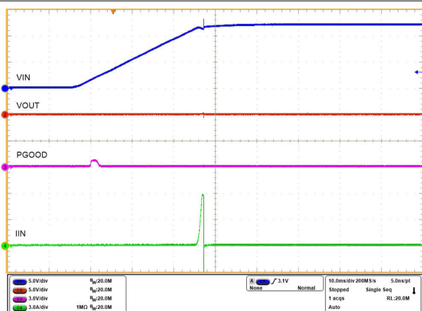
图 9-9. Power-Up With Short-Circuit on Output
