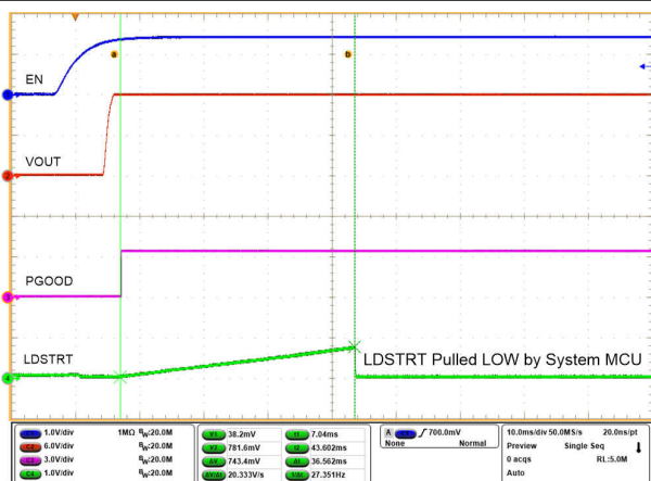
图 9-11. Successful Load Handshake (LDSTRT)
