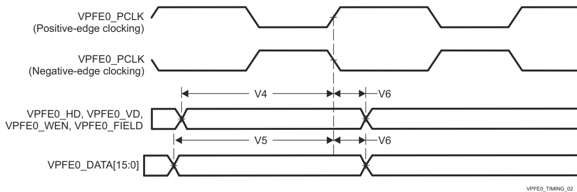
图 7-40. VPFE0 Timing Requirements
