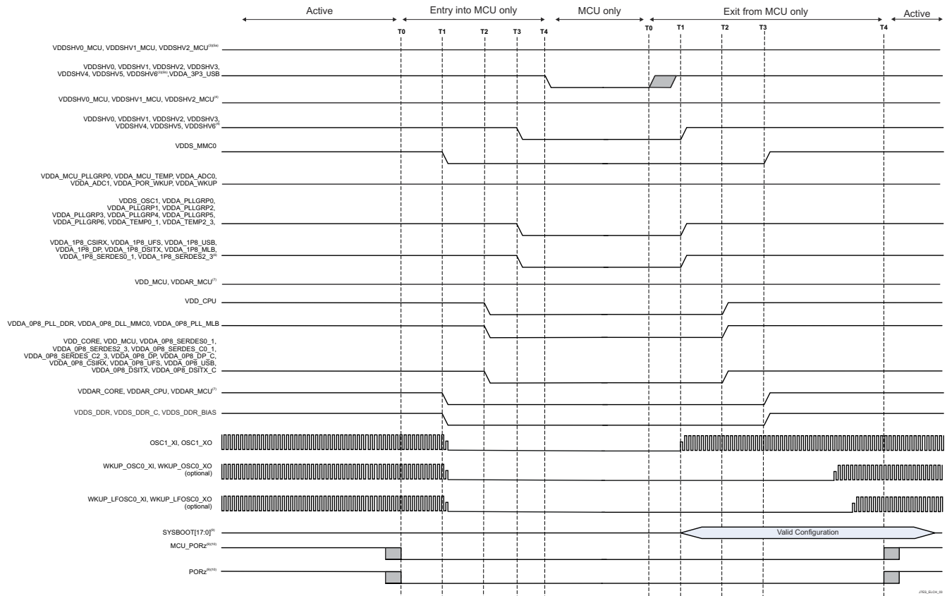
图 7-7. Entry and Exit of MCU Only Sequencing
