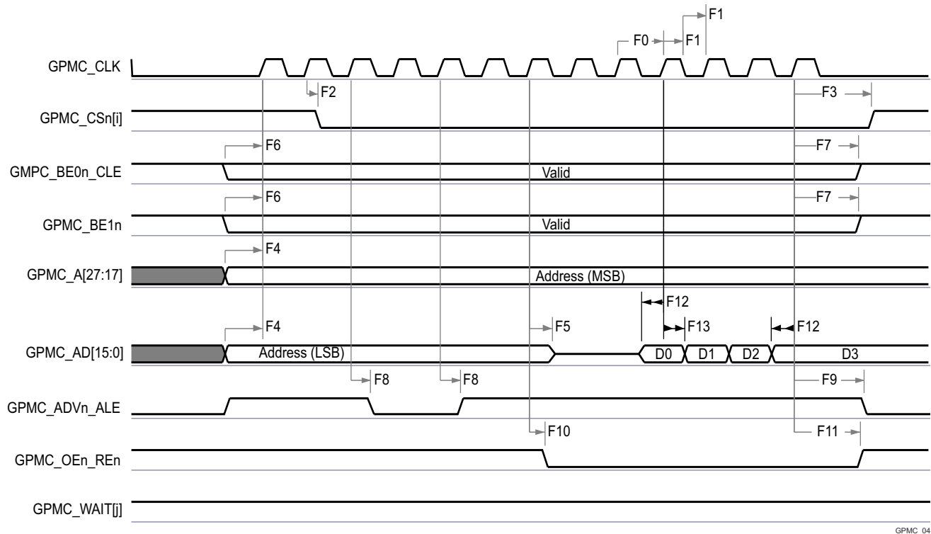
图 7-65. GPMC and NOR Flash—Synchronous Burst Write (GPMCFCLKDIVIDER = 0)
