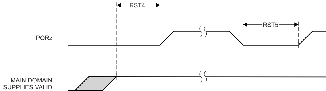
图 7-10. PORz Timing Requirements
