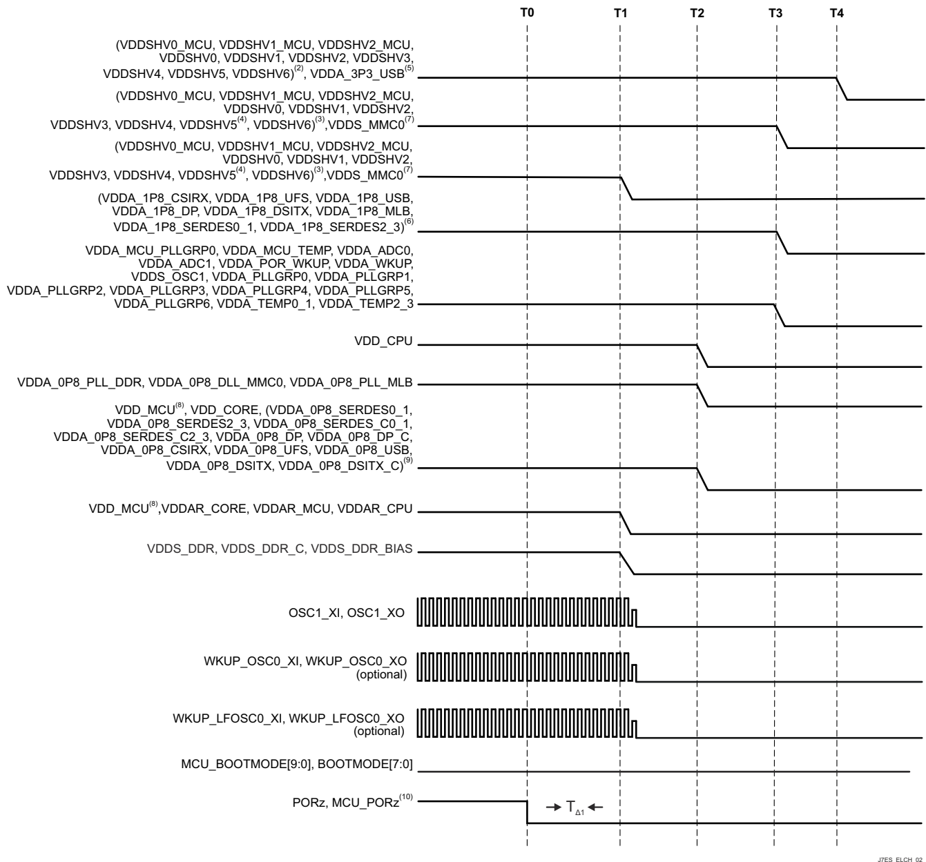
图 7-4. Combined MCU and Main Domains, Primary Power-Down Sequence
