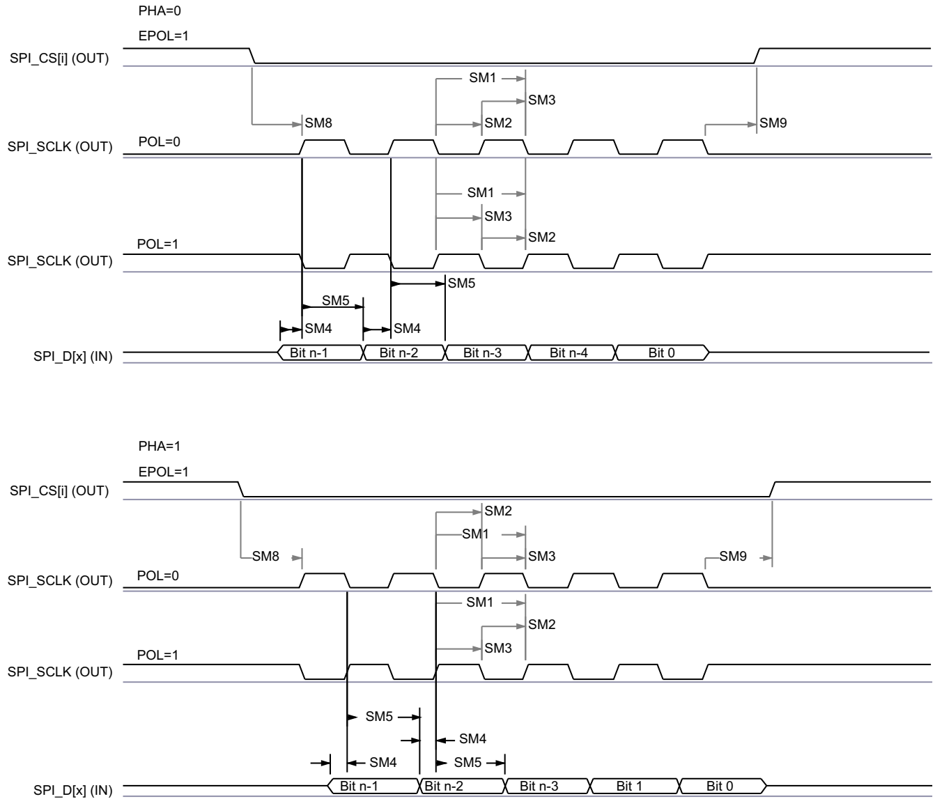
图 7-86. SPI Master Mode Receive Timing
