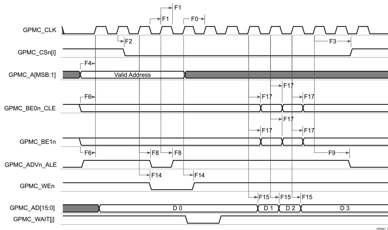
图 7-64. GPMC and NOR Flash — Synchronous Burst Read — 4x16 - bit (GPMCFCLKDIVIDER = 0)
