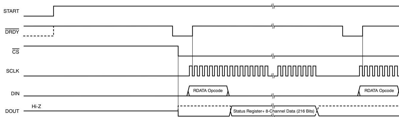
Figure 39. RDATA Usage
