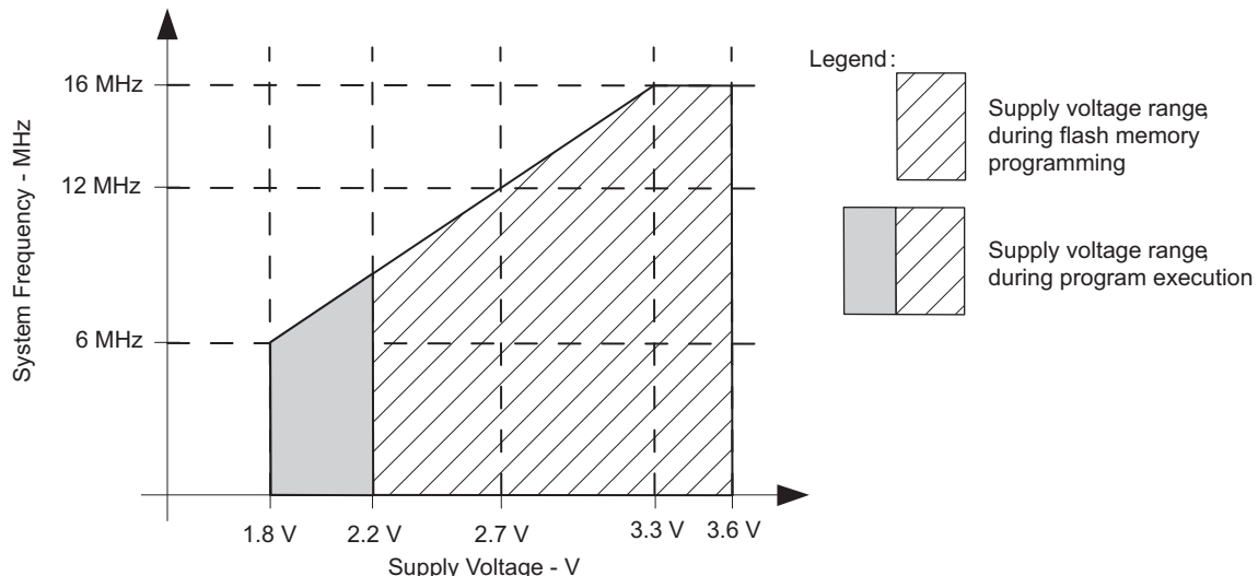
Figure 1. Safe Operating Area
