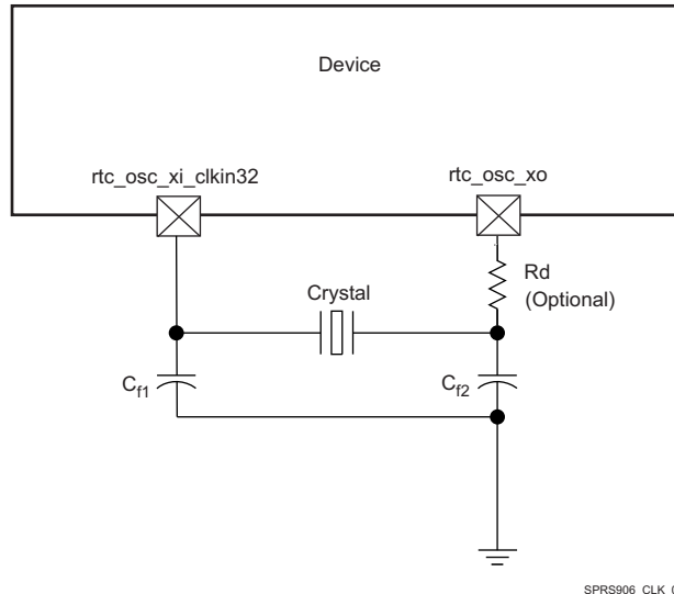
Figure 6-10. Crystal Implementation
