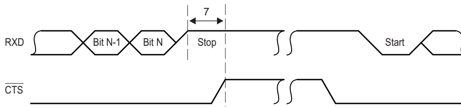
图 5-51. UART RTS (Request-to-Send Output) – Autoflow Timing Waveform
