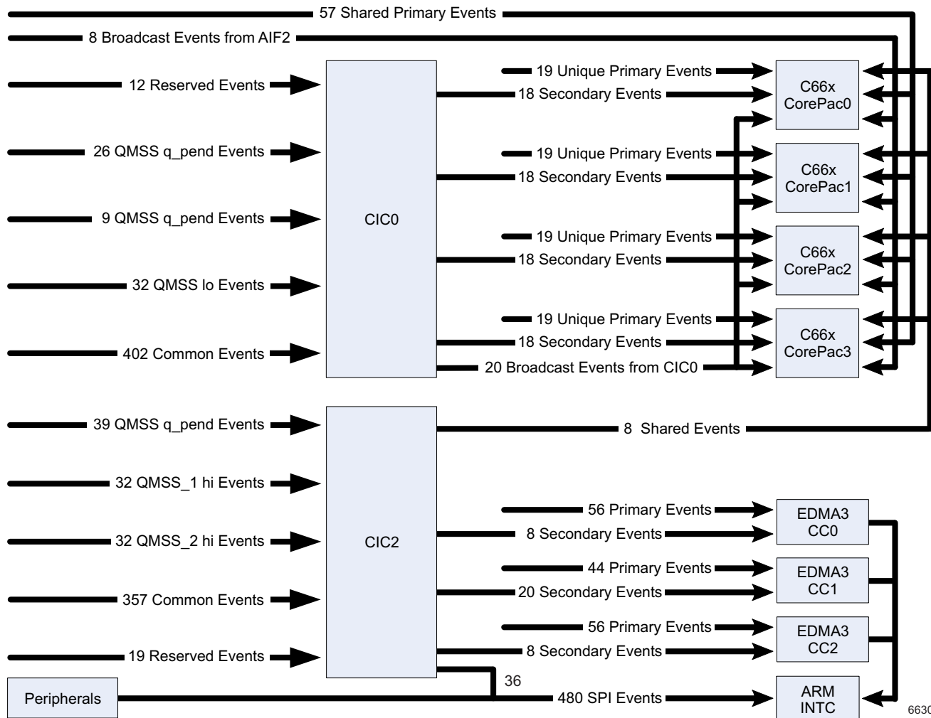
图 6-13. Interrupt Topology
