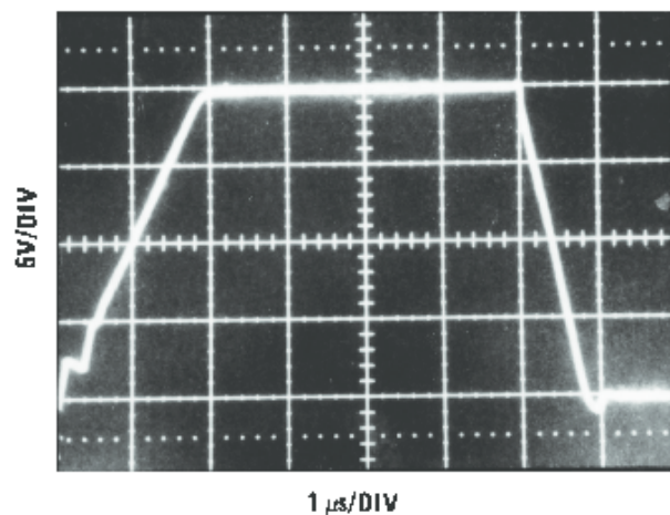
1 μs/DIV Figure 37. LF356
