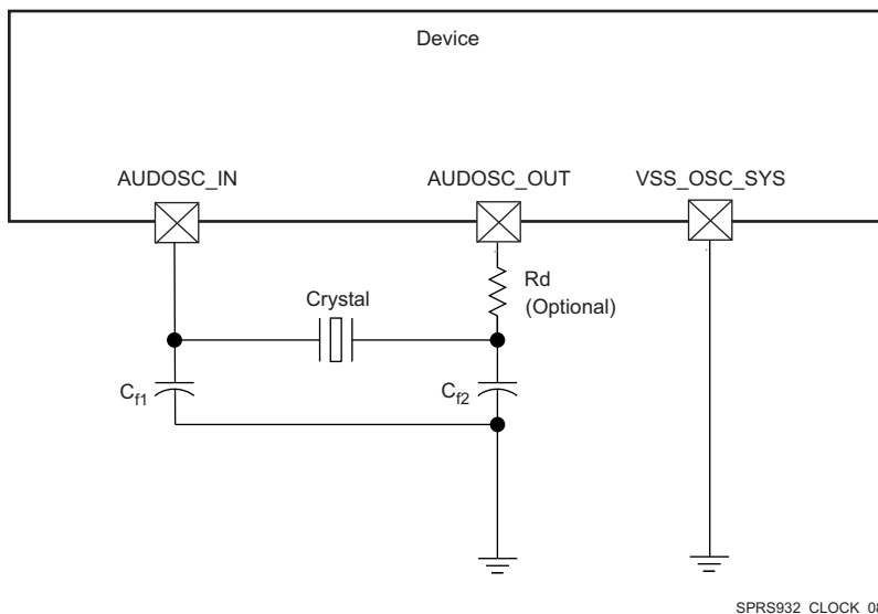
Figure 5-17. Crystal Implementation (1)
