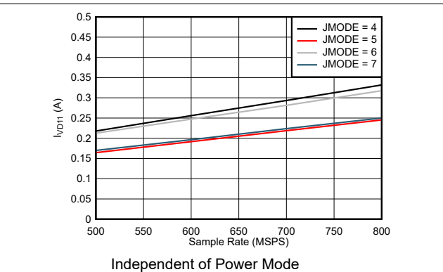
Figure 7-78. Quad Channel, I_{VD11} vs F_S for JMODES 4 - 7 Independent of Power Mode
