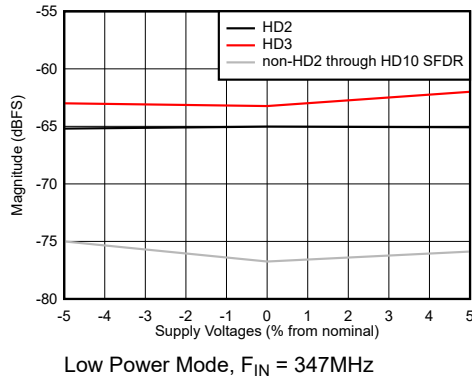
Low Power Mode, F_{IN} = 347 MHz Figure 7-49. HD2, HD3 and Worst non-HD2/3 Spur vs Supply Voltage
