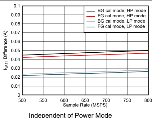
Figure 7-107. Quad Channel, I_{VA11} Change with Calibration Mode
