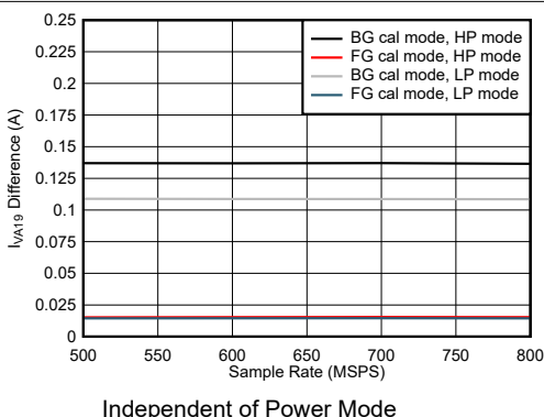
Figure 7-105. Dual Channel, I_{VA19} Change with Calibration Mode
