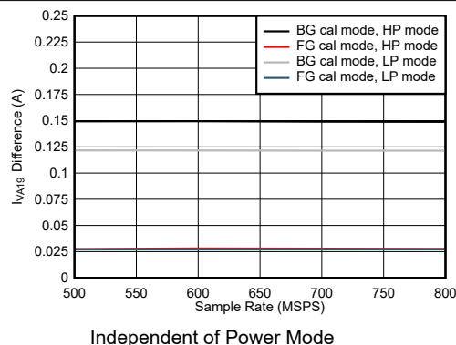
Figure 7-104. Quad Channel, I_{VA19} Change with Calibration Mode
