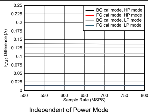
Figure 7-106. Single Channel, I_{VA19} Change with Calibration Mode
