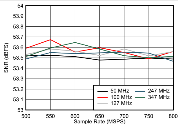
Figure 7-25. SNR vs Sample Rate
