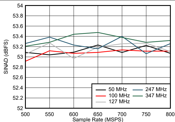
Figure 7-26. SINAD vs Sample Rate
