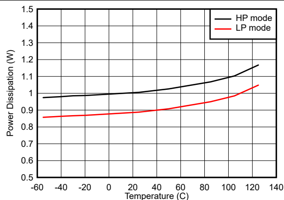
Independent of Power Mode Figure 7-115. Single Channel, Power Dissipation vs Temperature
