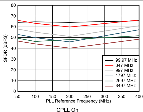
Figure 7-64. SFDR vs Reference Clock Frequency
