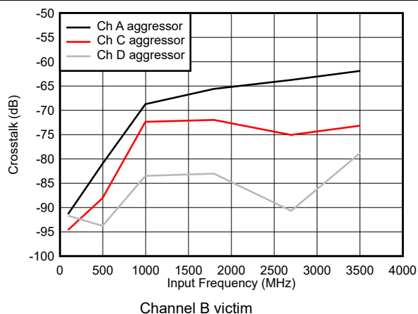
Figure 7-62. Crosstalk vs Input Frequency
