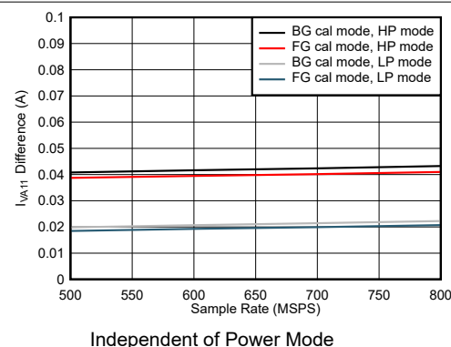
Figure 7-108. Dual Channel, I_{VA11} Change with Calibration Mode
