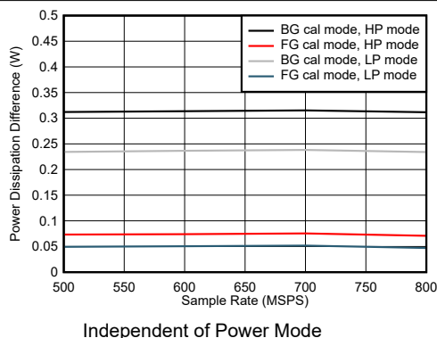
Figure 7-103. Single Channel, Power Dissipation Change with Calibration Mode
