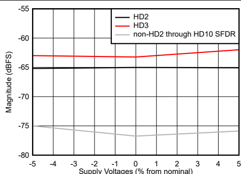
Figure 7-49. HD2, HD3 and Worst non-HD2/3 Spur vs Supply Voltage
