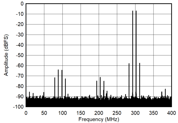
-7 dBFS each tone Figure 7-54. Single Tone FFT at 2698 MHz
