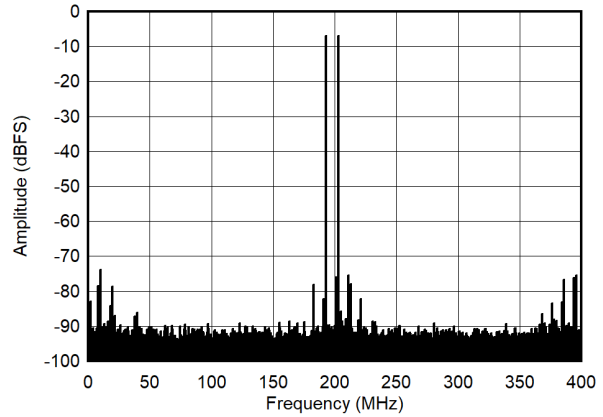
-7 dBFS each tone Figure 7-52. Single Tone FFT at 998 MHz
