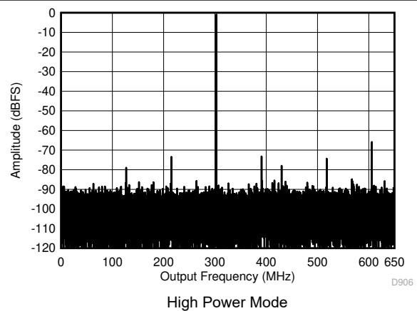
图 7-6. Single Tone FFT at 997 MHz and -1 dBFS
