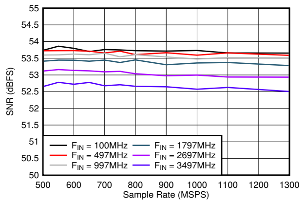
图 7-22. SNR vs Sample Rate
