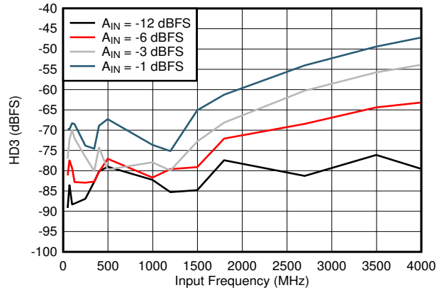
图 7-20. HD3 vs Input Frequency
