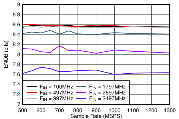
图 7-24. ENOB vs Sample Rate
