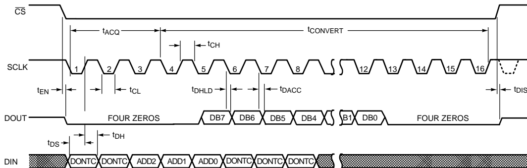
Figure 2. ADC088S052 Serial Timing Diagram
