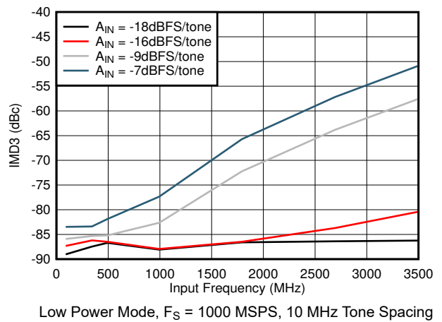
图 7-58. IMD3 vs Input Frequency
