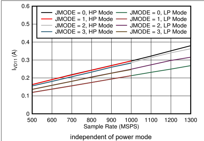
图 7-97. Dual Channel, I_{VD11} vs FS and JMODE 0 - 3
