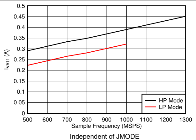
图 7-96. Dual Channel, I_{VA11} vs FS
