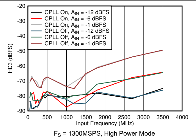
图 7-74. HD3 vs Input Frequency, CPLL and Input Amplitude
