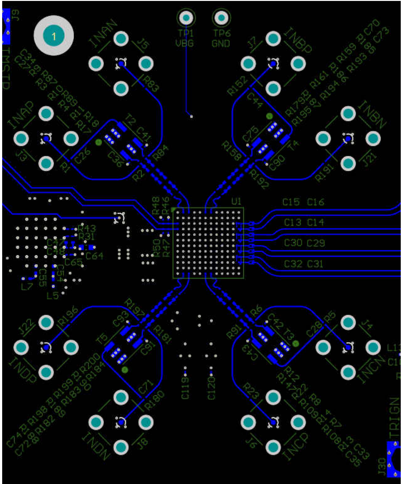
图 11-1. Top Layer Routing: Analog Inputs (INA ± , INB ± , INC ± , IND ± ), TM STP ± and D[3:0] ± Routing
