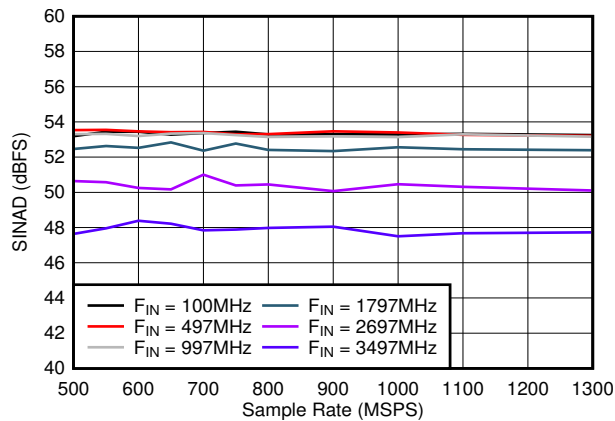
图 7-23. SINAD vs Sample Rate
