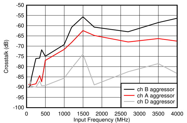
图 7-60. Crosstalk to Channel B vs F_{IN}
