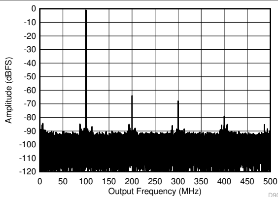
图 7-9. Single Tone FFT at 2697 MHz and -1 dBFS
