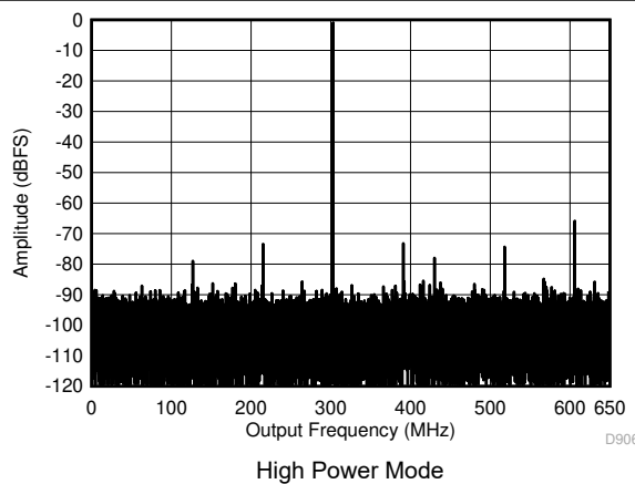
图 7-6. Single Tone FFT at 997 MHz and -1 dBFS
