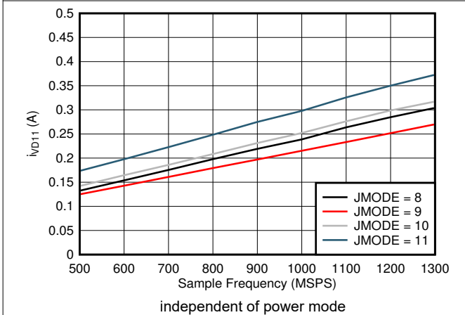
图 7-99. Dual Channel, I_{VD11} vs FS and JMODE 8 - 11
