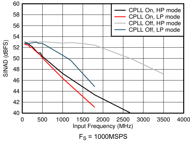
图 7-67. SINAD vs Input Frequency and CPLL
