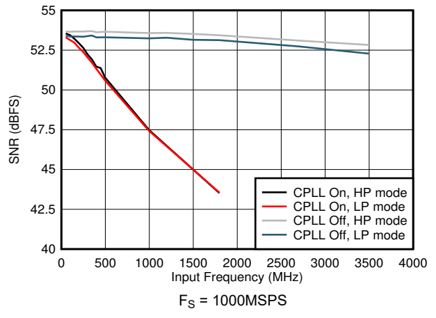
图 7-66. SNR vs Input Frequency and CPLL
