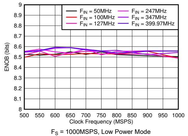
图 7-28. ENOB vs Sample Rate
