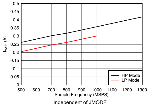
图 7-106. Single Channel, I_{VA11} vs FS
