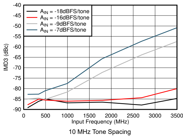
图 7-57. IMD3 vs Input Frequency
