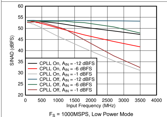
图 7-77. SINAD vs Input Frequency, CPLL and Input Amplitude
