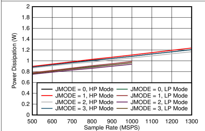
图 7-101. Single Channel, Power Dissipation vs FS for JMODES 0 - 3
