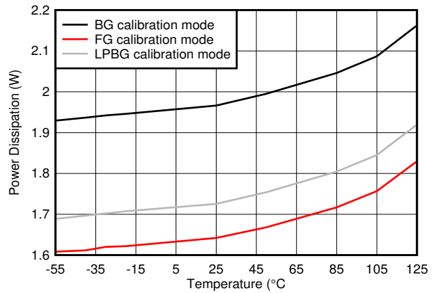
图 7-124. Dual Channel, Power Dissipation vs Temperature
