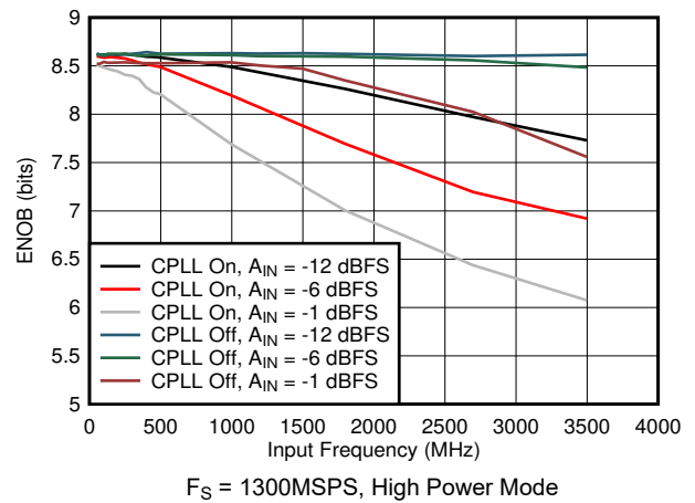
图 7-72. ENOB vs Input Frequency, CPLL and Input Amplitude
