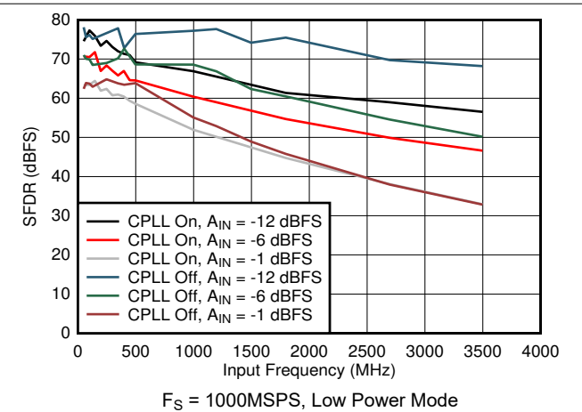
图 7-76. SFDR vs Input Frequency, CPLL and Input Amplitude
