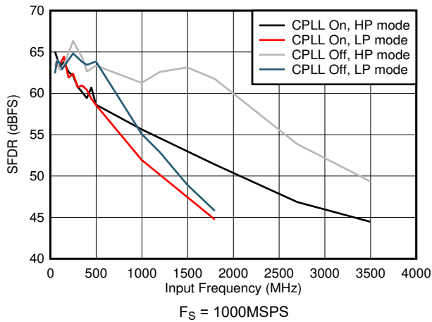
图 7-65. SFDR vs Input Frequency and CPLL
