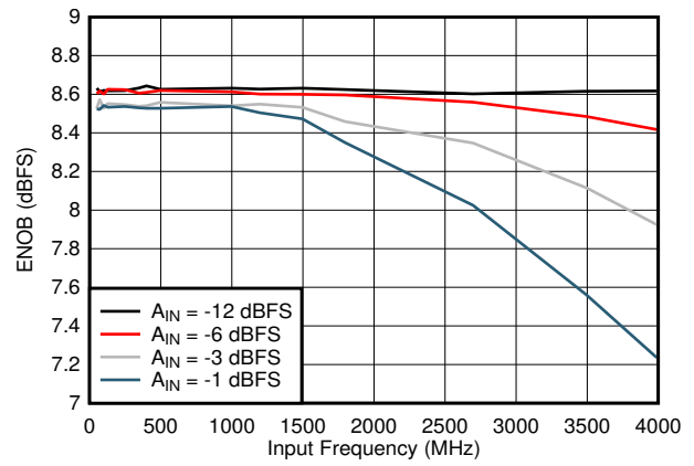
图 7-18. ENOB vs Input Frequency
