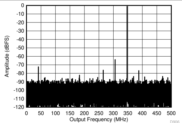
图 7-10. Single Tone FFT at 3497 MHz and -1 dBFS
