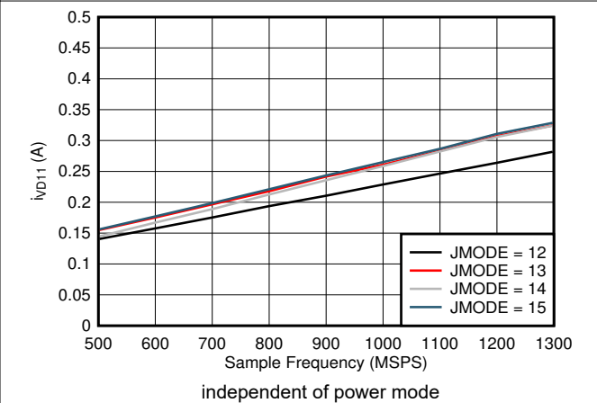
图 7-100. Dual Channel, I_{VD11} vs FS and JMODE 12 - 15
