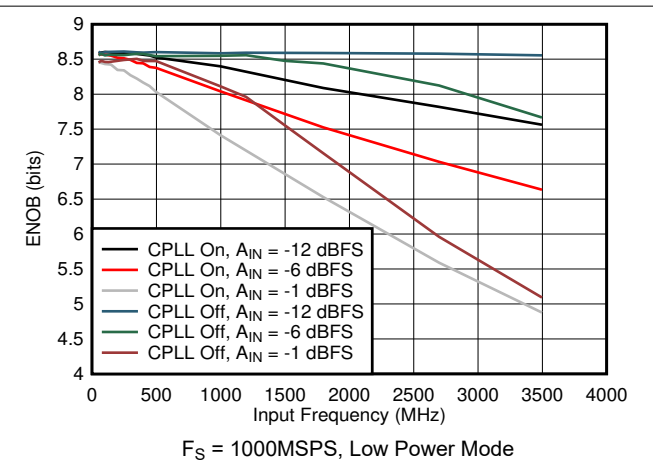
图 7-78. ENOB vs Input Frequency, CPLL and Input Amplitude
