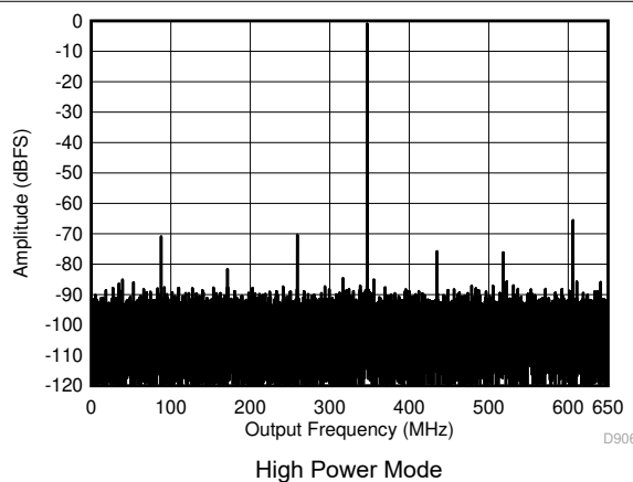
图 7-4. Single Tone FFT at 347 MHz and -1 dBFS
