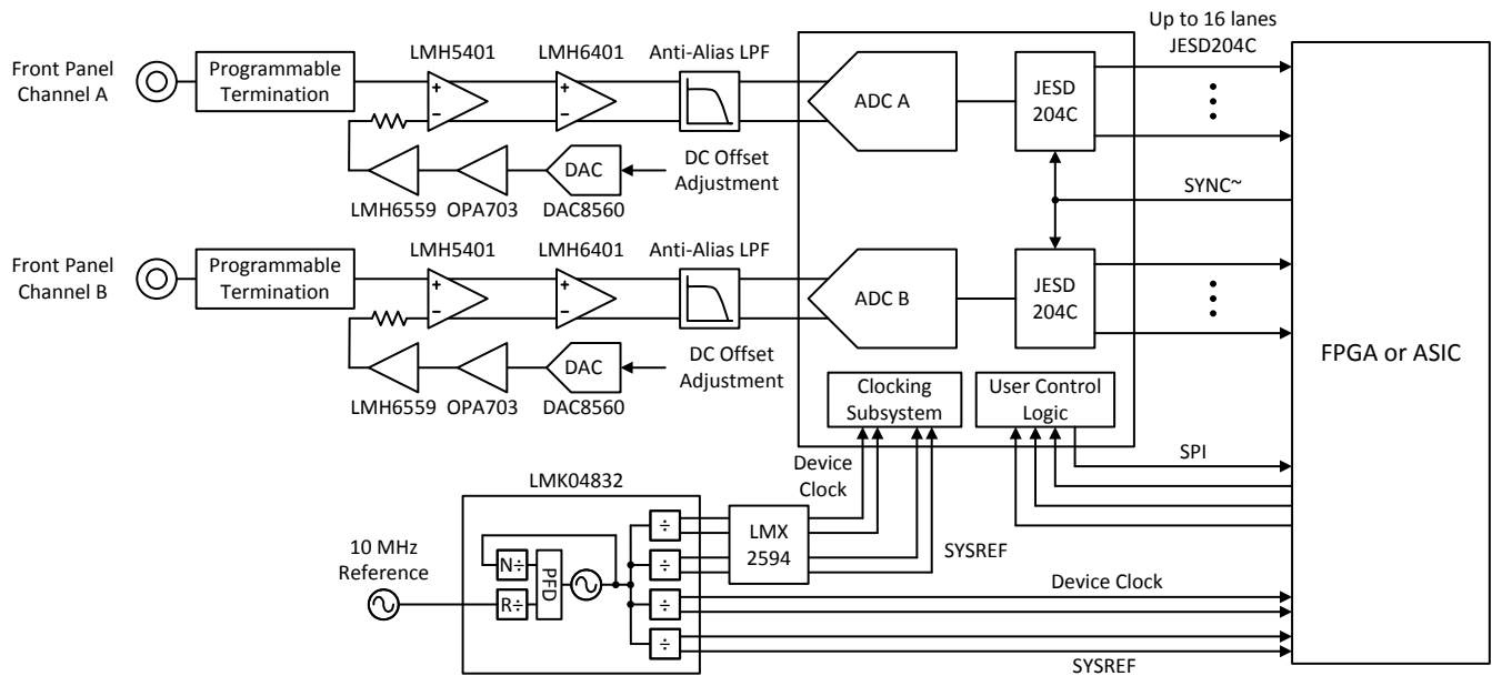
图 9-3. Typical Configuration for Reconfigurable Oscilloscope
