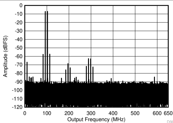
图 7-51. Two Tone FFT at 998 MHz Center
