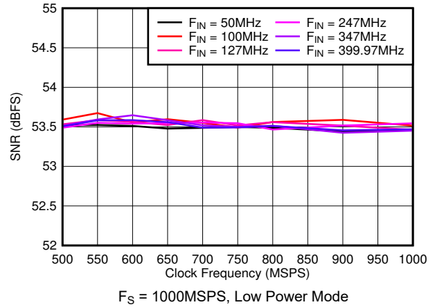
图 7-26. SNR vs Sample Rate
