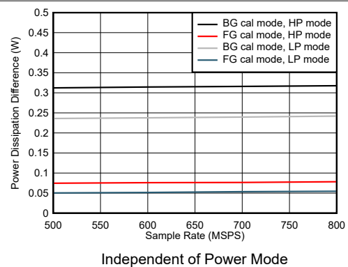
图 7-102. Dual Channel, Power Dissipation Change with Calibration Mode
