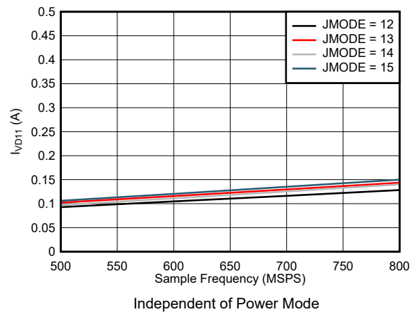
图 7-100. Single Channel, I_{VD11} vs F_S for JMODES 12 - 15
