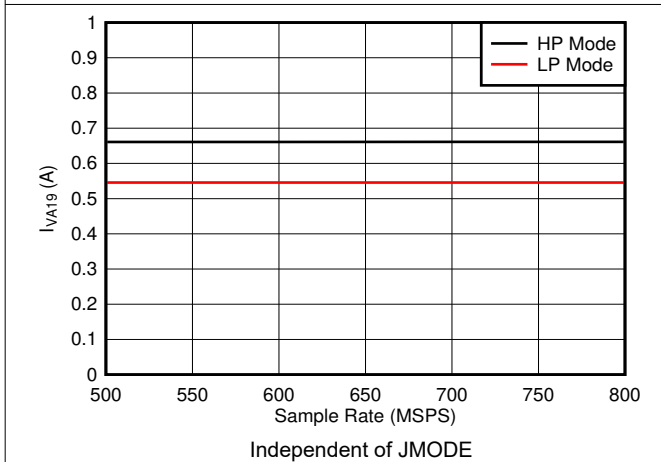
图 7-75. Quad Channel, I_{VA19} vs F_S
