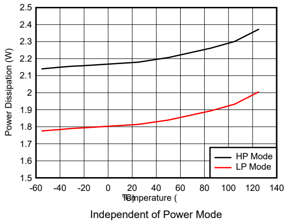
图 7-113. Quad Channel, Power Dissipation vs Temperature
