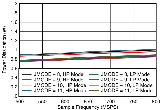
图 7-93. Single Channel, Power Dissipation vs F_S for JMODES 8 - 11
