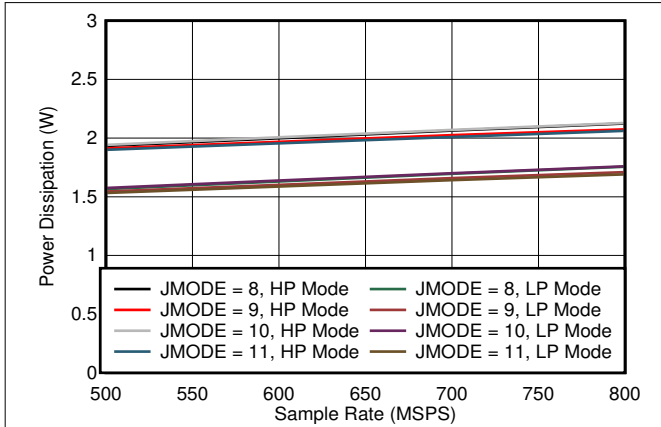
图 7-73. Quad Channel, Power Dissipation vs F_S for JMODES 8 - 11
