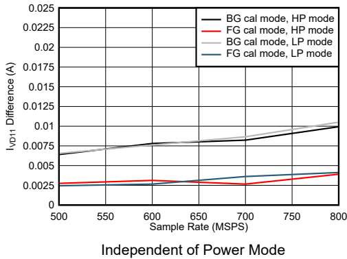
图 7-111. Dual Channel, I_{VD11} Change with Calibration Mode
