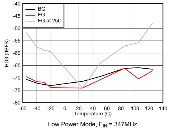
图 7-44. HD3 vs Temperature
