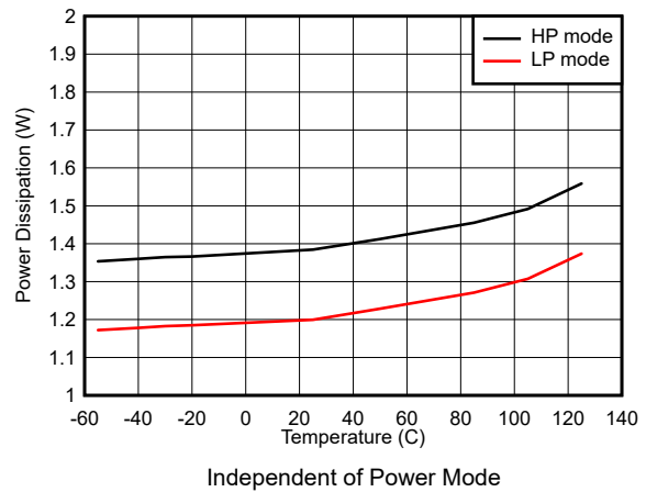
图 7-114. Dual Channel, Power Dissipation vs Temperature
