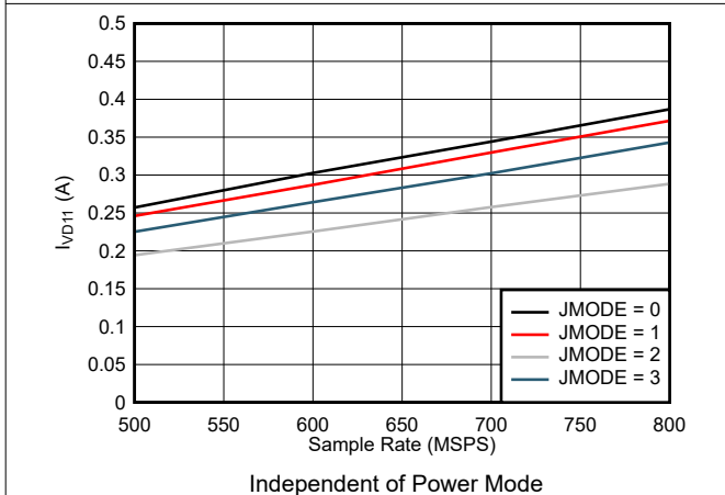
图 7-77. Quad Channel, I_{VD11} vs F_S for JMODES 0 - 3
