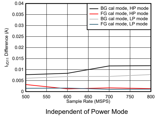
图 7-110. Quad Channel, I_{VD11} Change with Calibration Mode
