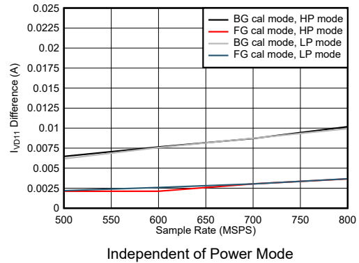
图 7-112. Single Channel, I_{VD11} Change with Calibration Mode
