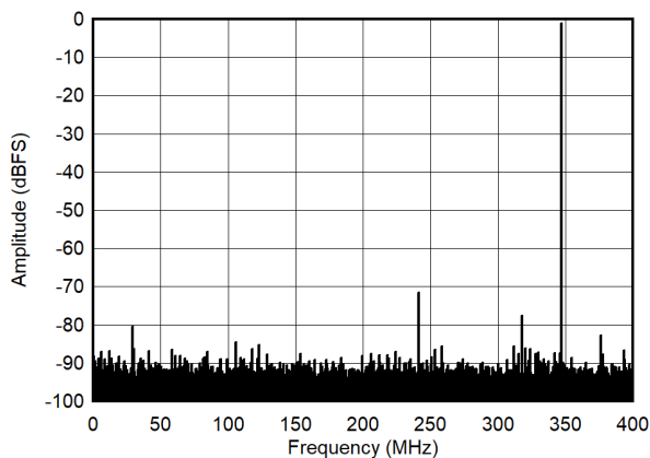
图 7-11. Single Tone FFT at 347MHz and -1dBFS
