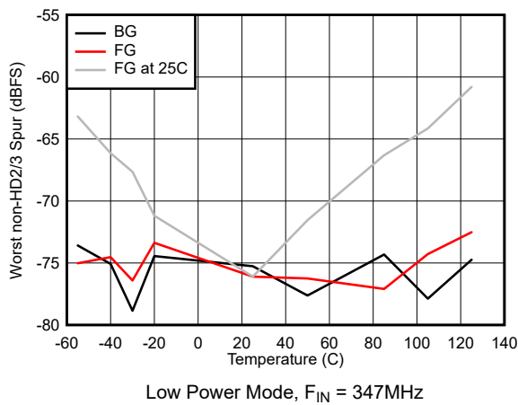
图 7-45. Worst non-HD2/3 Spur vs Temperature
