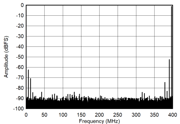
图 7-12. Single Tone FFT at 1197MHz and -1dBFS
