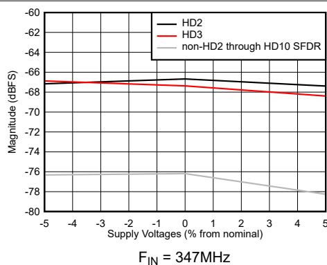
图 7-47. HD2, HD3 and Worst non-HD2/3 Spur vs Supply Voltage
