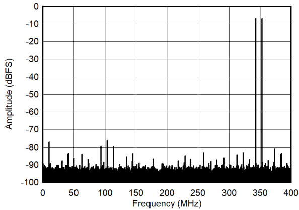
图 7-51. Dual Tone FFT at 348 MHz -7 dBFS each tone
