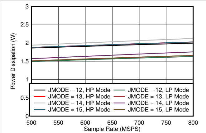
图 7-74. Quad Channel, Power Dissipation vs F_S for JMODES 12 - 15
