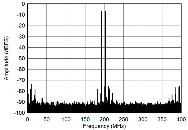
图 7-52. Dual Tone FFT at 998 MHz -7 dBFS each tone
