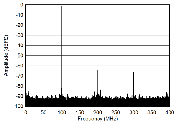
图 7-10. Single Tone FFT at 100MHz and -1dBFS
