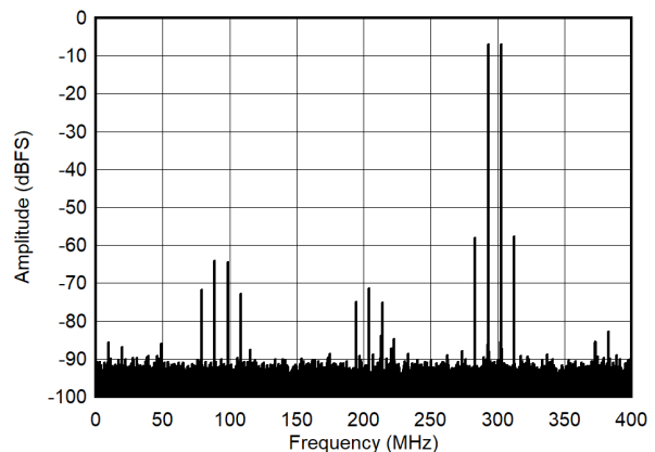
图 7-54. Dual Tone FFT at 2698 MHz -7 dBFS each tone
