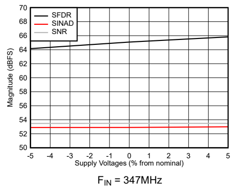
图 7-46. SNR, SFDR and SINAD vs Supply Voltage
