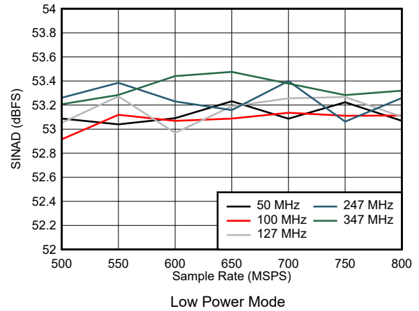
图 7-26. SINAD vs Sample Rate
