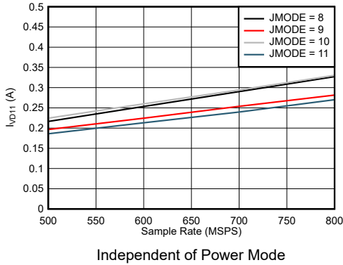
图 7-79. Quad Channel, I_{VD11} vs F_S for JMODES 8 - 11
