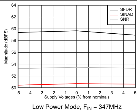
图 7-48. SNR, SFDR and SINAD vs Supply Voltage
