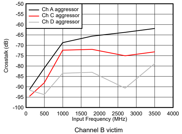
图 7-62. Crosstalk vs Input Frequency
