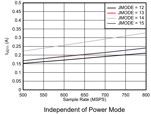
图 7-80. Quad Channel, I_{VD11} vs F_S for JMODES 12 - 15
