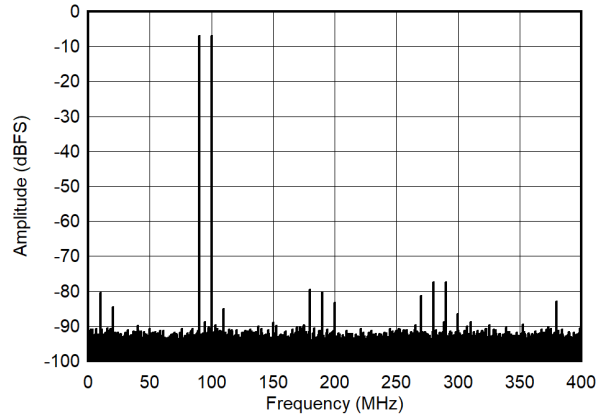
图 7-50. Dual Tone FFT at 95 MHz -7 dBFS each tone
