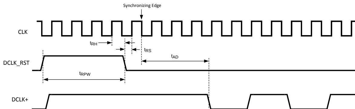
Figure 8. Clock Reset Timing in DDR Mode
