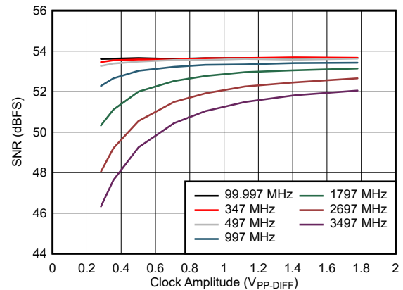
图 7-32. SNR vs Clock Amplitude
