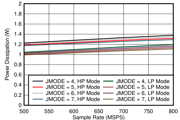
图 7-82. Dual Channel, Power Dissipation vs F_S for JMODES 4 - 7
