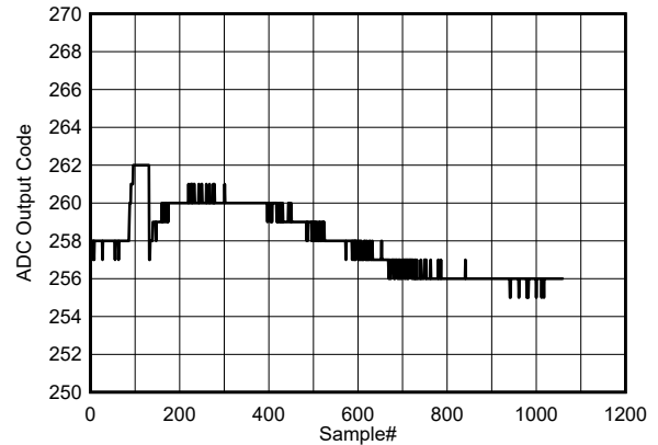
图 7-116. Background Core Transition (DC midscale input)
