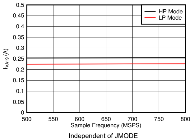
图 7-95. Single Channel, I_{VA19} vs F_S
