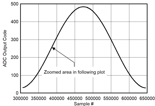
图 7-117. Background Core Transition (AC Signal)
