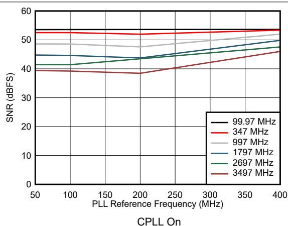
图 7-63. SNR vs Reference Clock Frequency
