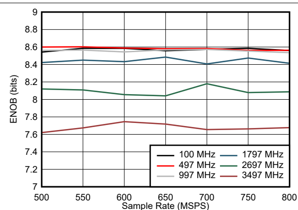
图 7-23. ENOB vs Sample Rate
