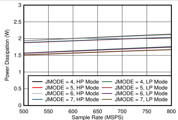
图 7-72. Quad Channel, Power Dissipation vs F_S for JMODES 4 - 7
