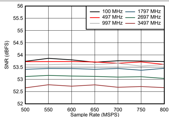
图 7-21. SNR vs Sample Rate
