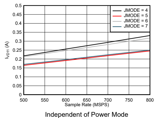
图 7-78. Quad Channel, I_{VD11} vs F_S for JMODES 4 - 7
