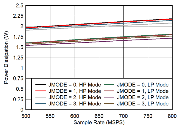
图 7-71. Quad Channel, Power Dissipation vs F_S for JMODES 0 - 3
