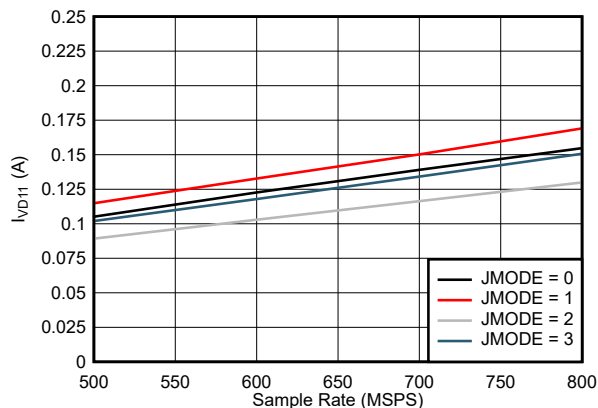
图 7-97. Single Channel, I_{VD11} vs F_S for JMODES 0 - 3
