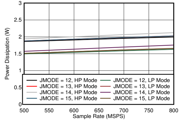
图 7-74. Quad Channel, Power Dissipation vs F_S for JMODES 12 - 15
