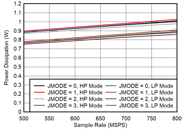
图 7-91. Single Channel, Power Dissipation vs F_S for JMODES 0 - 3
