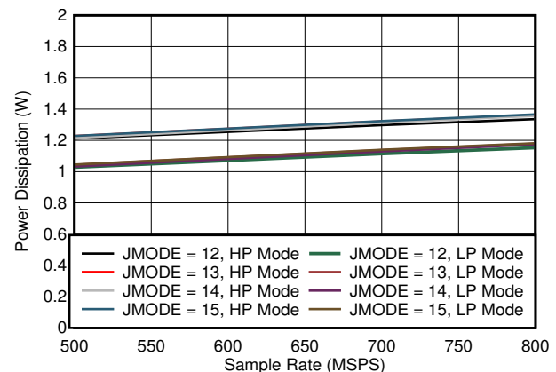
图 7-84. Dual Channel, Power Dissipation vs F_S for JMODES 12 - 15
