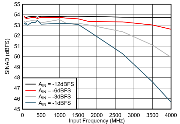
图 7-16. SINAD vs Input Frequency
