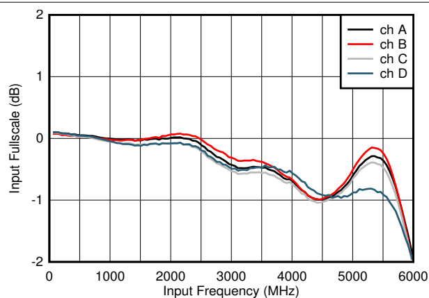
图 7-3. Input Fullscale vs Input Frequency
