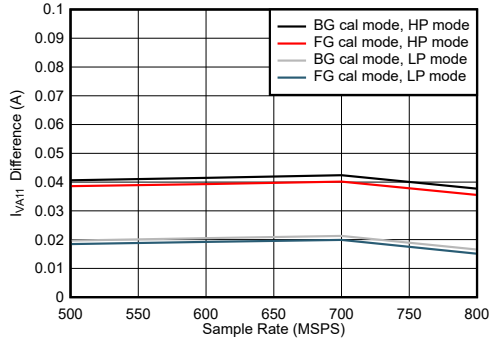
图 7-109. Single Channel, I_{VA11} Change with Calibration Mode
