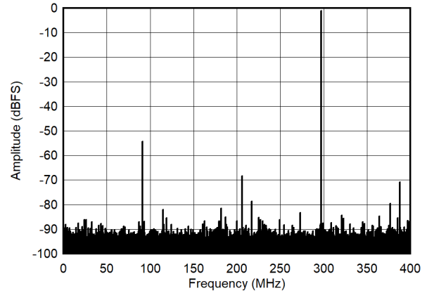
图 7-8. Single Tone FFT at 2697 MHz and -1dBFS
