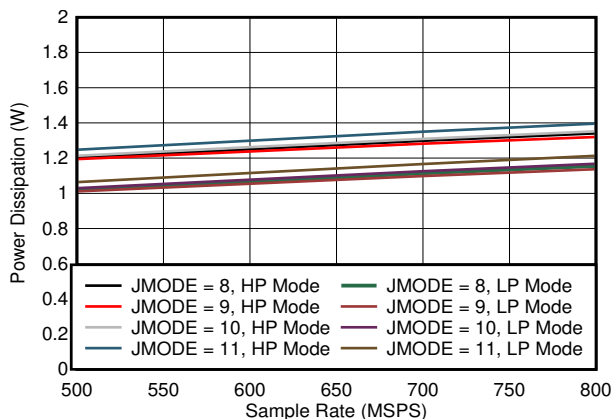
图 7-83. Dual Channel, Power Dissipation vs F_S for JMODES 8 - 11
