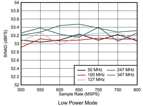
图 7-26. SINAD vs Sample Rate
