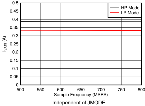
图 7-85. Dual Channel, I_{VA19} vs F_S
