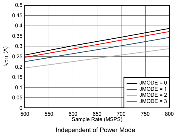
图 7-77. Quad Channel, I_{VD11} vs F_S for JMODES 0 - 3
