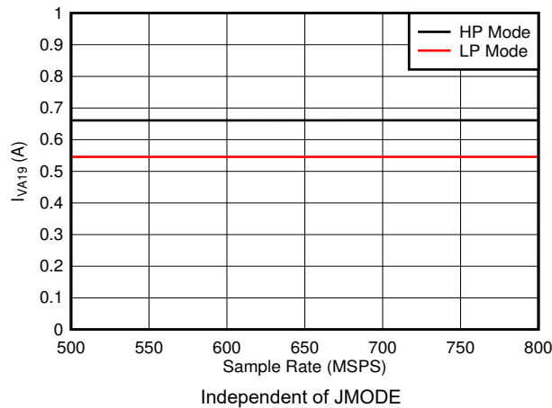
图 7-75. Quad Channel, I_{VA19} vs F_S
