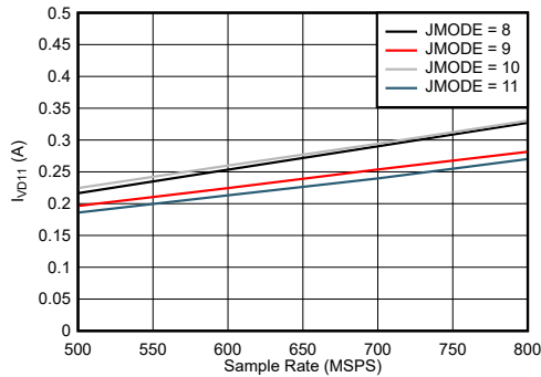
图 7-79. Quad Channel, I_{VD11} vs F_S for JMODES 8 - 11
