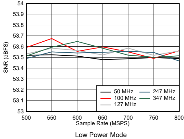
图 7-25. SNR vs Sample Rate
