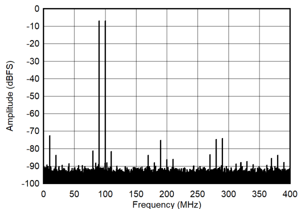
图 7-56. Dual Tone FFT at 95 MHz (LP Mode)
