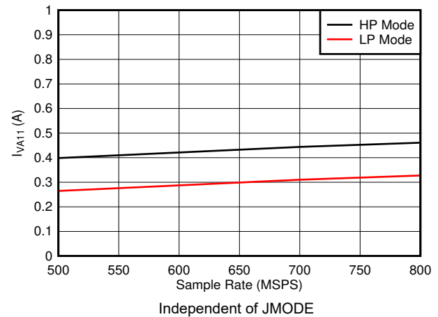
图 7-76. Quad Channel, I_{VA11} vs F_S
