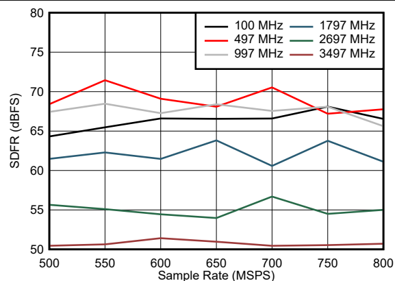
图 7-20. SFDR vs Sample Rate
