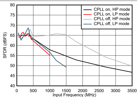
图 7-65. SFDR vs Input Frequency and CPLL and Power Mode
