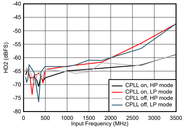
图 7-69. HD2 vs Input Frequency and CPLL and Power Mode
