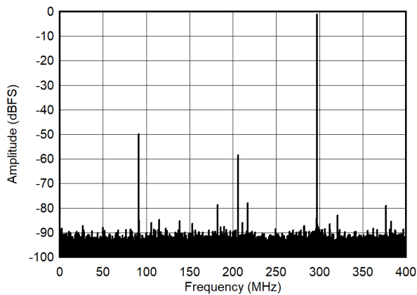
图 7-9. Single Tone FFT at 3497 MHz and -1dBFS
