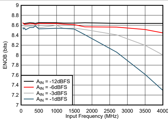
图 7-17. ENOB vs Input Frequency
