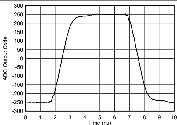
图 9-2. Measured Pulse using Sub-Sampling Technique for Equivalent 25.6 GSPS Measurement
