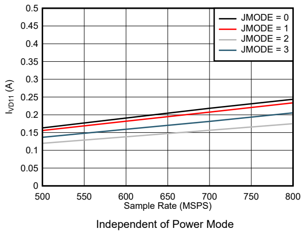
图 7-87. Dual Channel, I_{VD11} vs F_S for JMODES 0 - 3
