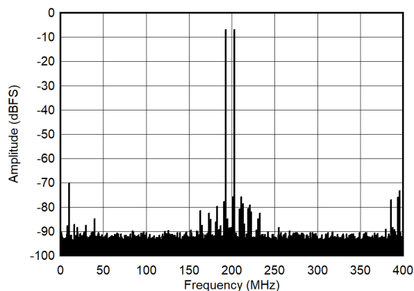
图 7-58. Dual Tone FFT at 998 MHz (LP Mode)
