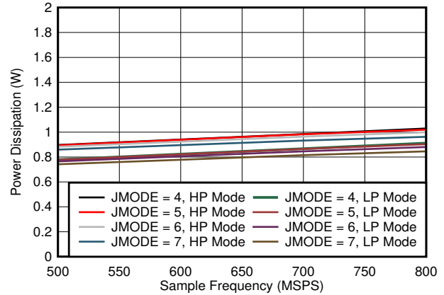
图 7-92. Single Channel, Power Dissipation vs F_S for JMODES 4 - 7
