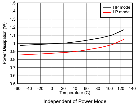
图 7-115. Single Channel, Power Dissipation vs Temperature
