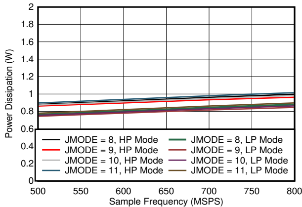
图 7-93. Single Channel, Power Dissipation vs F_S for JMODES 8 - 11
