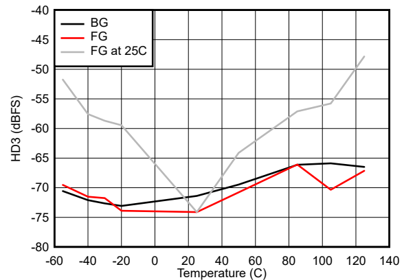
图 7-44. HD3 vs Temperature
