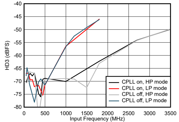
图 7-70. HD3 vs Input Frequency and CPLL and Power Mode
