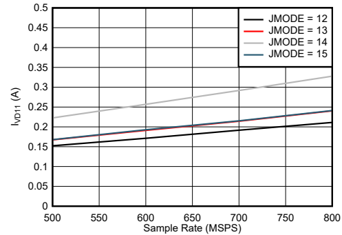
图 7-80. Quad Channel, I_{VD11} vs F_S for JMODES 12 - 15
