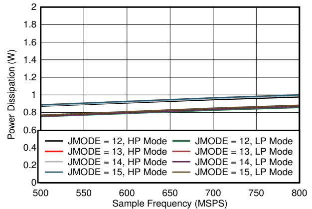
图 7-94. Single Channel, Power Dissipation vs F_S for JMODES 12 - 15
