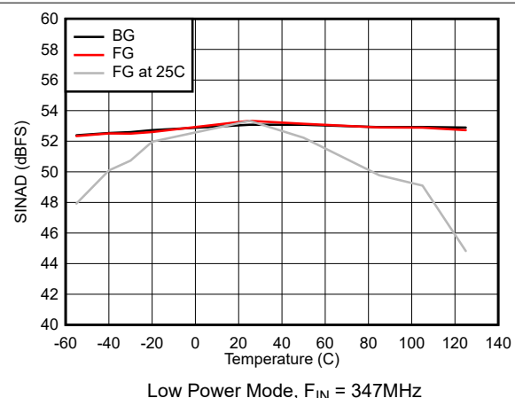
图 7-42. SINAD vs Temperature
