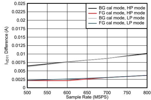
图 7-110. Quad Channel, I_{VD11} Change with Calibration Mode
