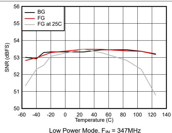
图 7-40. SNR vs Temperature
