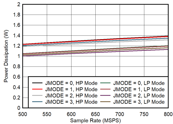
图 7-81. Dual Channel, Power Dissipation vs F_S for JMODES 0 - 3
