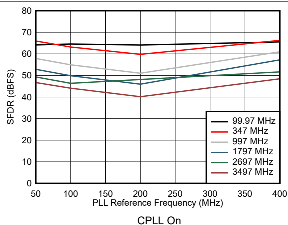
图 7-64. SFDR vs Reference Clock Frequency
