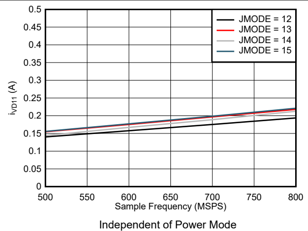
图 7-90. Dual Channel, I_{VD11} vs F_S for JMODES 12 - 15
