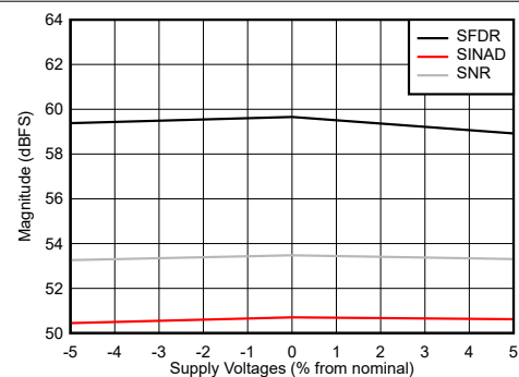
图 7-48. SNR, SFDR and SINAD vs Supply Voltage
