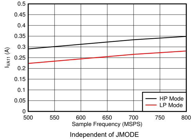
图 7-86. Dual Channel, I_{VA11} vs F_S
