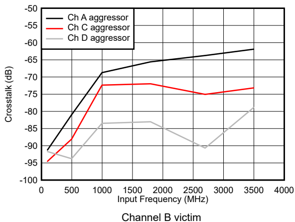
图 7-62. Crosstalk vs Input Frequency
