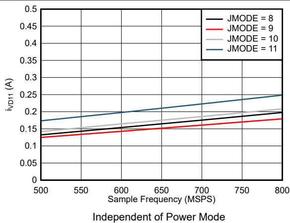
图 7-89. Dual Channel, I_{VD11} vs F_S for JMODES 8 - 11
