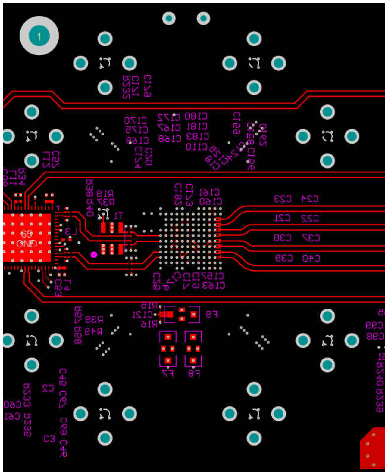
图 11-3. Bottom Layer Routing: CLK±, SYSREF and D[7:4]± Routing
