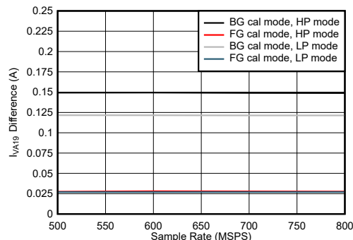
图 7-104. Quad Channel, I_{VA19} Change with Calibration Mode
