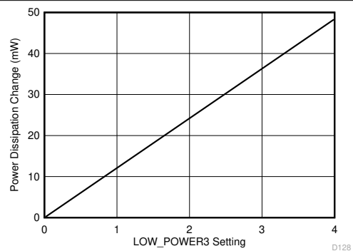
图 8-13. Power Dissipation Change vs LOW_POWER3 register setting
