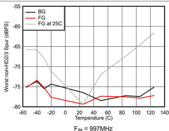
图 7-39. Worst non-HD2/3 Spur vs Temperature
