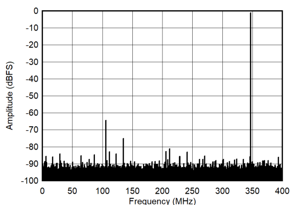
图 7-4. Single Tone FFT at 347 MHz and -1dBFS
