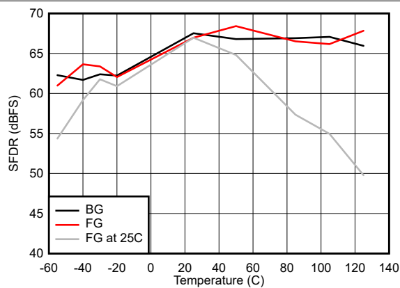
图 7-35. SFDR vs Temperature
