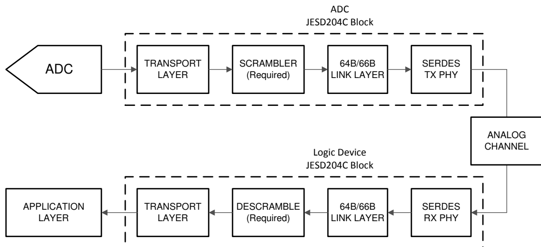
图 8-8. Simplified 64B/66B Encoded JESD204C Interface Diagram
