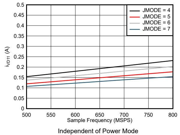
图 7-88. Dual Channel, I_{VD11} vs F_S for JMODES 4 - 7
