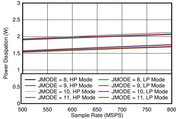
图 7-73. Quad Channel, Power Dissipation vs F_S for JMODES 8 - 11
