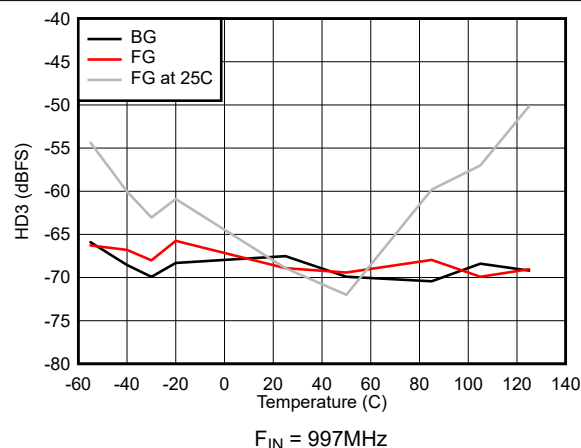
图 7-38. HD3 vs Temperature
