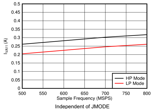
图 7-96. Single Channel, I_{VA11} vs F_S
