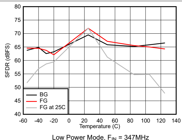
图 7-41. SFDR vs Temperature
