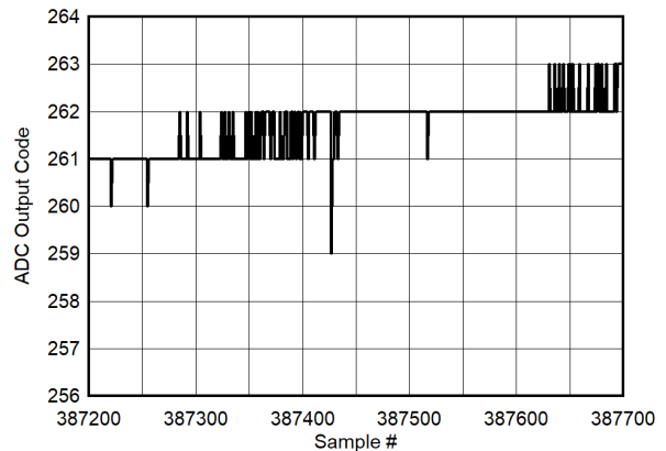
图 7-118. Background Core Transition (AC Signal Zoomed)
