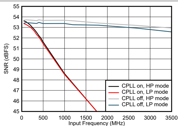
图 7-66. SNR vs Input Frequency and CPLL and Power Mode
