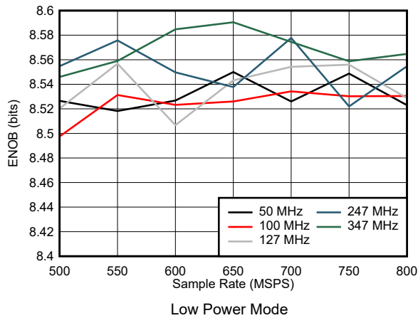
图 7-27. ENOB vs Sample Rate
