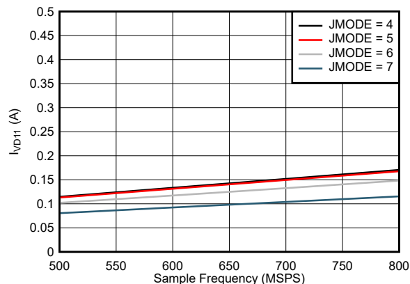
图 7-98. Single Channel, I_{VD11} vs F_S for JMODES 4 - 7
