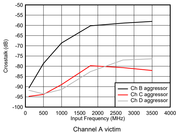
图 7-61. Crosstalk vs Input Frequency
