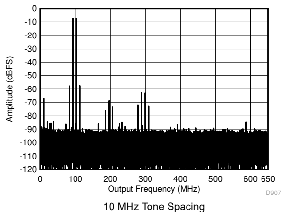
图 7-53. Two Tone FFT at 2698 MHz Center
