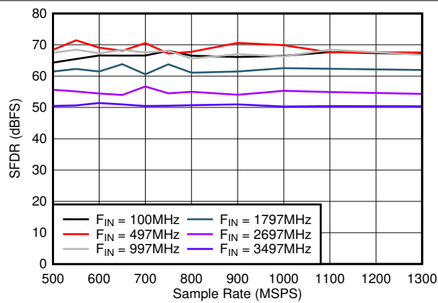
图 7-21. SFDR vs Sample Rate
