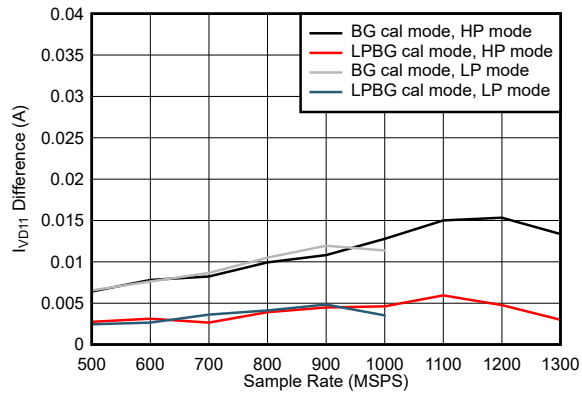
图 7-121. Dual Channel, I_{VD11} Change with Calibration Mode
