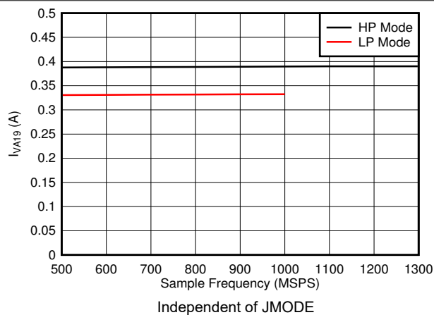
图 7-95. Dual Channel, I_{VA19} vs FS
