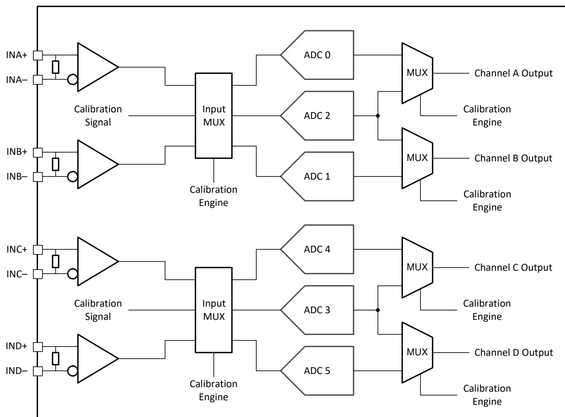
图 8-15. Quad Channel Calibration System Block Diagram
