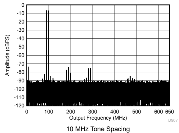
图 7-48. Two Tone FFT at 95.07 MHz Center
