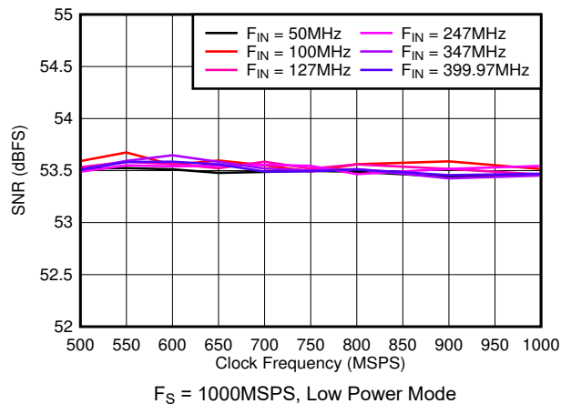
图 7-26. SNR vs Sample Rate
