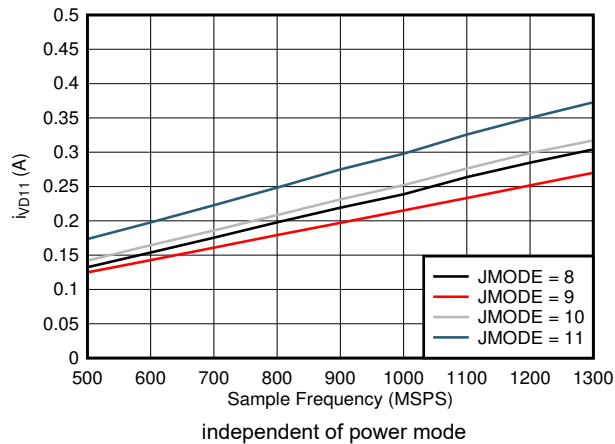
图 7-99. Dual Channel, I_{VD11} vs FS and JMODE 8 - 11
