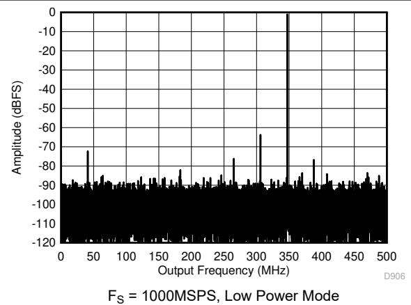
图 7-12. Single Tone FFT at 347 MHz and -1 dBFS
