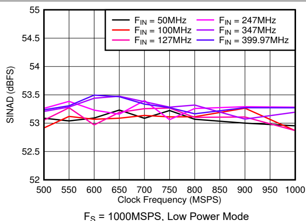
图 7-27. SINAD vs Sample Rate
