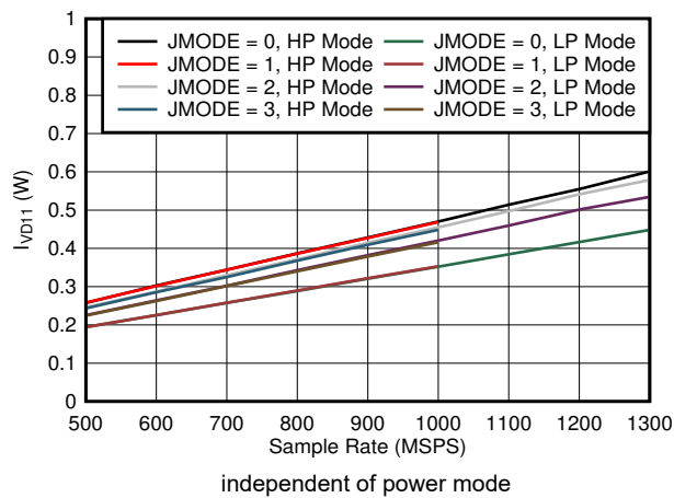
图 7-87. Quad Channel, I_{VD11} vs FS and JMODE 0 - 3
