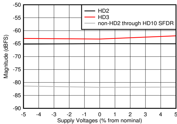
图 7-45. HD2, HD3 and Worst non-HD Spur vs Supply Voltage
