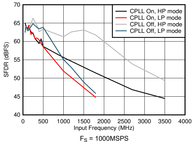
图 7-65. SFDR vs Input Frequency and CPLL
