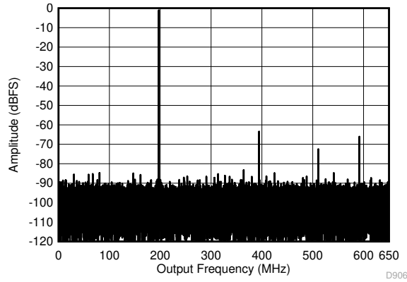
图 7-7. Single Tone FFT at 1497 MHz and -1 dBFS
