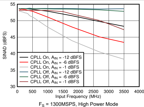
图 7-71. SINAD vs Input Frequency, CPLL and Input Amplitude
