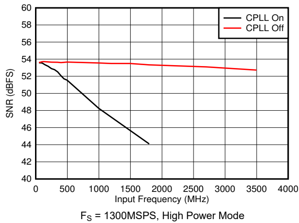
图 7-63. SNR vs Input Frequency and CPLL
