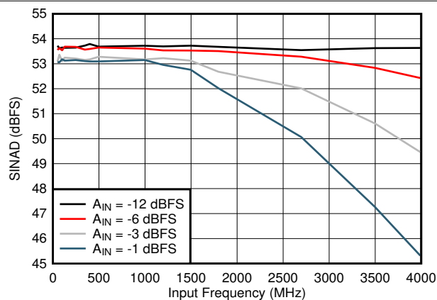
图 7-17. SINAD vs Input Frequency
