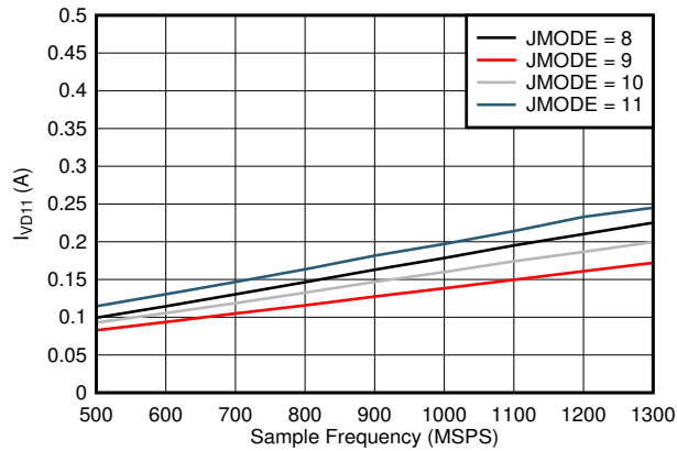
图 7-109. Single Channel, I_{VD11} vs FS and JMODE 8 - 11
