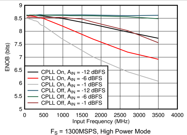
图 7-72. ENOB vs Input Frequency, CPLL and Input Amplitude
