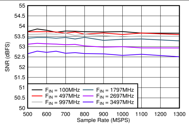
图 7-22. SNR vs Sample Rate
