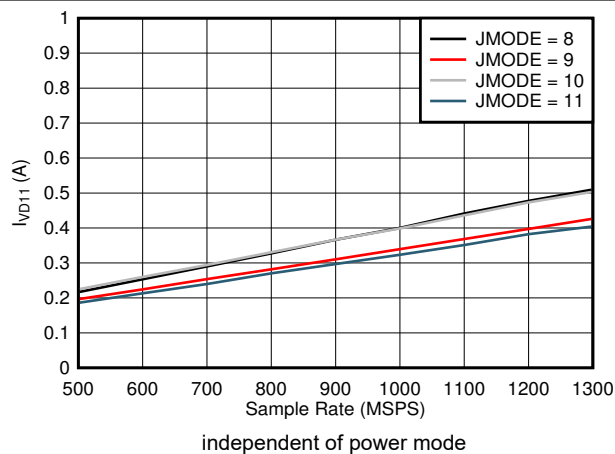
图 7-89. Quad Channel, I_{VD11} vs FS and JMODE 8 - 11
