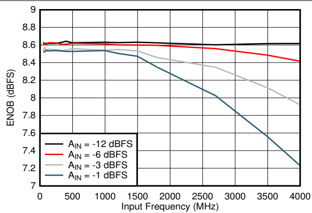
图 7-18. ENOB vs Input Frequency
