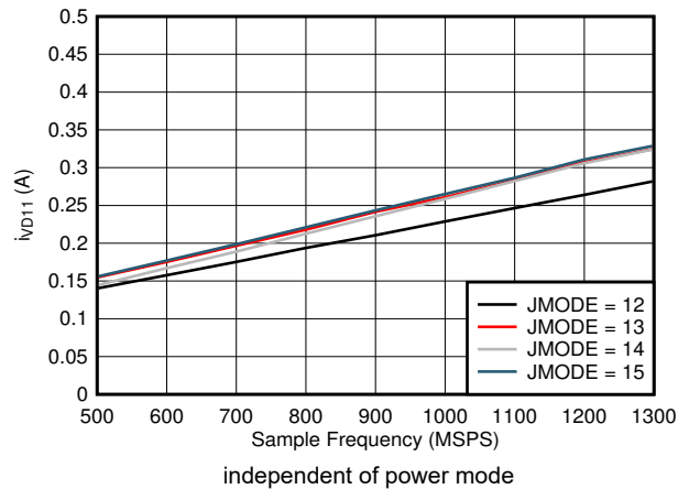
图 7-100. Dual Channel, I_{VD11} vs FS and JMODE 12 - 15
