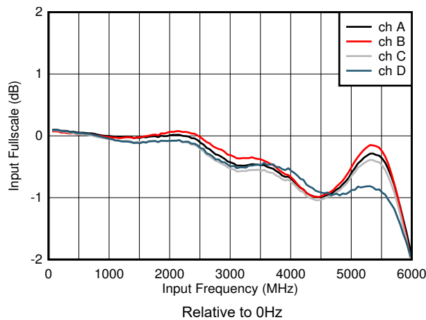
图 7-3. Input Fullscale vs Input Frequency
