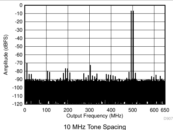
图 7-50. Two Tone FFT at 498 MHz Center
