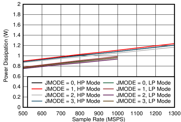
图 7-101. Single Channel, Power Dissipation vs FS for JMODES 0 - 3
