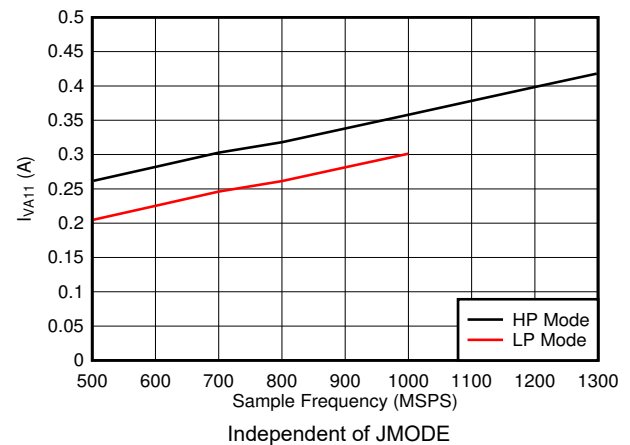
图 7-106. Single Channel, I_{VA11} vs FS
