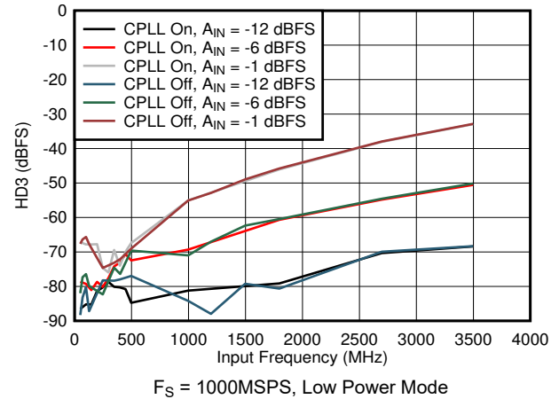
图 7-80. HD3 vs Input Frequency, CPLL and Input Amplitude
