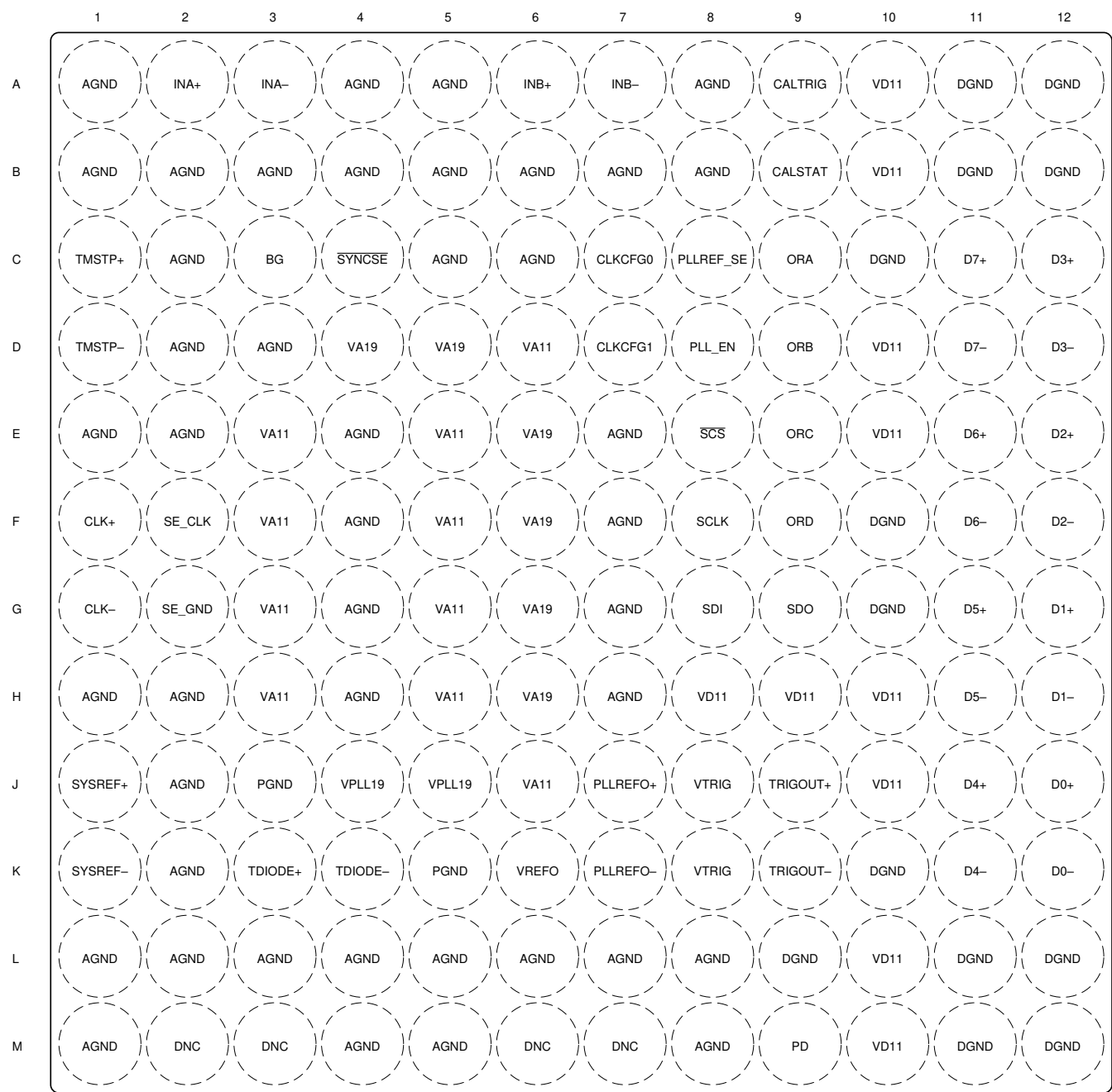
图 6-2. Dual Channel AAV Package, 144-Ball Flip Chip BGA (Top View)
