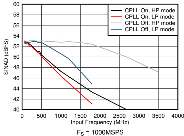
图 7-67. SINAD vs Input Frequency and CPLL
