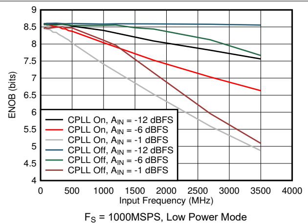
图 7-78. ENOB vs Input Frequency, CPLL and Input Amplitude
