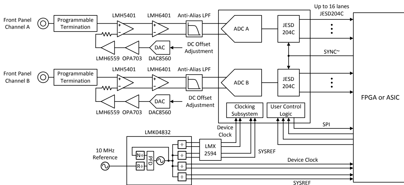
图 9-3. Typical Configuration for Reconfigurable Oscilloscope
