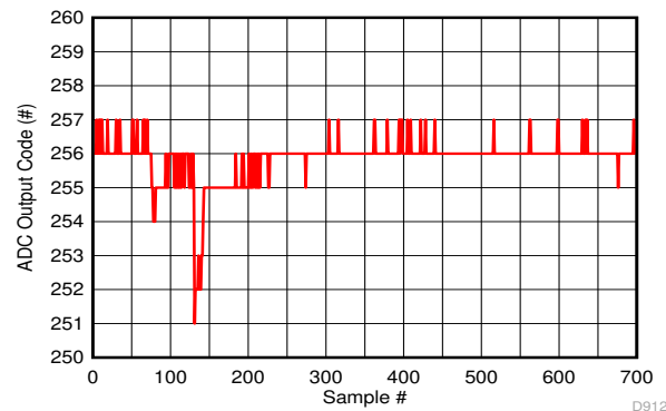
图 7-126. Background Calibration Core Transition (midscale voltage)
