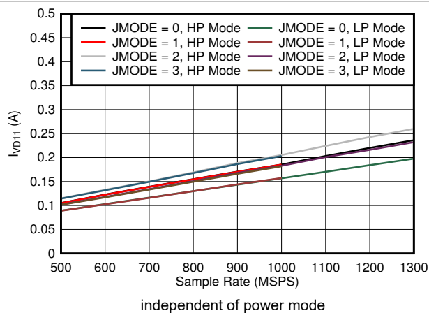
图 7-107. Single Channel, I_{VD11} vs FS and JMODE 0 - 3
