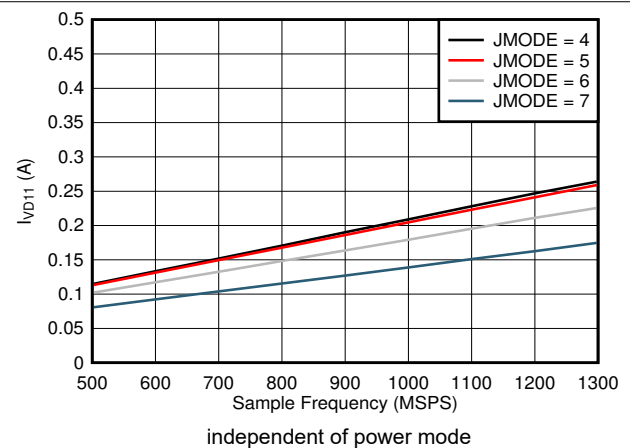
图 7-108. Single Channel, I_{VD11} vs FS and JMODE 4 - 7
