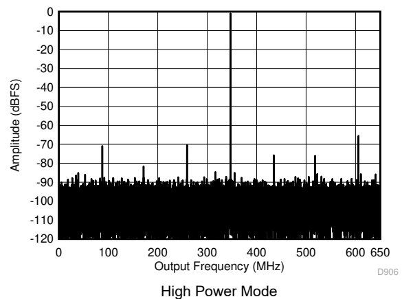
图 7-4. Single Tone FFT at 347 MHz and -1 dBFS
