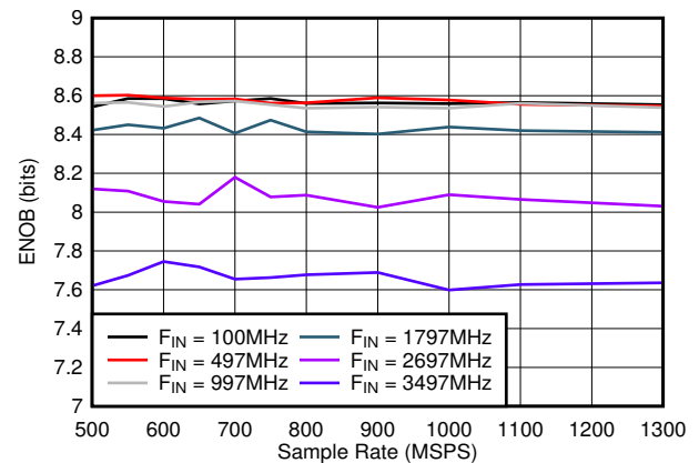
图 7-24. ENOB vs Sample Rate
