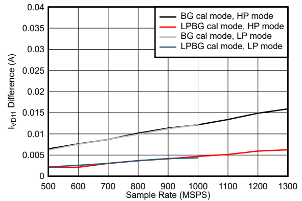
图 7-122. Dual Channel, I_{VD11} Change with Calibration Mode
