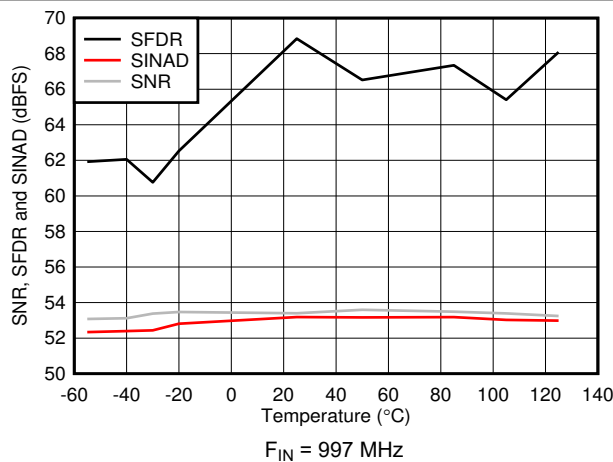
图 7-35. SNR, SFDR and SINAD vs Temperature
