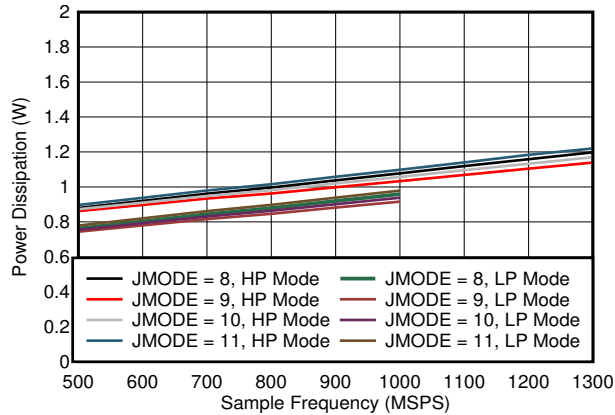
图 7-103. Single Channel, Power Dissipation vs FS for JMODES 8 - 11
