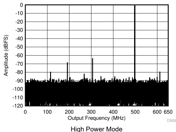
图 7-5. Single Tone FFT at 497 MHz and -1 dBFS
