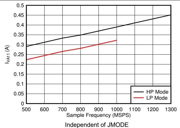
图 7-96. Dual Channel, I_{VA11} vs FS
