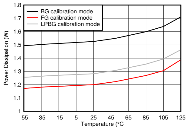
图 7-125. Single Channel, Power Dissipation vs Temperature
