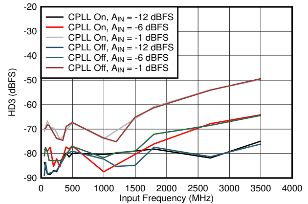
图 7-74. HD3 vs Input Frequency, CPLL and Input Amplitude
