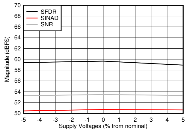
图 7-46. SNR, SFDR and SINAD vs Supply Voltage
