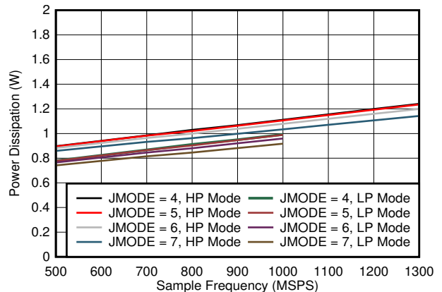
图 7-102. Single Channel, Power Dissipation vs FS for JMODES 4 - 7
