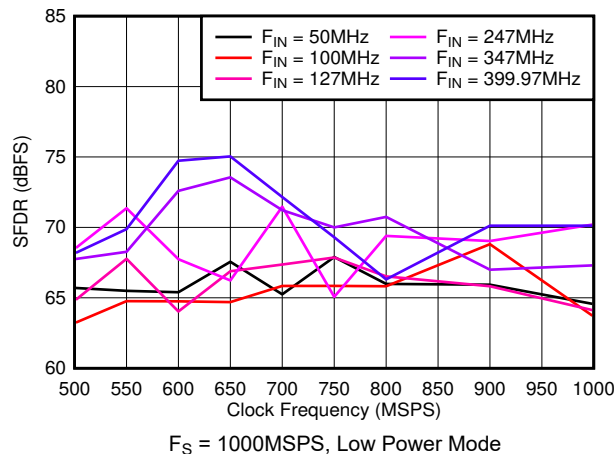
图 7-25. SFDR vs Sample Rate
