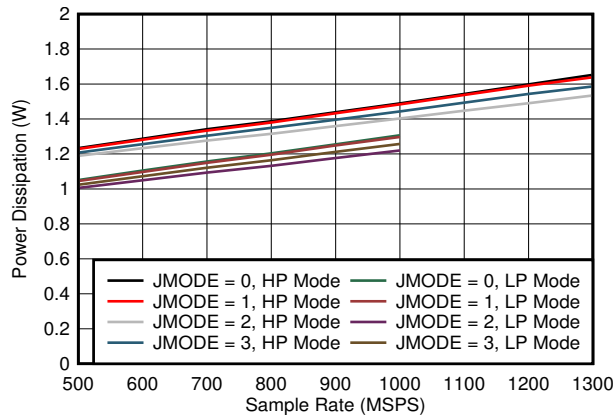
图 7-91. Dual Channel, Power Dissipation vs FS for JMODES 0 - 3
