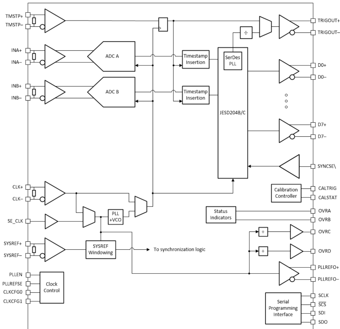
图 8-2. Dual Channel Functional Block Diagram
