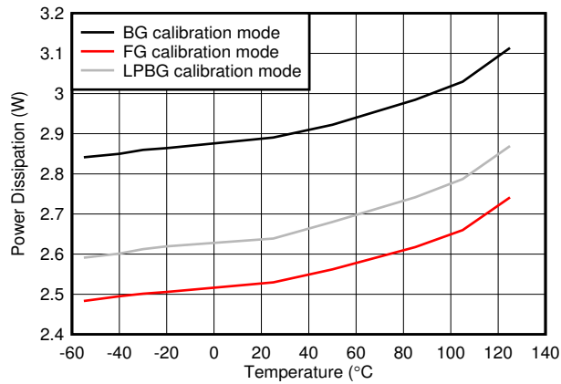
图 7-123. Quad Channel, Power Dissipation vs Temperature
