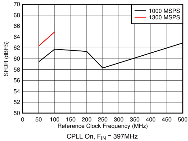
图 7-61. SFDR vs Reference Clock Frequency
