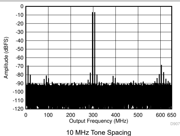
图 7-51. Two Tone FFT at 998 MHz Center
