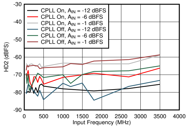
图 7-73. HD2 vs Input Frequency, CPLL and Input Amplitude
