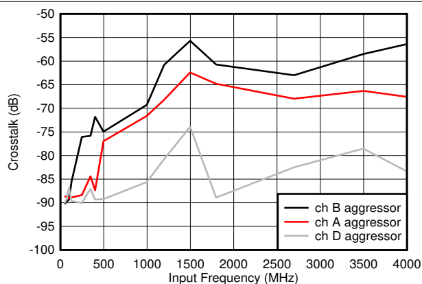
图 7-60. Crosstalk to Channel B vs F_{IN}
