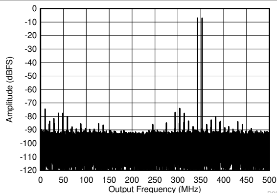
图 7-55. Two Tone FFT at 348 MHz Center
