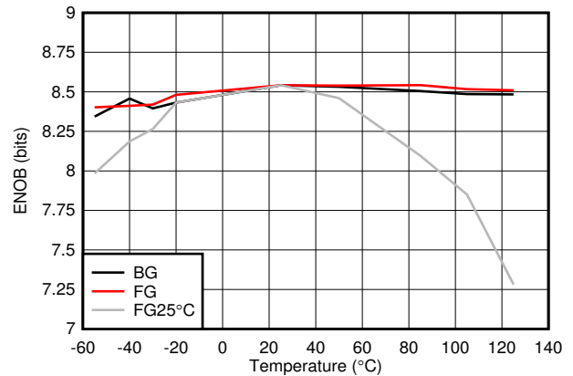
图 7-38. ENOB vs Temperature and Calibration Mode
