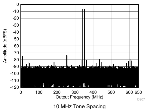
图 7-49. Two Tone FFT at 348 MHz Center
