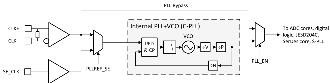
图 8-6. Converter PLL (C-PLL) Architecture
