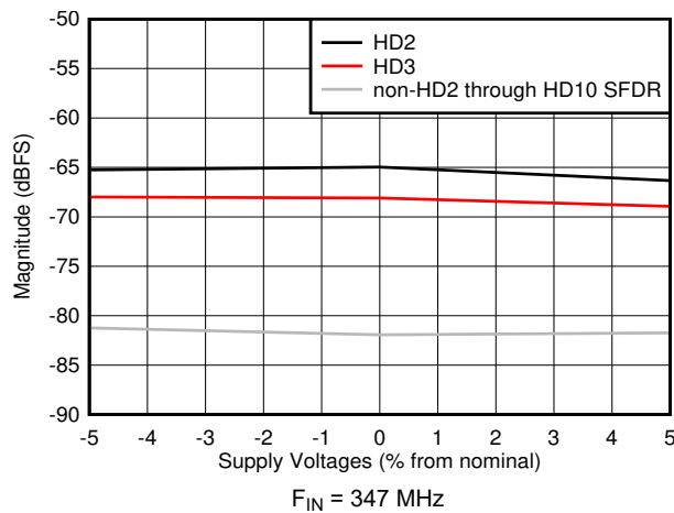
图 7-45. HD2, HD3 and Worst non-HD Spur vs Supply Voltage
