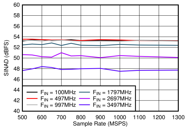
图 7-23. SINAD vs Sample Rate
