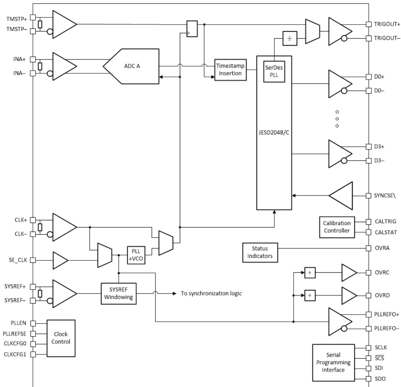
图 8-3. Single Channel Functional Block Diagram
