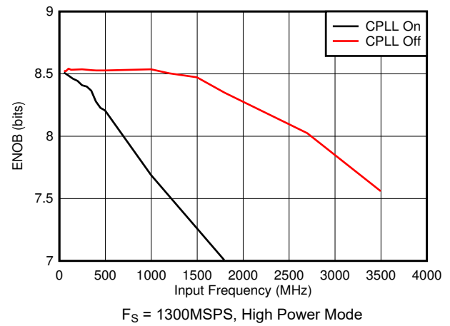
图 7-64. ENOB vs Input Frequency and CPLL
