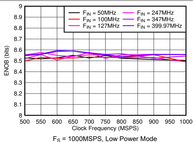
图 7-28. ENOB vs Sample Rate
