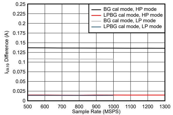
图 7-116. Single Channel, I_{VA19} Change with Calibration Mode
