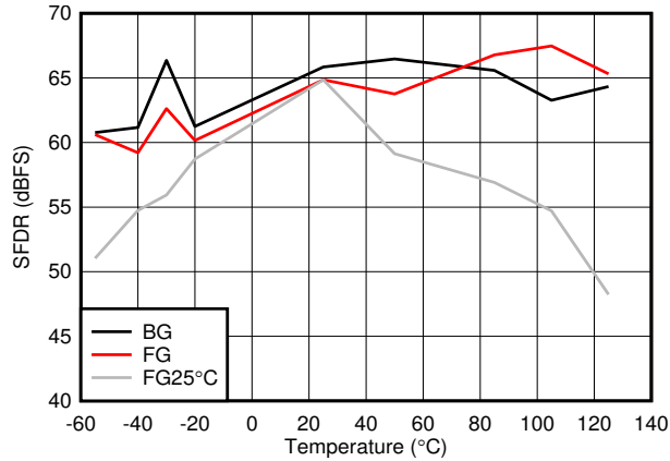
图 7-43. SFDR vs Temperature and Calibration Mode
