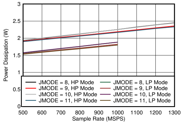
图 7-83. Quad Channel, Power Dissipation vs FS for JMODES 8 - 11
