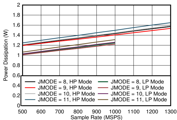
图 7-93. Dual Channel, Power Dissipation vs FS for JMODES 8 - 11
