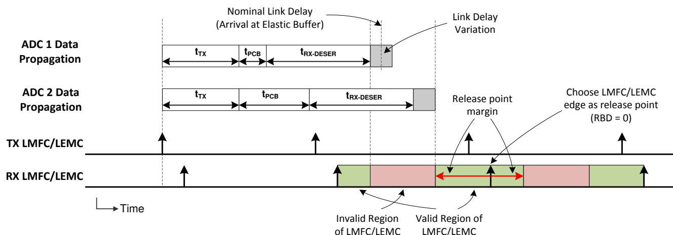
图 8-11. LMFC/LEMC Valid Region Definition for Elastic Buffer Release Point Selection
