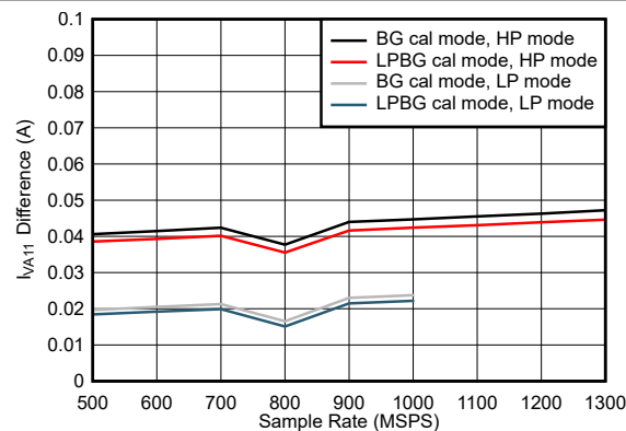
图 7-117. Quad Channel, I_{VA11} Change with Calibration Mode
