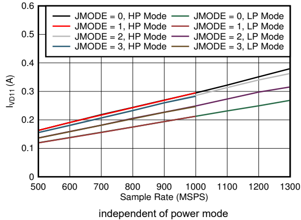
图 7-97. Dual Channel, I_{VD11} vs FS and JMODE 0 - 3
