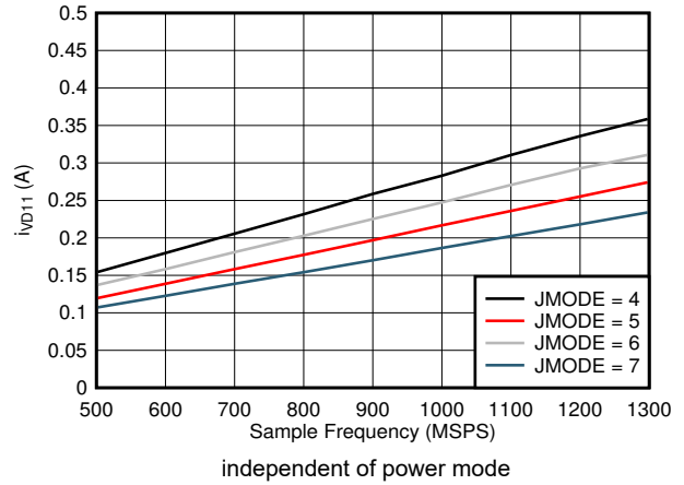
图 7-98. Dual Channel, I_{VD11} vs FS and JMODE 4 - 7
