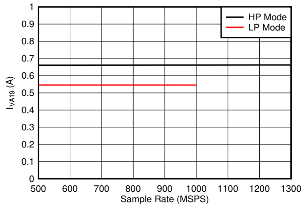
图 7-85. Quad Channel, I_{VA19} vs FS
