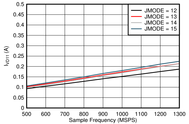
图 7-110. Single Channel, I_{VD11} vs FS and JMODE 12 - 15
