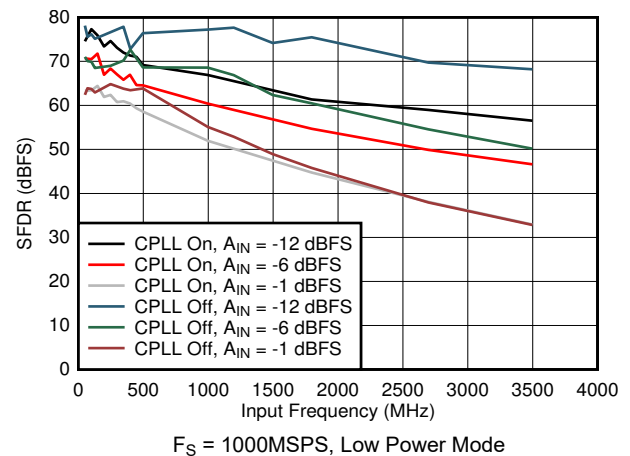
图 7-76. SFDR vs Input Frequency, CPLL and Input Amplitude
