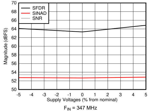
图 7-44. SNR, SFDR and SINAD vs Supply Voltage
