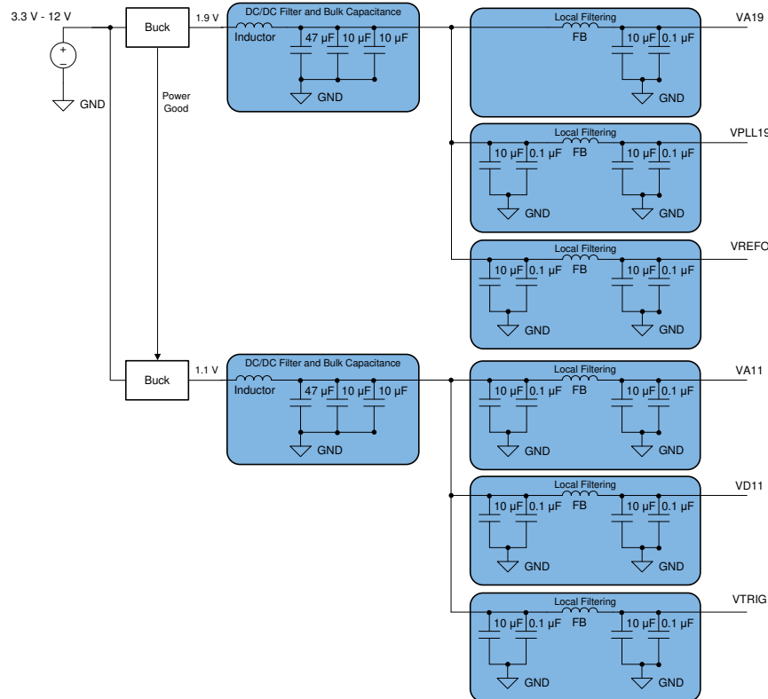
图 10-2. Switcher-Only Approach Example
