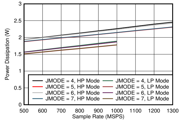
图 7-82. Quad Channel, Power Dissipation vs FS for JMODES 4 - 7
