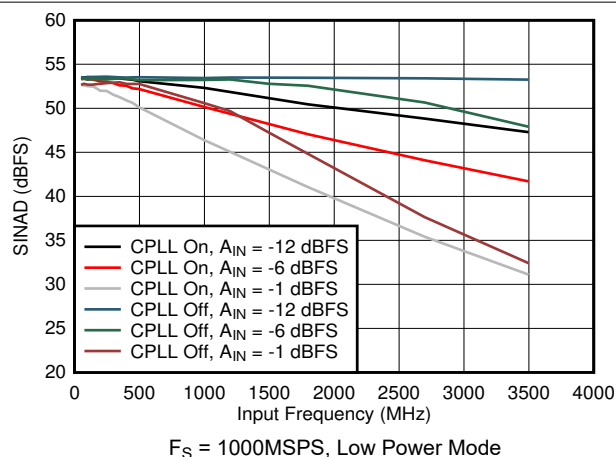
图 7-77. SINAD vs Input Frequency, CPLL and Input Amplitude
