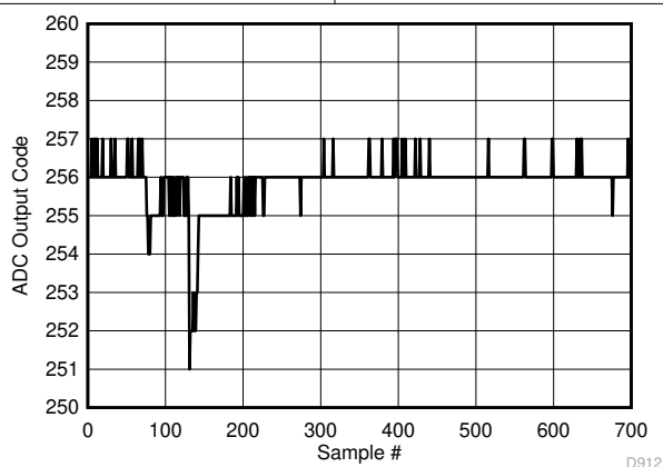
图 7-129. Background Calibration Core Transition (DC Signal)
