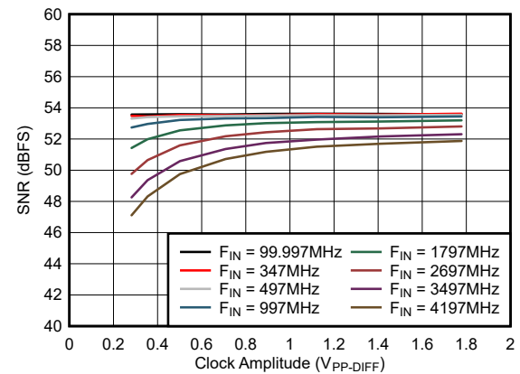
图 7-34. SNR vs Clock Amplitude
