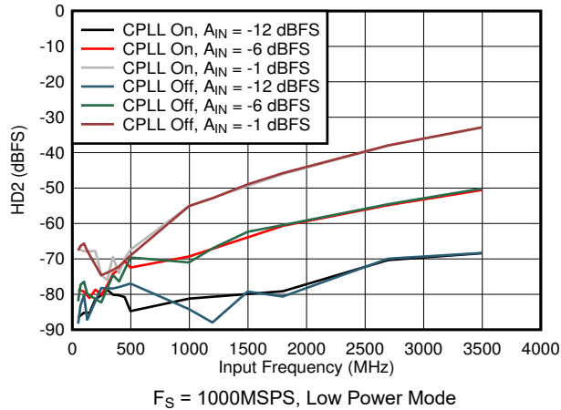
图 7-79. HD2 vs Input Frequency, CPLL and Input Amplitude
