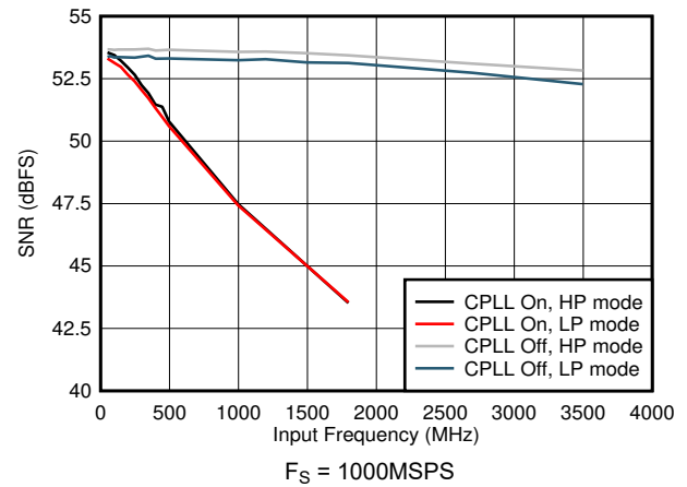
图 7-66. SNR vs Input Frequency and CPLL
