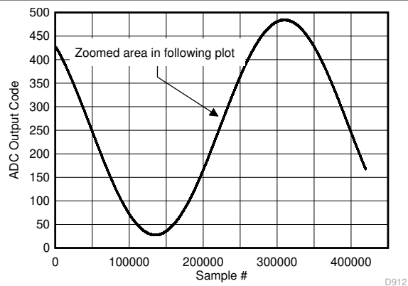
图 7-127. Background Calibration Core Transition (AC Signal)
