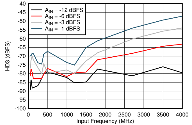
图 7-20. HD3 vs Input Frequency
