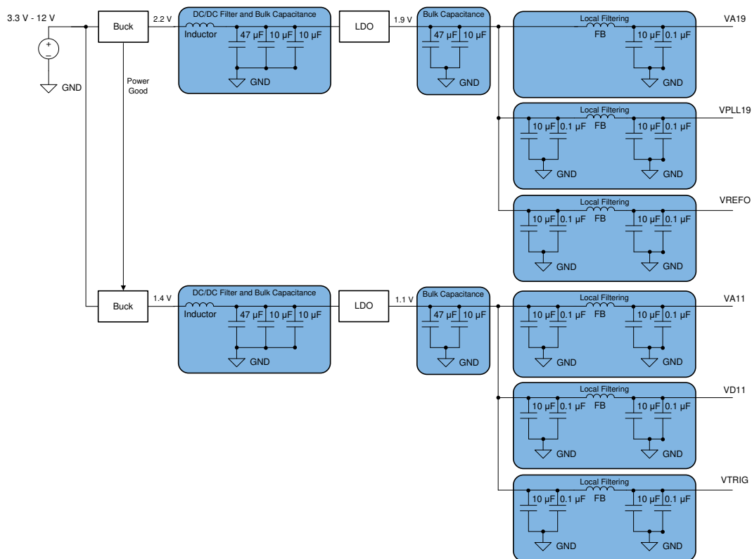
图 10-1. LDO Linear Regulator Approach Example
