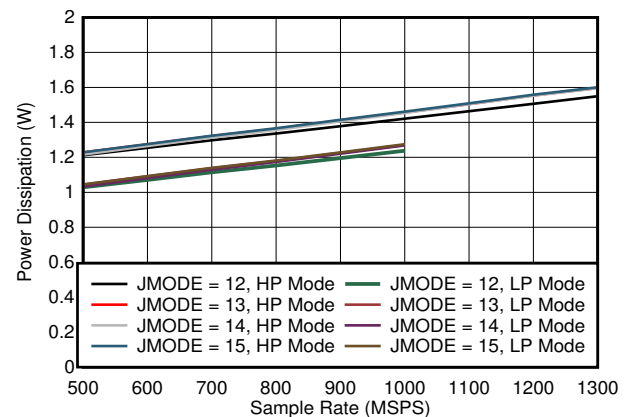
图 7-94. Dual Channel, Power Dissipation vs FS for JMODES 12 - 15
