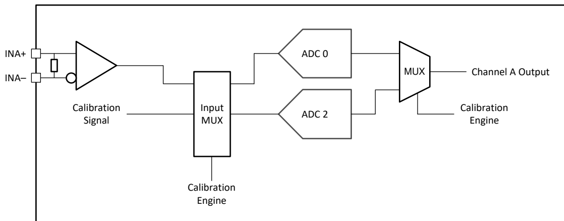
图 8-17. Single Channel Calibration System Block Diagram
