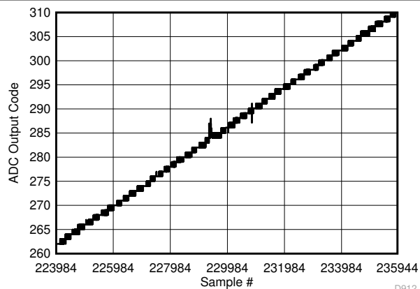
图 7-128. Background Calibration Core Transition (AC Signal Zoomed)
