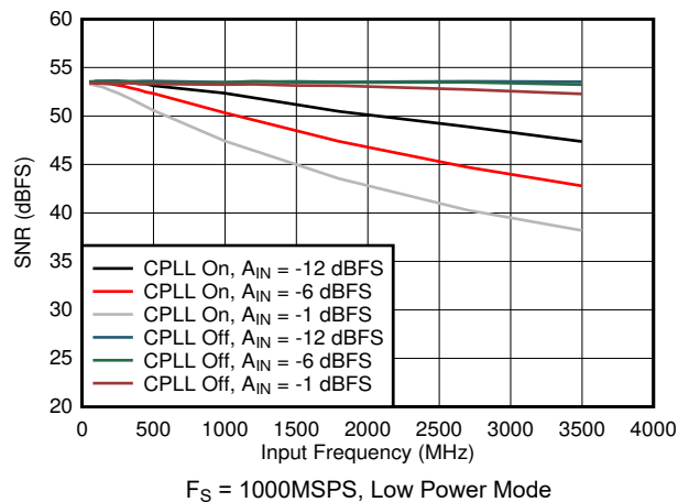
图 7-75. SNR vs Input Frequency, CPLL and Input Amplitude
