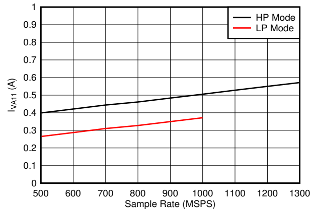
图 7-86. Quad Channel, I_{VA11} vs FS
