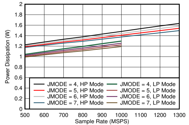
图 7-92. Dual Channel, Power Dissipation vs FS for JMODES 4 - 7
