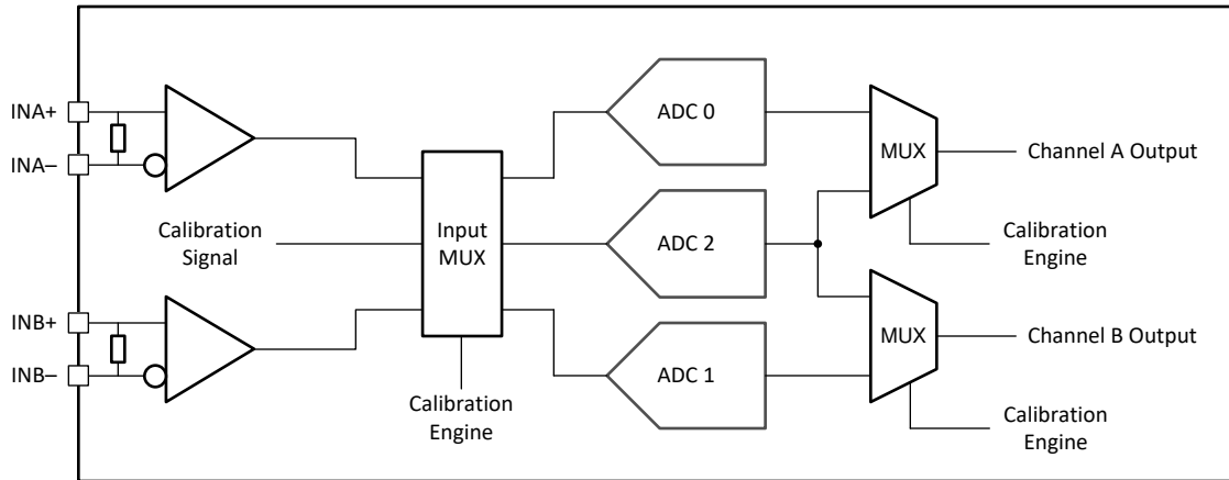
图 8-16. DualChannel Calibration System Block Diagram
