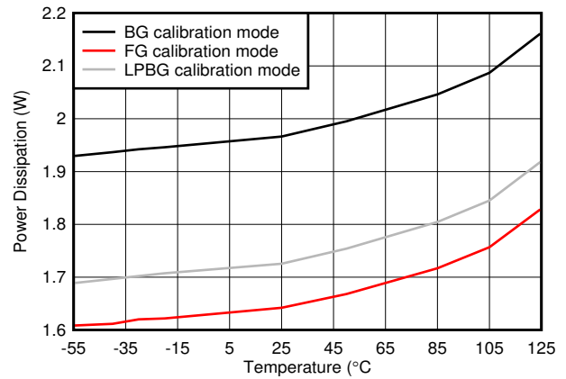
图 7-124. Dual Channel, Power Dissipation vs Temperature
