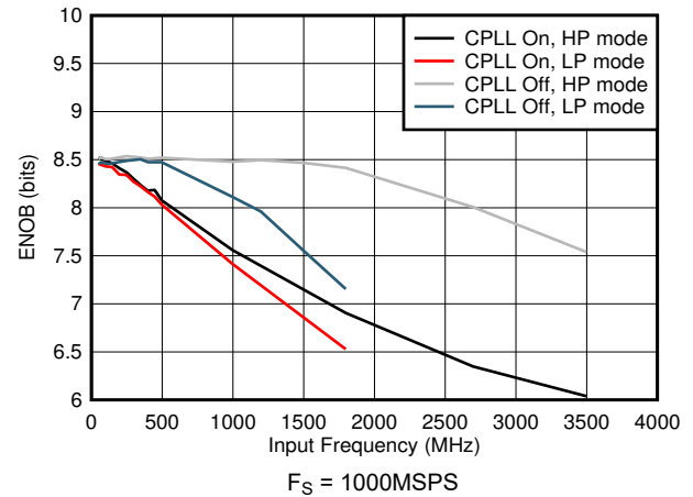
图 7-68. ENOB vs Input Frequency and CPLL
