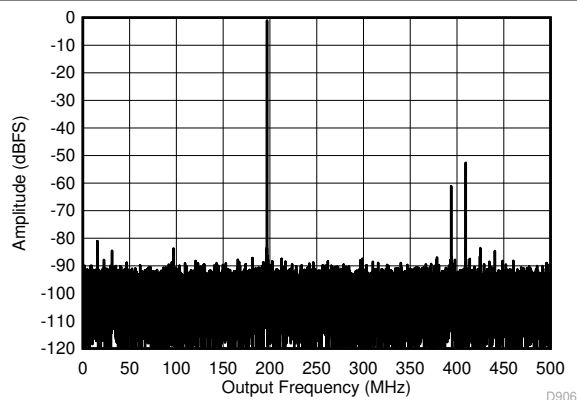
图 7-13. Single Tone FFT at 1197 MHz and -1 dBFS
