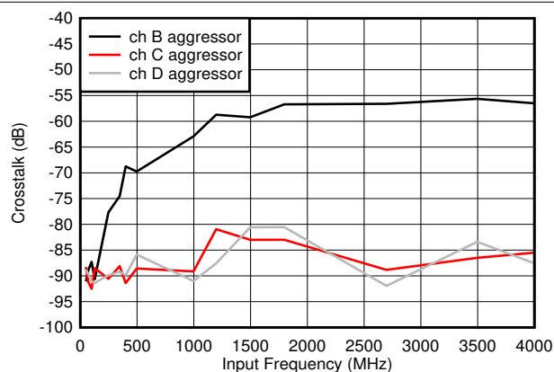
图 7-59. Crosstalk to Channel A vs F_{IN}
