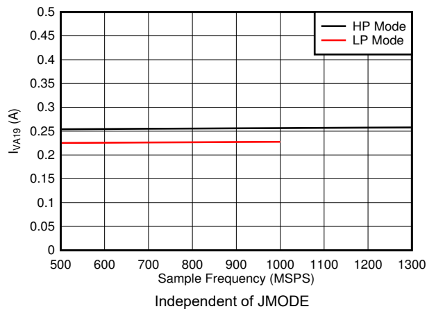
图 7-105. Single Channel, I_{VA19} vs FS
