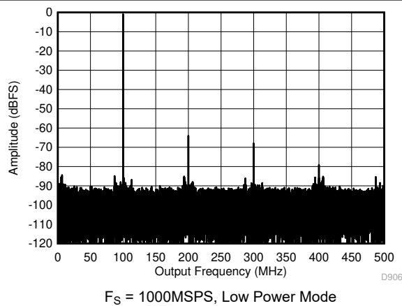
图 7-11. Single Tone FFT at 99.997 MHz and -1 dBFS
