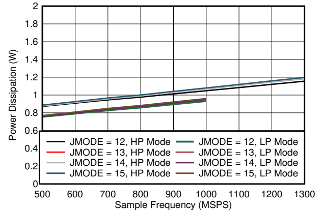
图 7-104. Single Channel, Power Dissipation vs FS for JMODES 12 - 15
