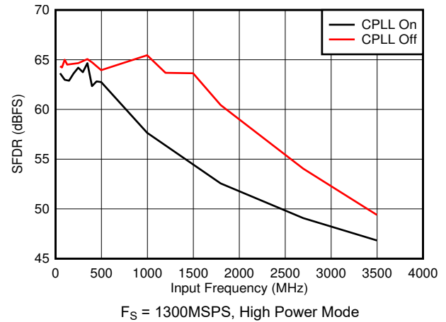
图 7-62. SFDR vs Input Frequency and CPLL
