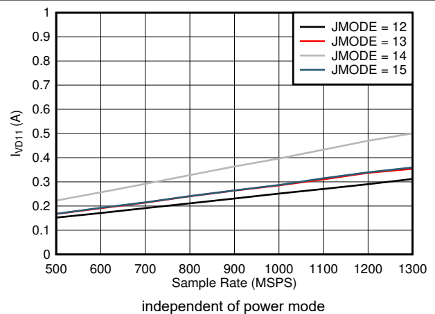
图 7-90. Quad Channel, I_{VD11} vs FS and JMODE 12 - 15
