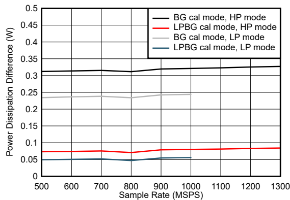
图 7-111. Quad Channel, Power Dissipation Change with Calibration Mode
