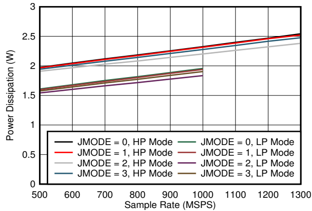
图 7-81. Quad Channel, Power Dissipation vs FS for JMODES 0 - 3
