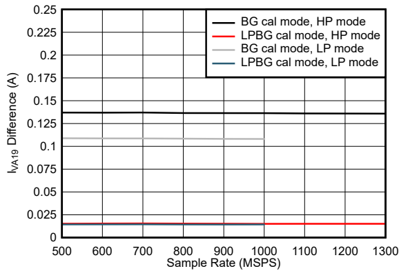
图 7-115. Dual Channel, I_{VA19} Change with Calibration Mode
