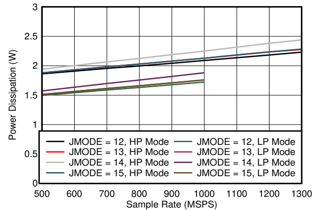
图 7-84. Quad Channel, Power Dissipation vs FS for JMODES 12 - 15
