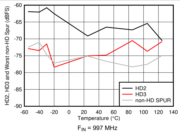
图 7-36. HD2, HD3 and worst non-HD Spur vs Temperature
