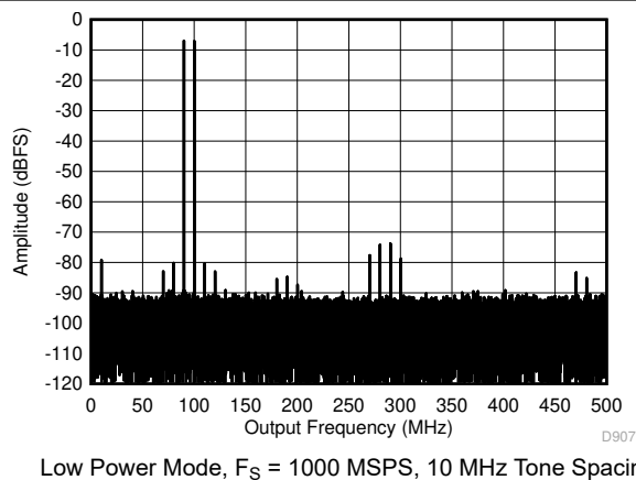
图 7-54. Two Tone FFT at 95.07 MHz Center
