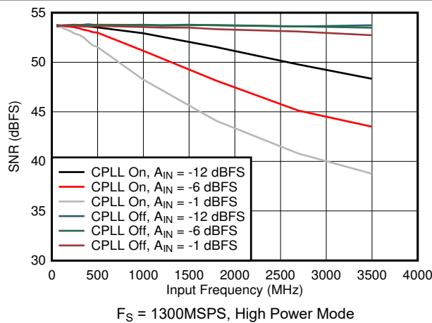
图 7-69. SNR vs Input Frequency, CPLL and Input Amplitude
