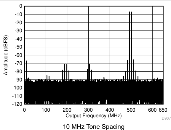
图 7-52. Two Tone FFT at 1798 MHz Center
