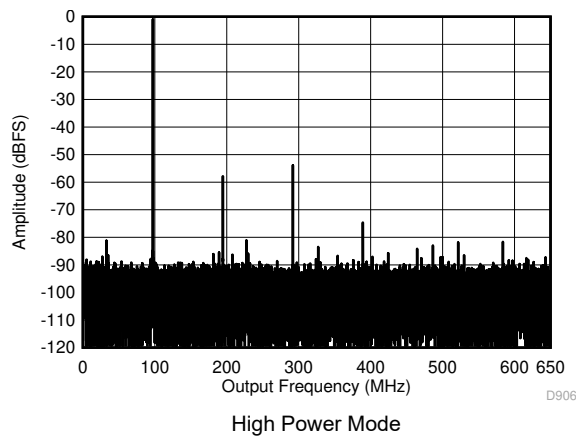
图 7-9. Single Tone FFT at 2697 MHz and -1 dBFS
