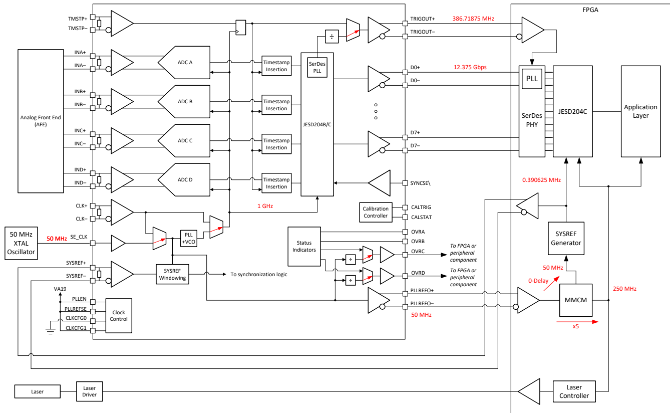
图 9-1. Typical Configuration for a LiDAR Digitizer
