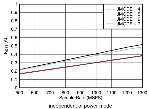
图 7-88. Quad Channel, I_{VD11} vs FS and JMODE 4 - 7
