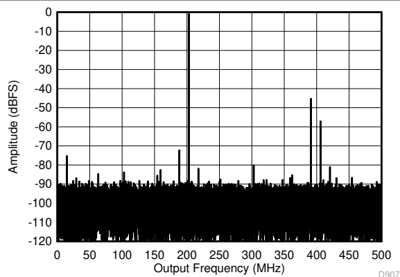
图 7-14. Single Tone FFT at 1797 MHz and -1 dBFS
