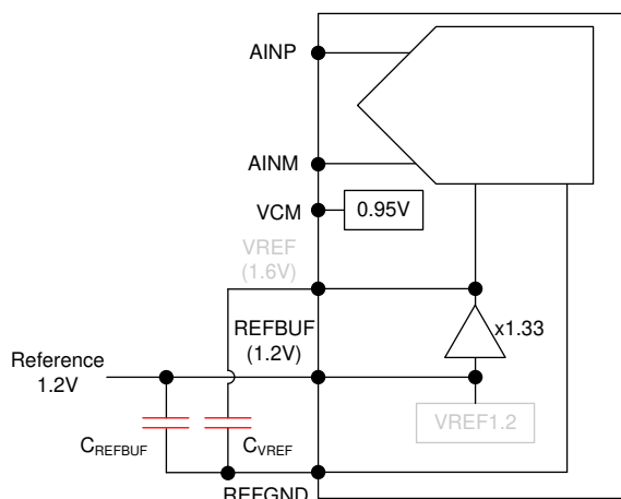
图 8-18. External 1.2V reference using internal reference buffer
