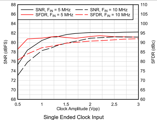
图 6-16. AC Performance vs Clock Amplitude
