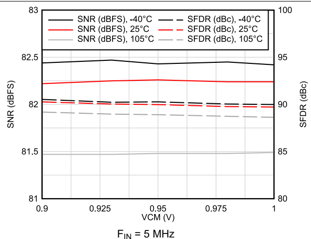
图 6-18. AC Performance vs VCM vs Temperature
